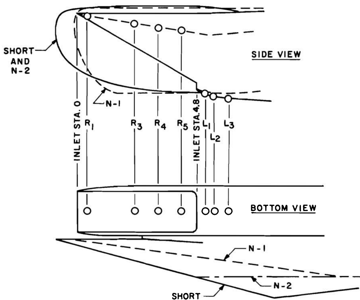
Fig. 10 Inlet Model Configurations and Pressure Orifice Locations
