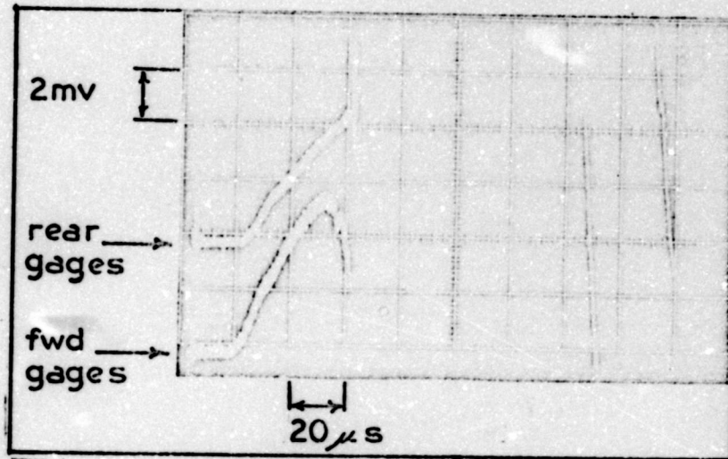
Fig. 26. Shot #30, Strain Pulse Distortion Experiment: Oscilloscope Traces
