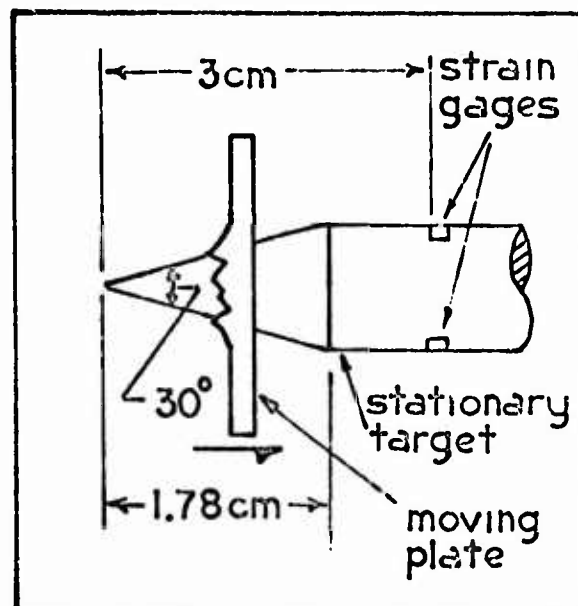
Fig. 13. The 30° Cone Perforation Model (Not to scale)
