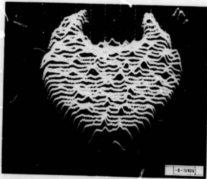
Fig. 4. Response profile of an \text{In}_{0.17}\text{Ga}_{0.83}\text{As} avalanche photodiode operating at a gain of 100 when scanned with a HeNe 0.633- \mu\text{m} laser.
