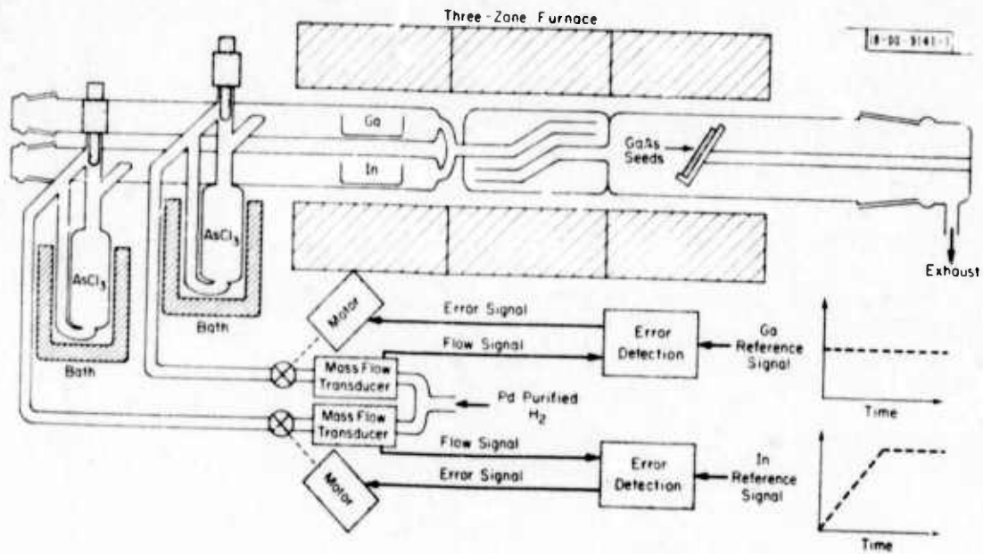
Fig. 1. Schematic diagram of the epitaxial \text{In}_x\text{Ga}_{1-x}\text{As} growth system.
