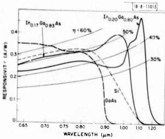
Fig. 3. Spectral responsivity of two \text{In}_x\text{Ga}_{1-x}\text{As} avalanche photodiodes at unity gain.
