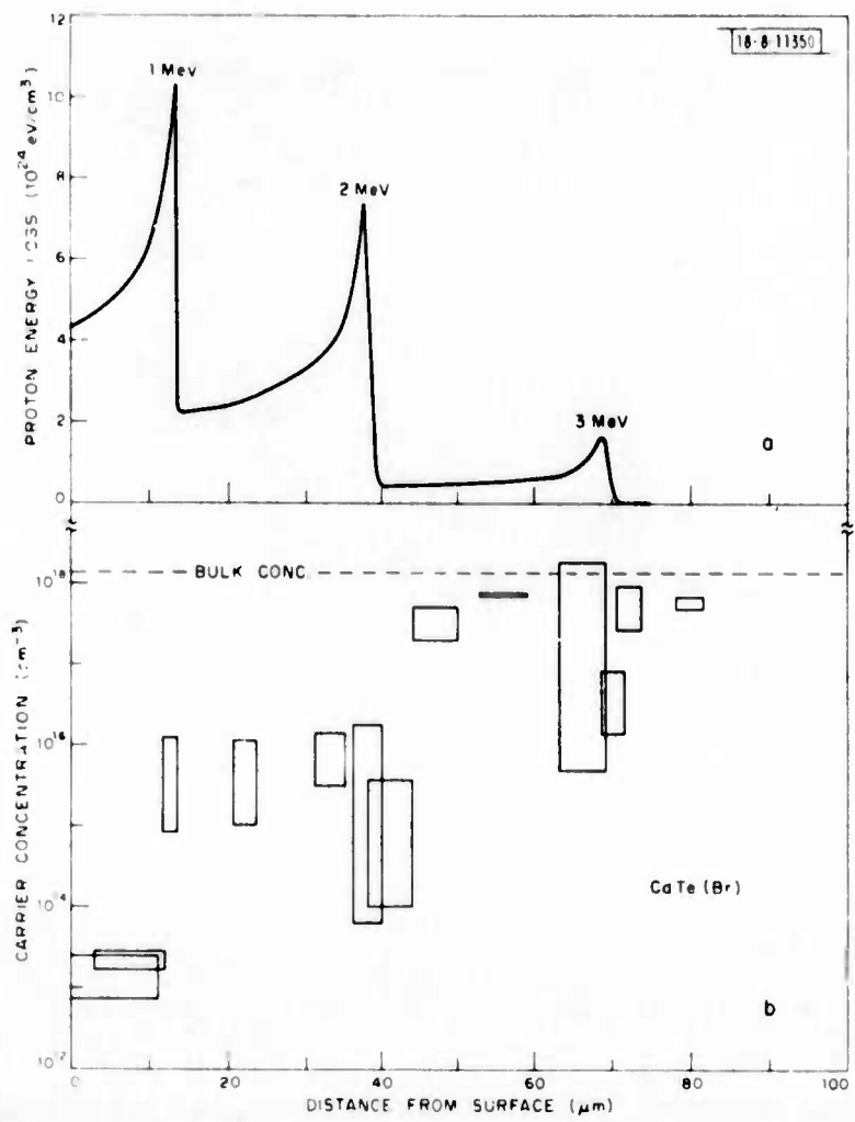
Fig. 7. (a) Theoretical proton energy loss as a function of distance from the surface for a CdTe sample subjected to three successive bombardments:
