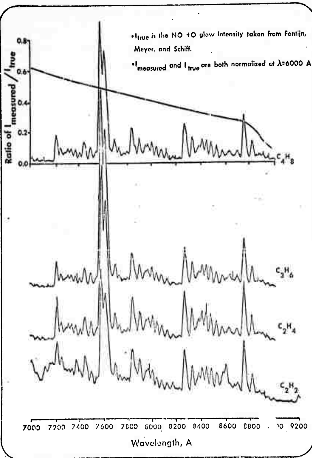
Figure 8. Meinel bands of OH for the attack of O on C_2H_4 at short contact time ( \sim 1-3 \text{ m sec} ) taken from Krieger, Malki and Kummler (1972). The total pressure is 1.28 Torr and the hydrocarbon partial pressure is 20 millitorr.
