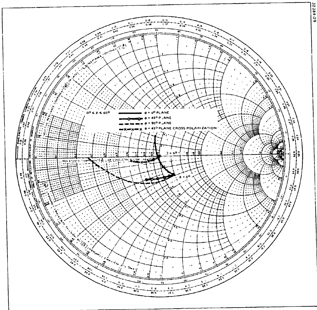
Figure 4-3(b). Impedance Loci at f_h for a Horizontally Polarized Array
