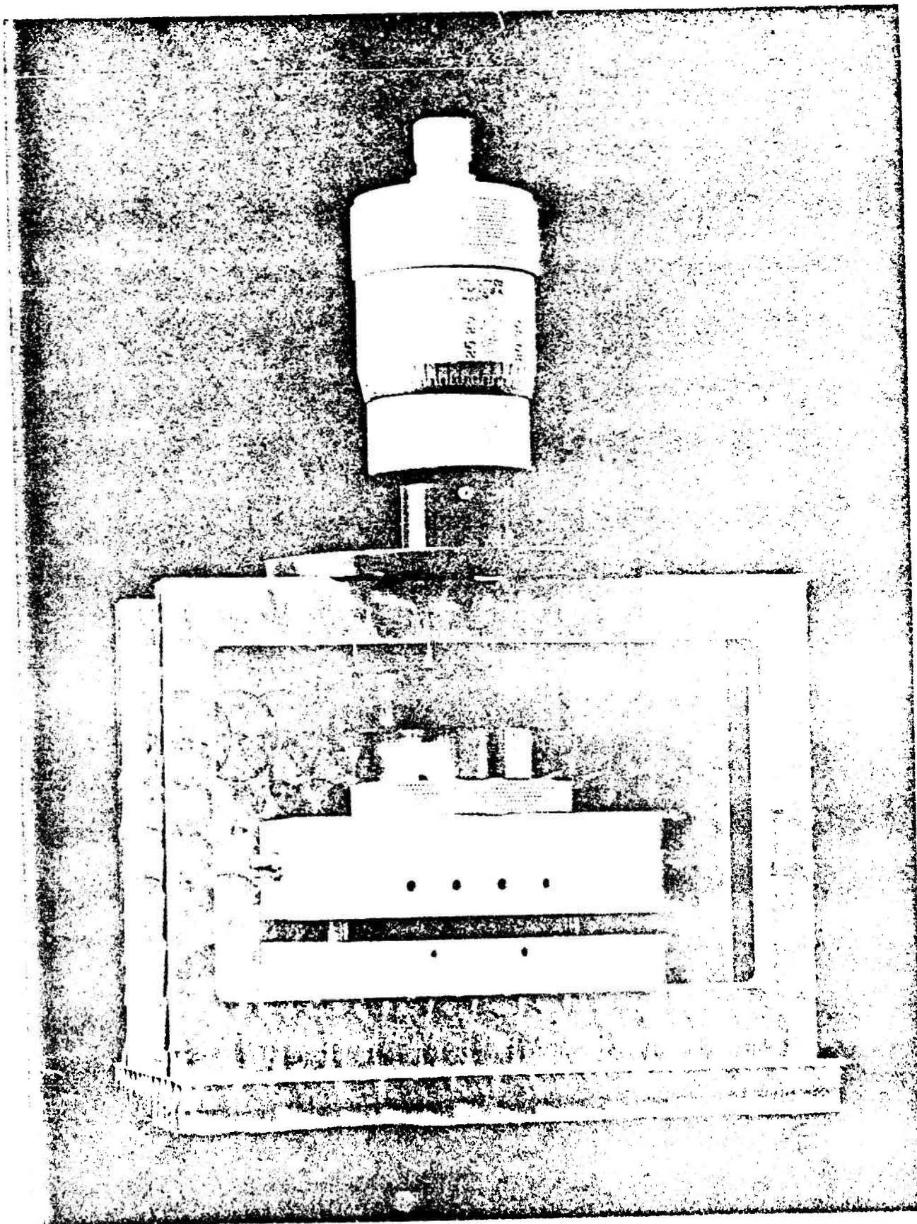
Figure 1a. Fluid coupling device showing the translating transducer mount (upper) and the stationary sample mount (lower)
