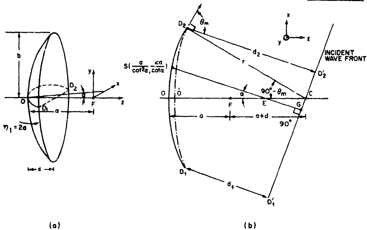
Fig. 1. Cross sectional view of a paraboloidal reflector.
