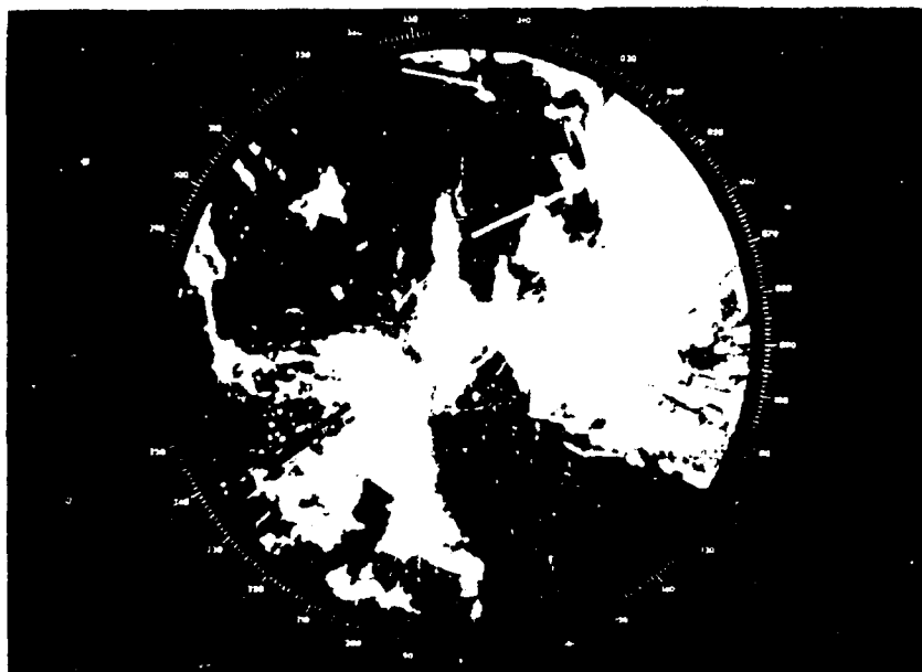
FIGURE 4-35. PPI display of VTS radar with linear antenna polarization during a rainstorm.
