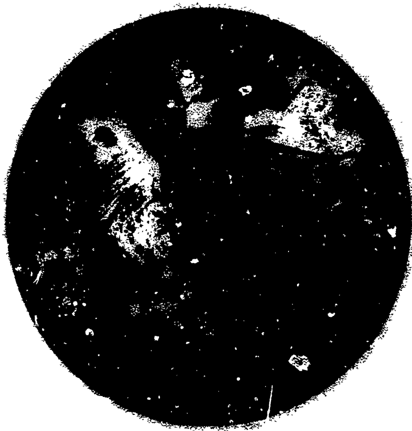
FIGURE 4-25. PPI display of AIL radar without FTC tracking 40-foot cutter at 190 degrees, range of 2300 yards in a local rainstorm.
