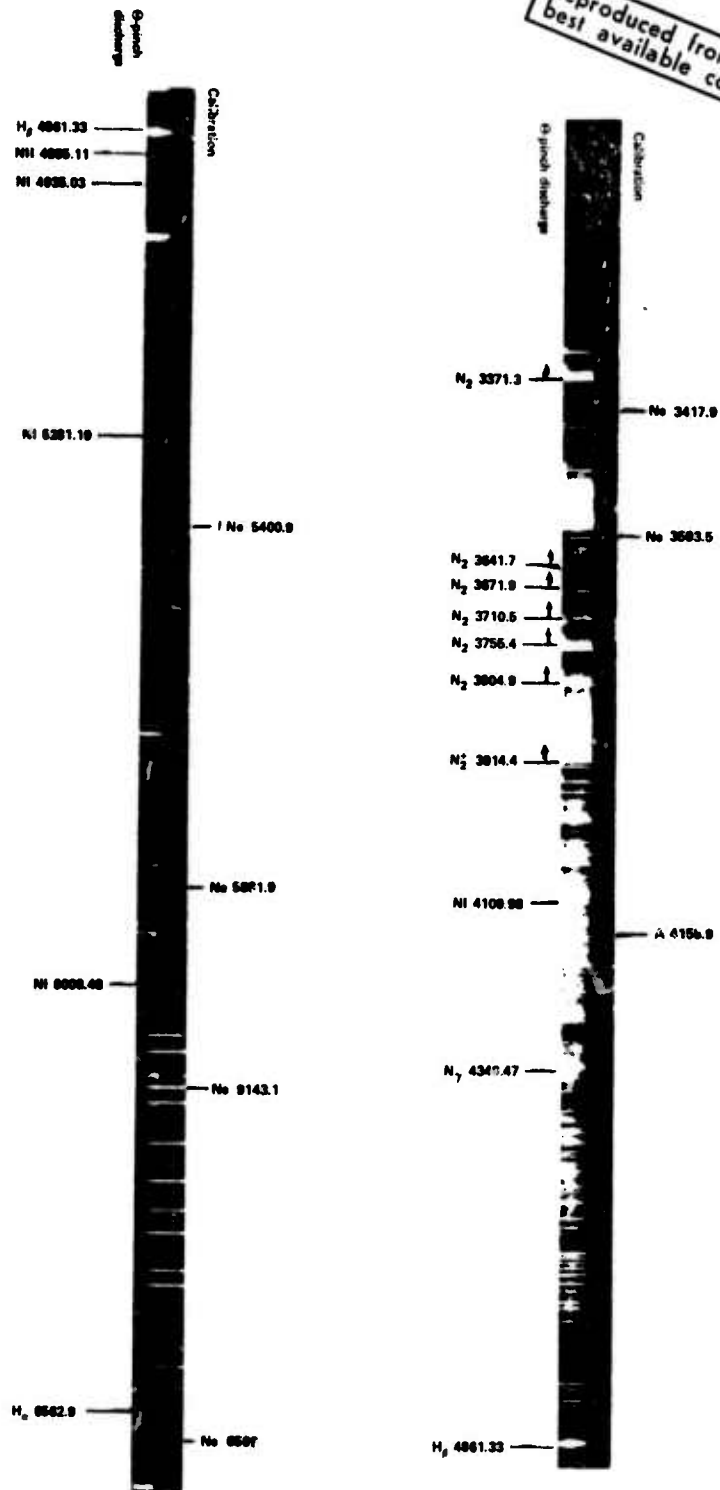
Figure 4. Spectrum of emission by the \theta -pinch device when filled to a pressure of 10 \mu with gaseous nitrogen.
