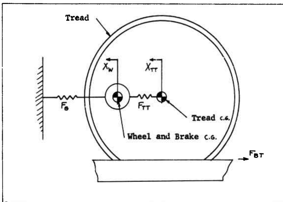
Figure A34 Tire Horizontal Model
