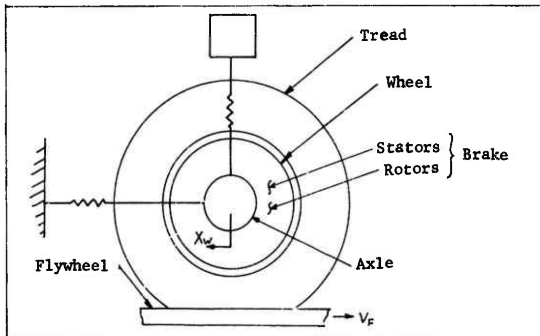
Figure A33 Components of the Wheel and Tire System
