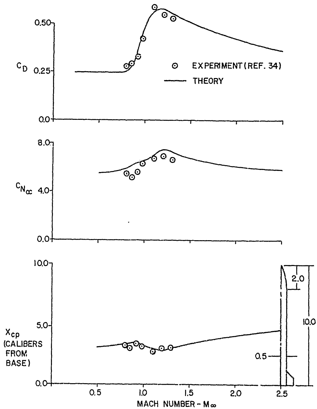
FIGURE 29. STATIC AERODYNAMICS OF A MISSILE CONFIGURATION; R=1.0 , \Delta_1=53.1^\circ , \lambda=0.5 , \alpha=1^\circ
