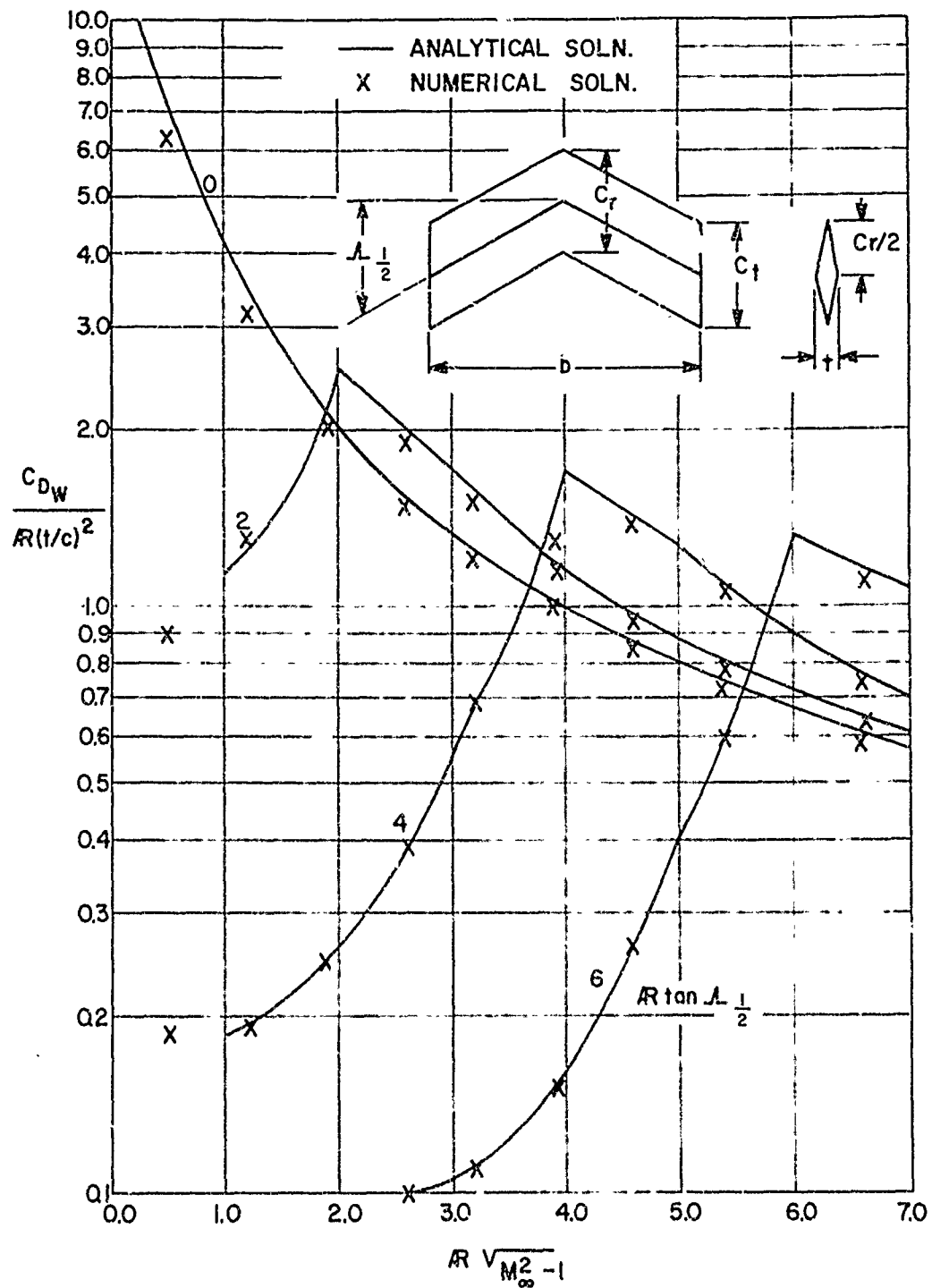
FIGURE 22. WAVE DRAG OF WING WITH DOUBLE WEDGE AIRFOIL SECTION; C_t / C_r = 1.0
