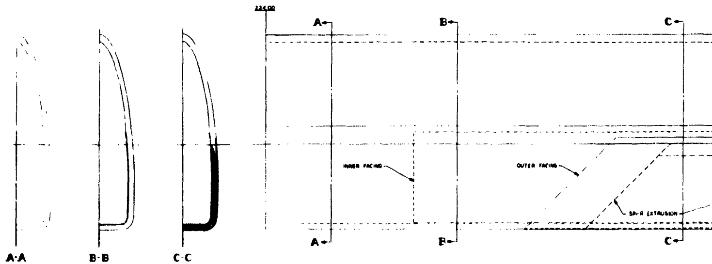
SPAR ASSEMBLY
