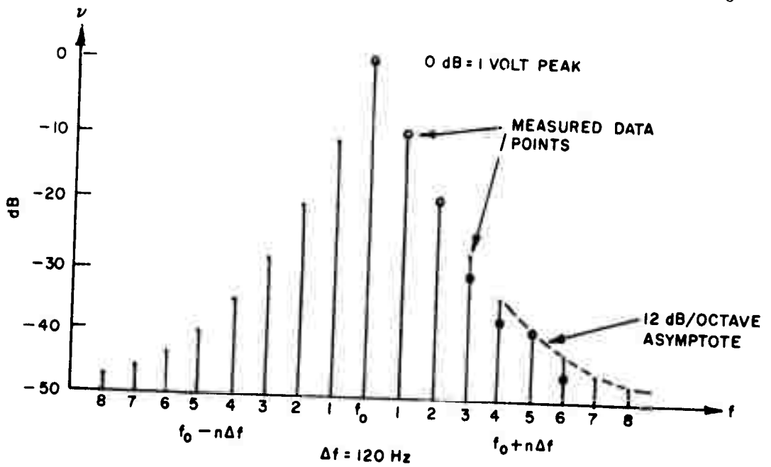
Figure 3-1B. Spectrum of Single-Phase, Full-Wave Dielectric Heater Signal
