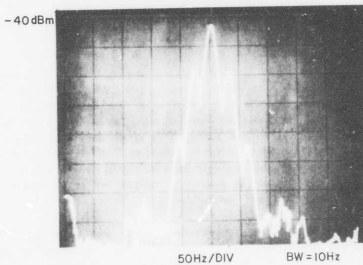
Figure B-6. VOR Carrier (SG-13 Simulator)
