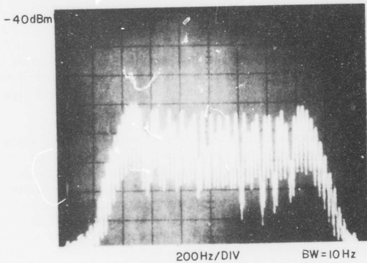
Figure B-5. VOR 9960 Hz Subcarrier (SG-13 Simulator)
