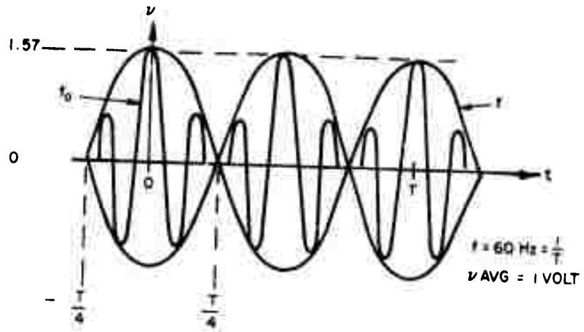
Figure 3-1A. Time Waveform of a Single-Phase, Full-Wave Dielectric Heater Signal
