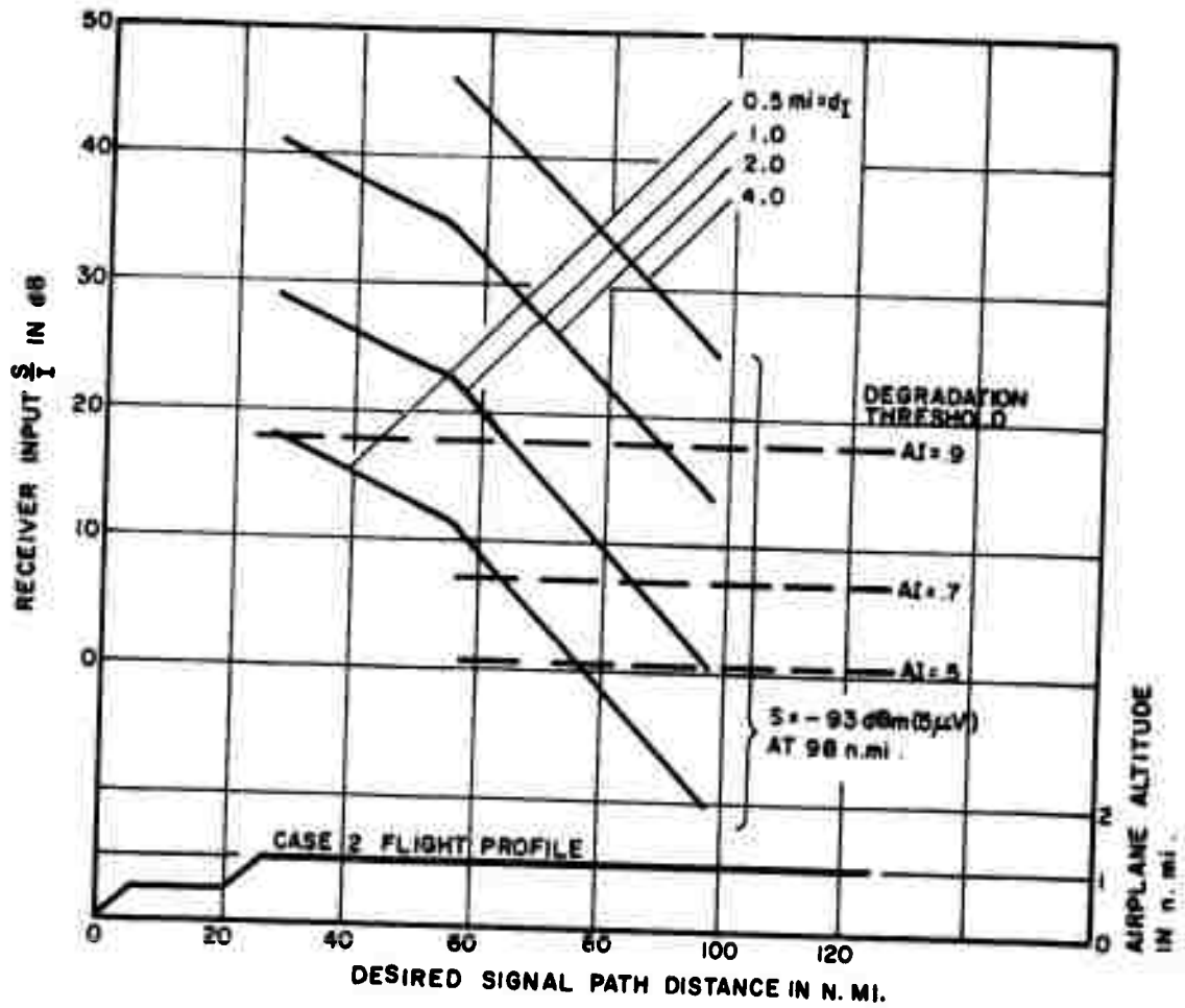
Figure 4-4. Communication Receiver Input Signal-to-Interference Ratios at Various Aircraft Locations for a Family of Interfering Path Distances with a Dielectric Heater Radiating 10 \mu V/m at 5280 feet
