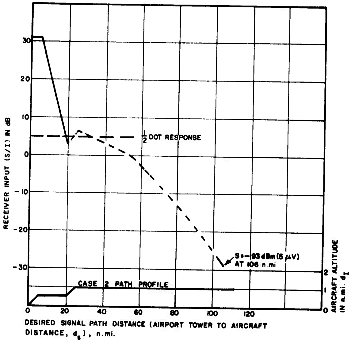
Figure 4-7. ILS Localizer Receiver Input Signal-to-Interference Ratio at Various Aircraft Locations for a Dielectric Heater Radiation of 10 μV/meter at 5280 feet
