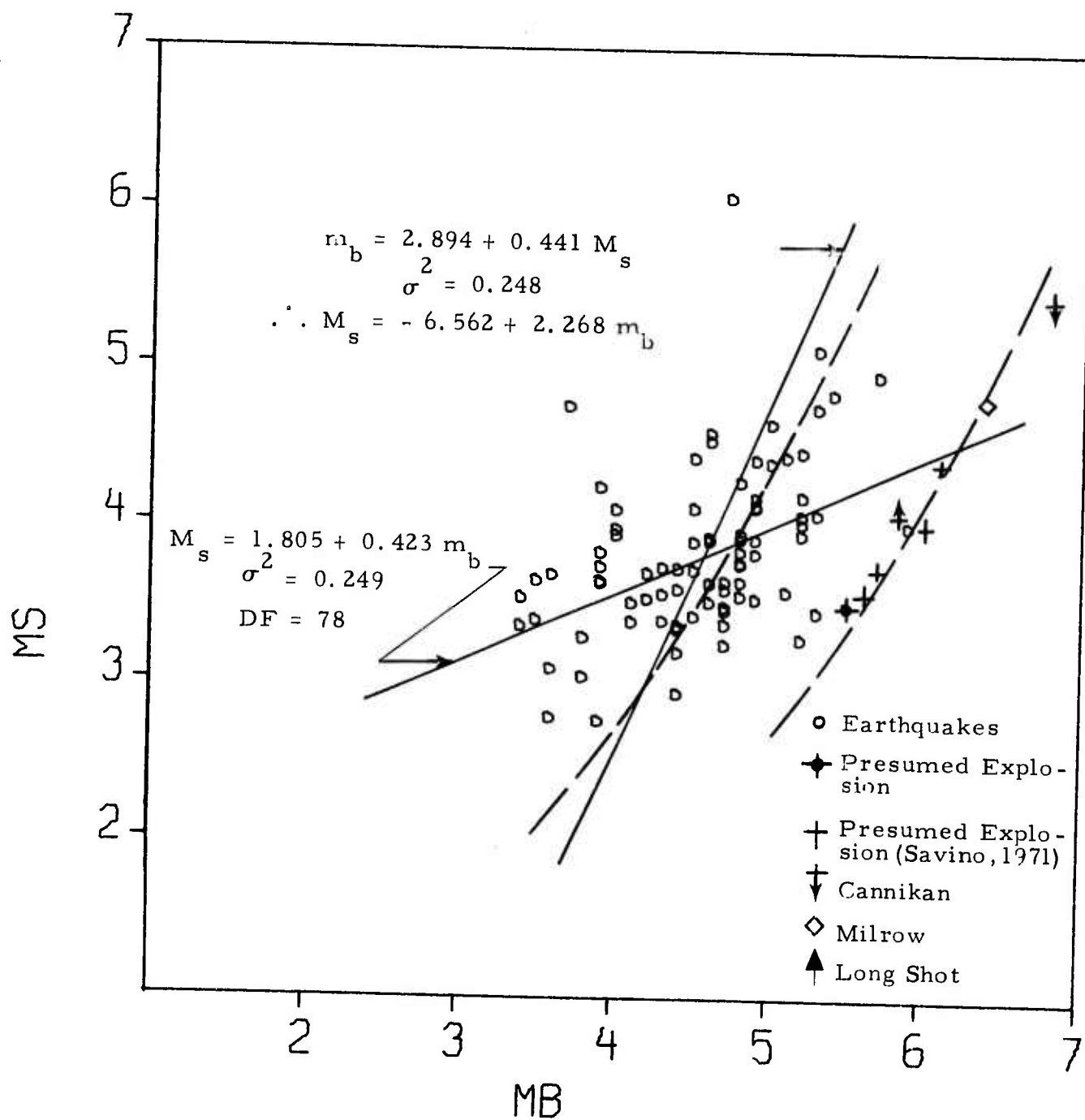
FIGURE III-32 M_s VERSUS m_b FOR 1/1/72 - 3/20/72 ( M_s DETERMINED BY TWO OR MORE VLPE STATION ESTIMATES)
