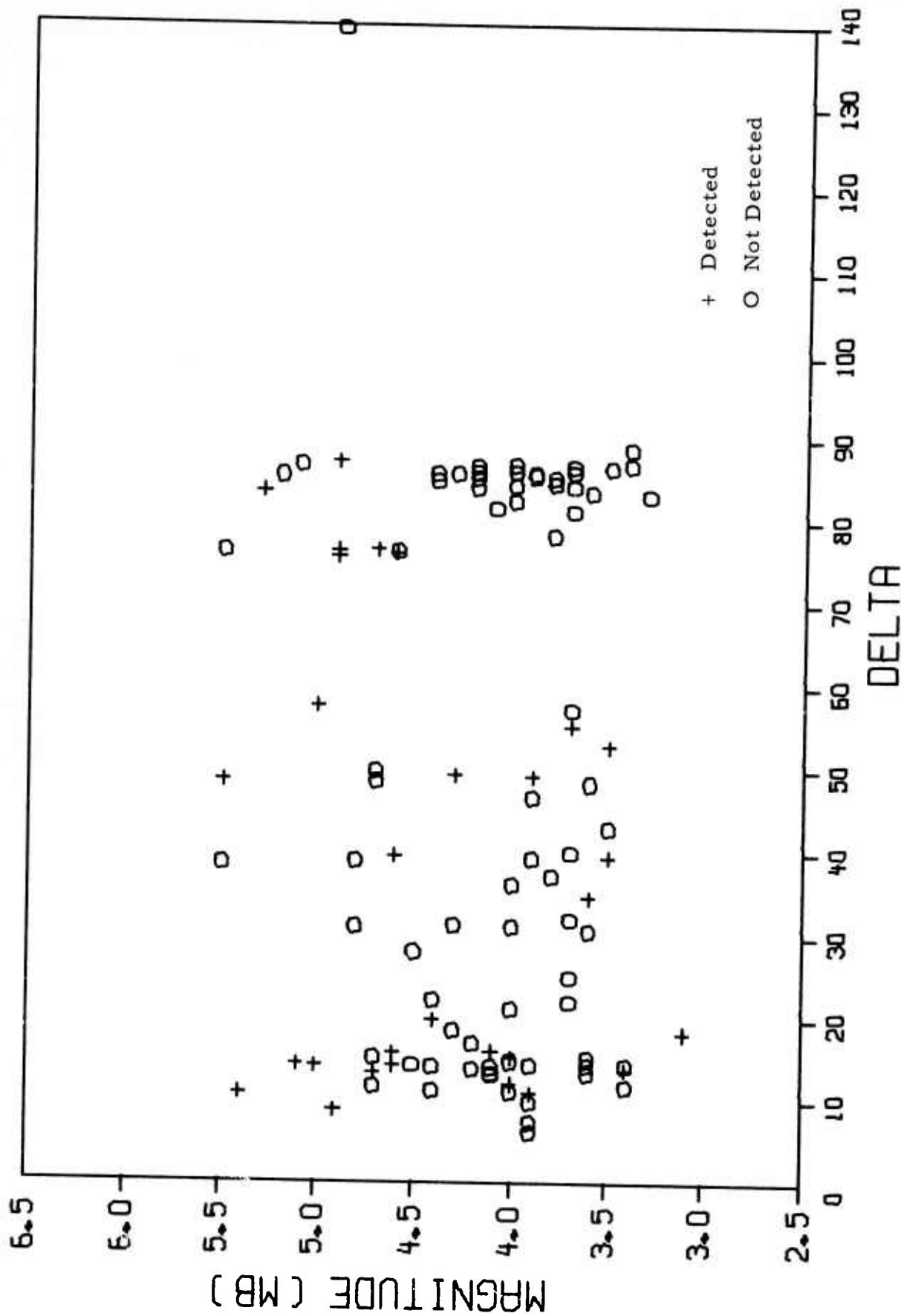
FIGURE III-9 EVENT DETECTION AS A FUNCTION OF DISTANCE AND MAGNITUDE ( m_b ) AT EIL, 6/1/72 - 7/31/72
