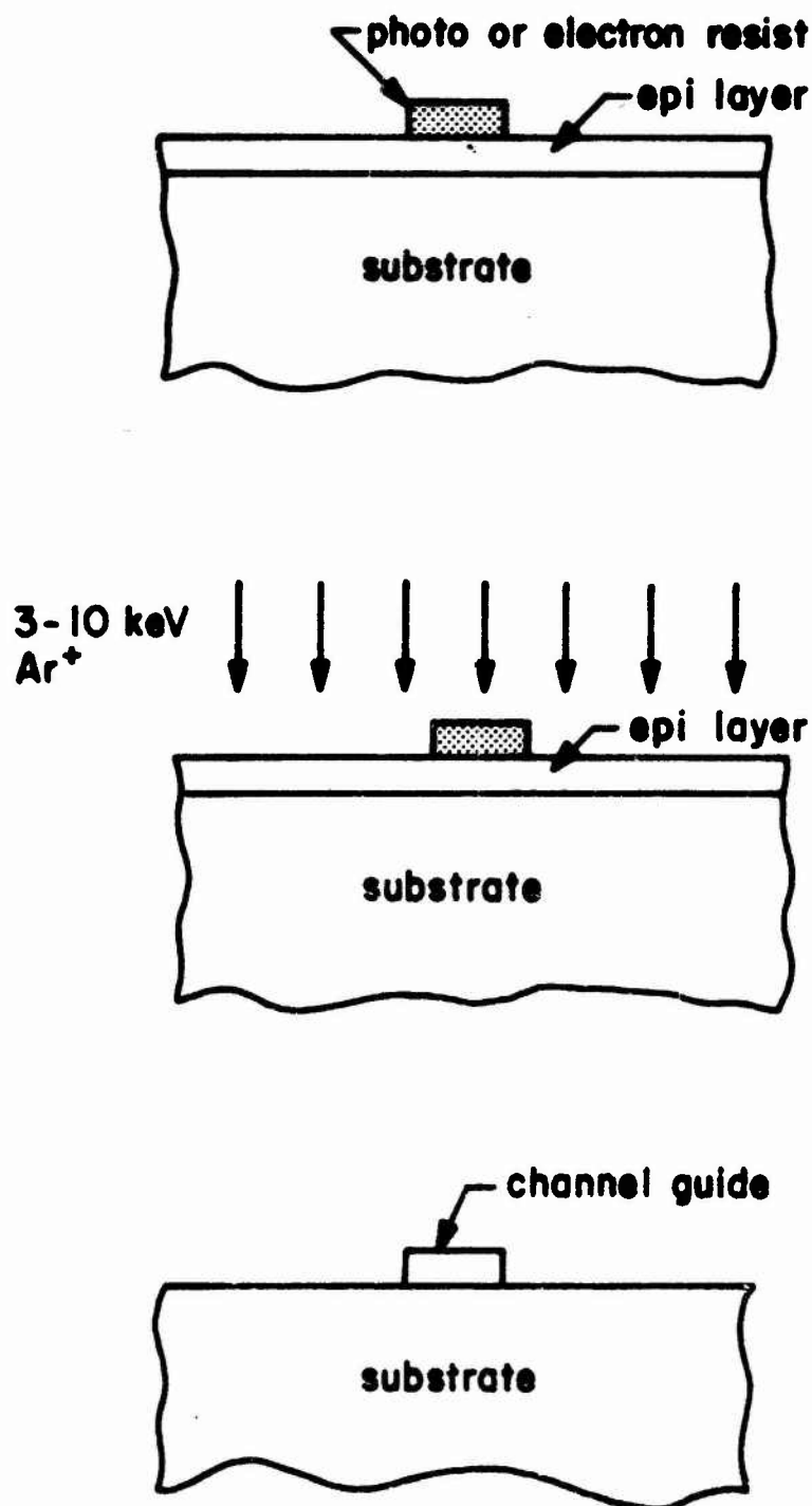
Fig. IV.8 Channel waveguide fabrication by removal of superfluous sections of an epilayer by ion milling.
