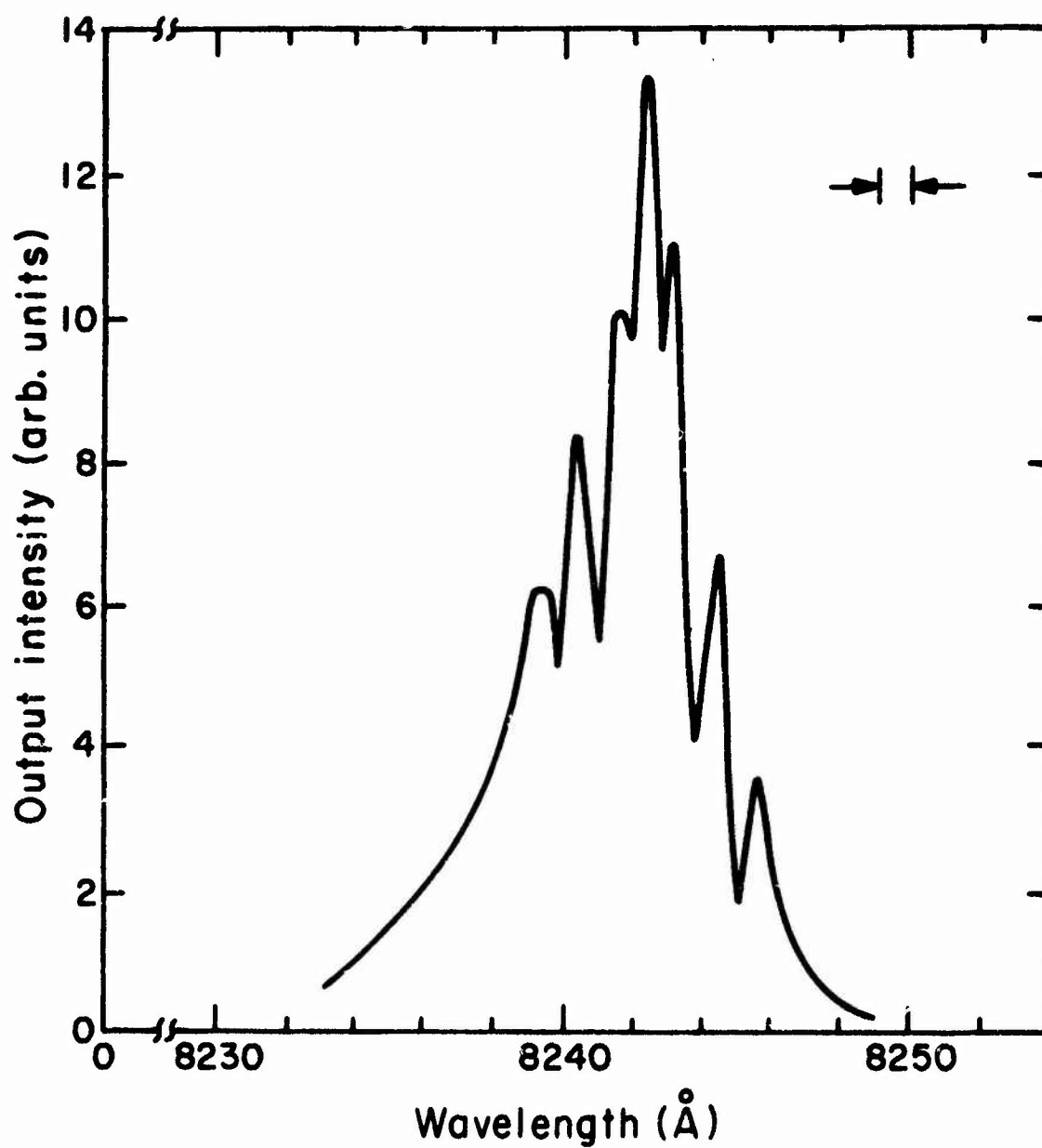
Fig. III.10. The emission spectrum of laser oscillation. The length of the pumped region was 700\mu . I/I_{th} = 1.4
