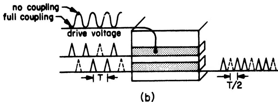
Fig. II.19 (a) Multiplexing scheme for a higher rate of information modulation. (b) Directional coupler multiplexer.
