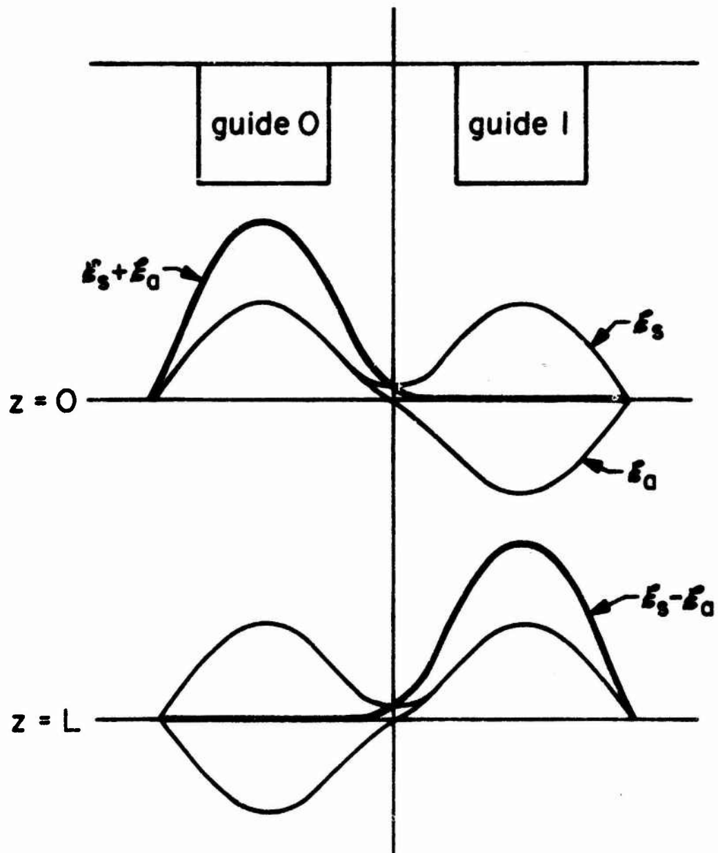
Fig. II.7 The symmetric and antisymmetric eigen modes of a dual directional coupler. Power is transferred from one channel to another because of not identical propagation constants.
