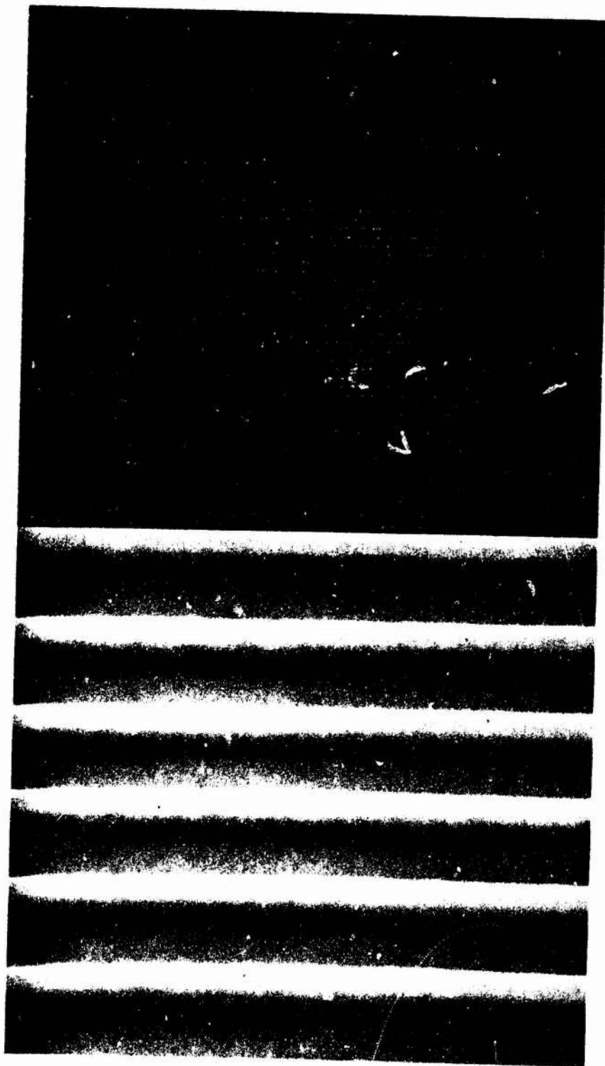
Fig. IV.4 SEM photographs of 1.4\text{ }\mu\text{m} grating in GaAs.
