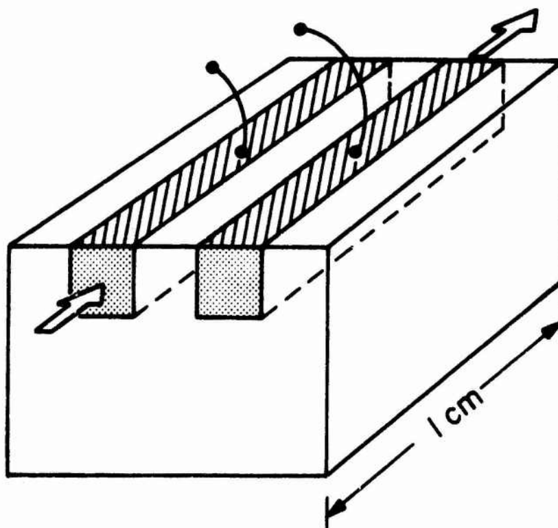
Fig. II.17 Example of a directional coupler modulator.
