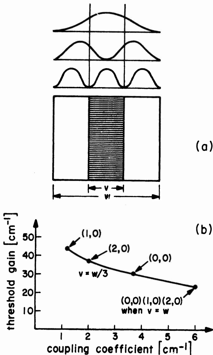
Fig. III.13. (a) Power profile distribution for different width-transverse modes.
