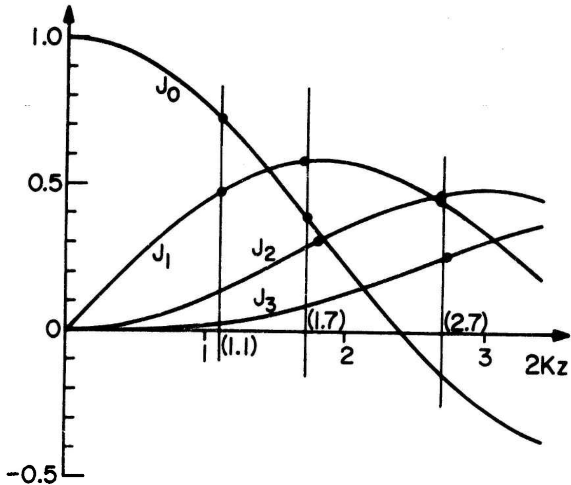
Fig. II.10 Sketch of various orders Bessel functions to which the square root of the amplitudes in Fig. II.1 are fitted.
