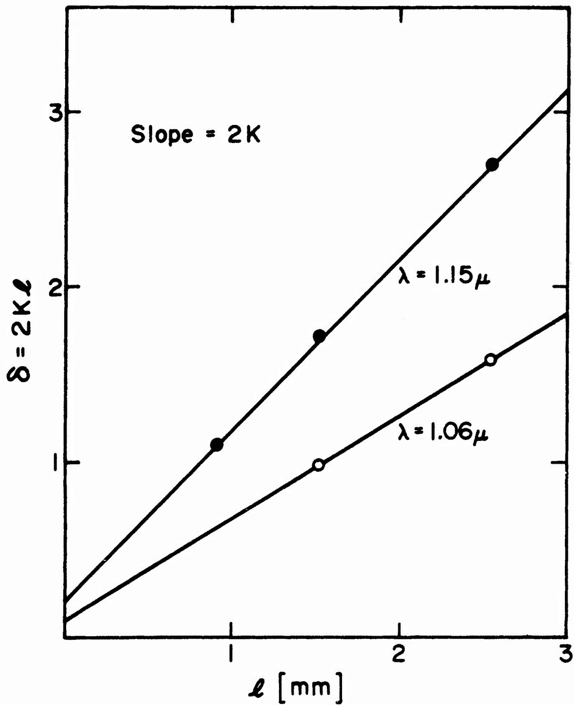
Fig. II.11 Plot of the arguments of the Bessel functions against the distance of propagation.
