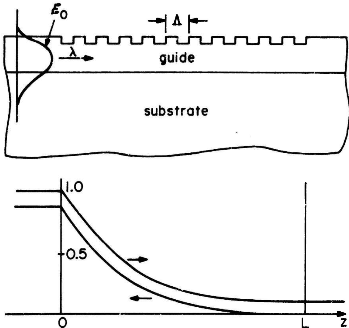
Fig. I.5 Bragg reflection from a distributed mirror, made of corrugation on the surface of the waveguide. The input beam decays as a function of z , giving rise to the reflected beam.
