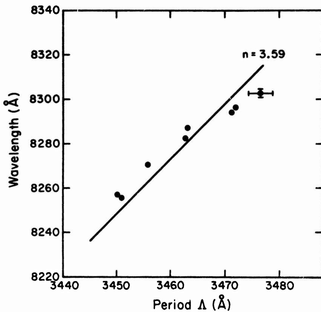
Fig. III.11. Oscillation wavelength as a function of corrugation period. The third order component of the corrugation is the Bragg reflector
