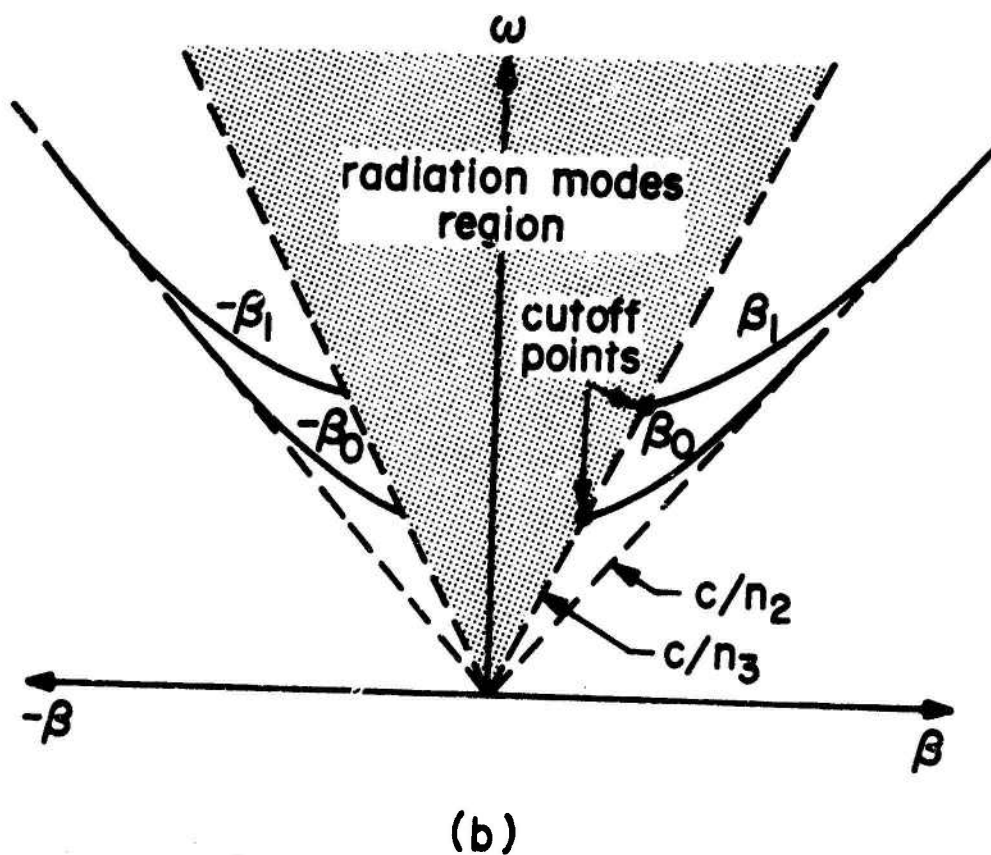
Fig. A.1 (a) The basic configuration of a planar dielectric waveguide. (b) Mode dispersion in the above waveguide.
