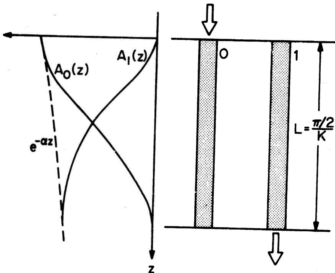
Fig. II.3 Sketch of a dual optical directional coupler showing flow of light energy between the guides.
