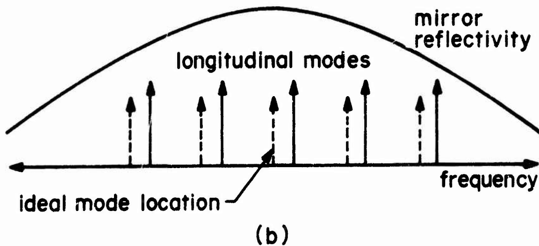
Fig. III.4. (a) A laser, formed by two distributed mirrors. (b) Longitudinal mode spectrum of the above laser.
