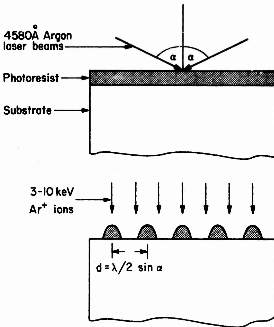
Fig IV.2 (a) Holographic exposure of photoresist. (b) Ion machining of photoresist after development.
