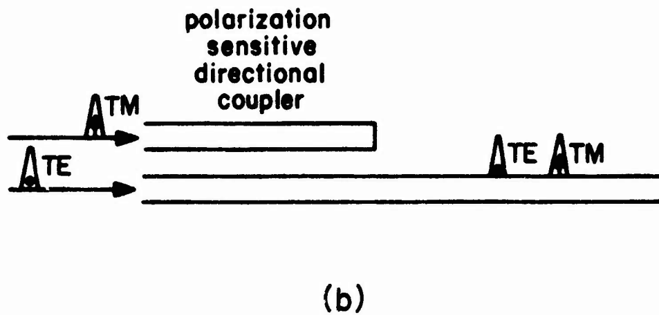
Fig. II.18 (a) Combination of a phase modulator and a polarization sensitive directional coupler. (b) Polarization sensitive directional coupler as a multiplexer.
