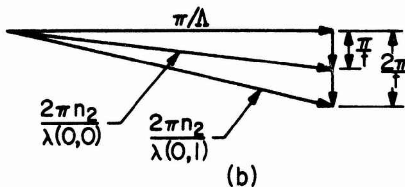
Fig. III.12. (a) Different transverse modes in a rectangular cross section laser. (b) \vec{k} vector diagram in a distributed feedback laser of thickness t .
