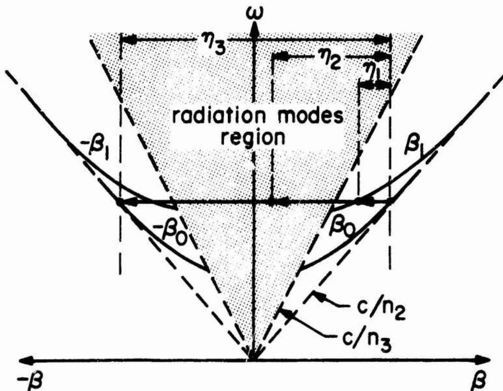
Fig. III.1. (a) Periodically corrugated dielectric waveguide. (b) Mode dispersion and possible interactions in the above guide.
