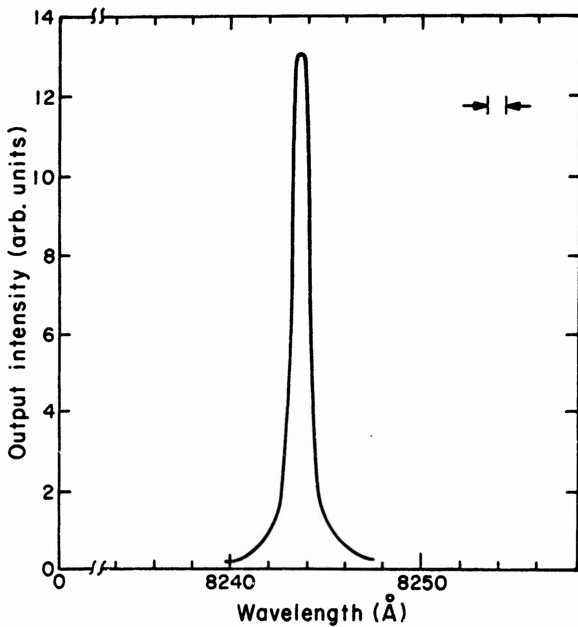
Fig. III.9. The oscillation spectrum of a GaAs waveguide laser. The length of the pumped region was 150 \mu and I/I_{th} = 1.1
