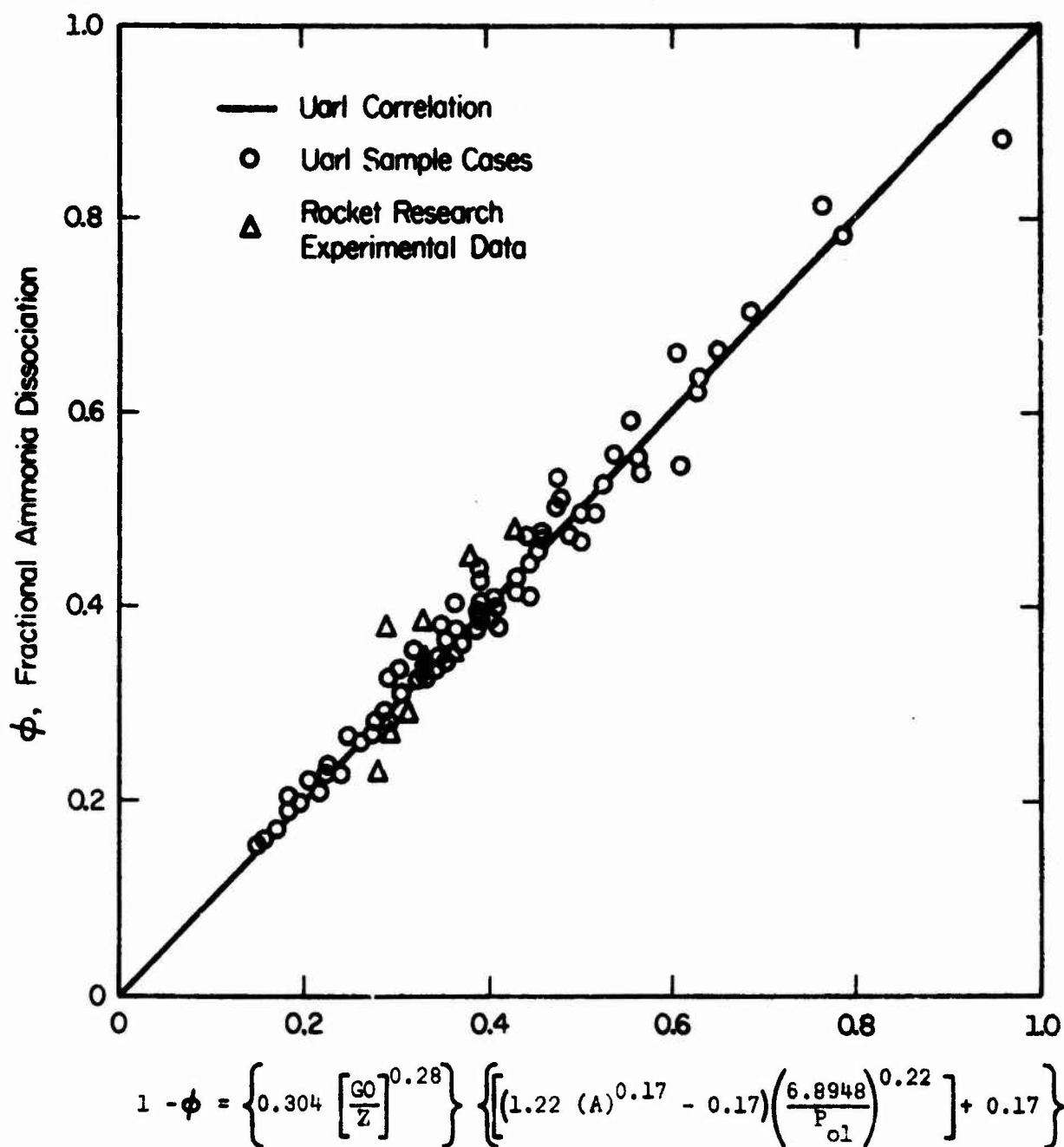
Figure 4 Empirical Correlation for Fractional Ammonia Dissociation in a Hydrazine Decomposition Chamber
