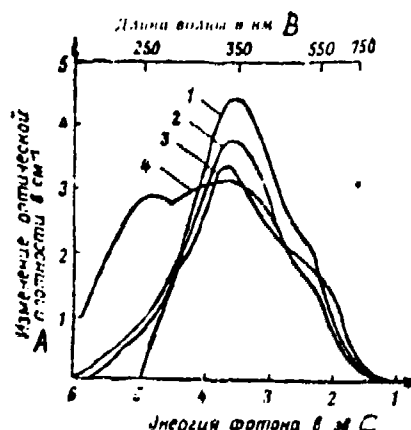
Fig. 11. Effect of replacing CaO with oxides on the radiation stability of a glass (radiation dose 1.15 \cdot 10^7 r) of different compositions, in mole %
