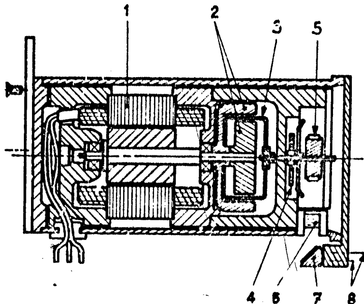
Fig.14(b) Cross section of a P51 tachometer
