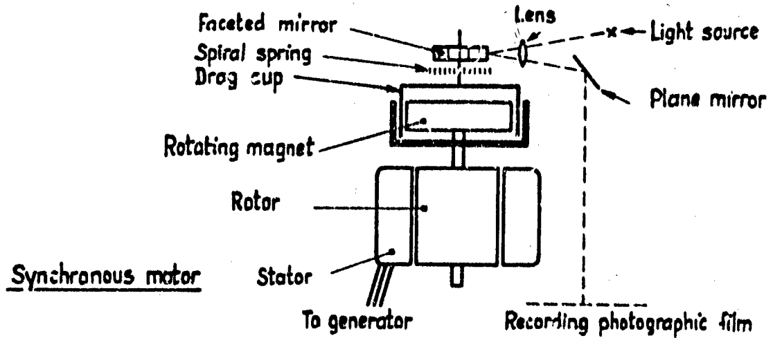
Fig.14(a) Schematic diagram of the P51 tachometer
