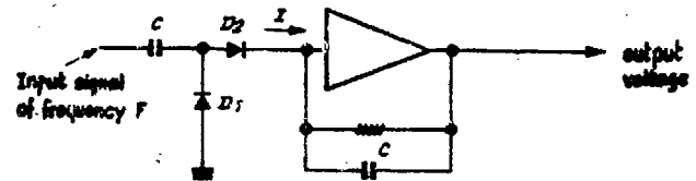
Fig.23 Frequency to voltage conversion using a diode pump
