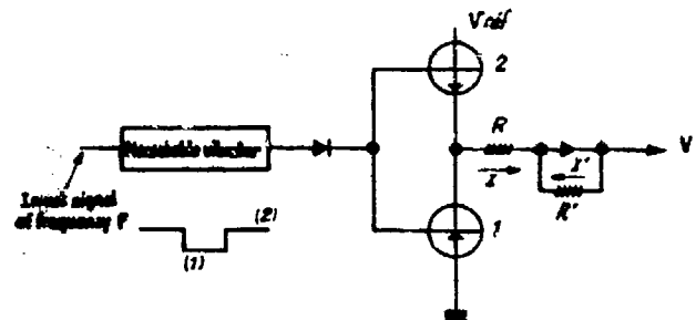
Fig.24 Frequency to voltage conversion using a single vibrator
