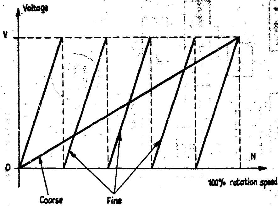
Fig.25 Coarse-fine recording
