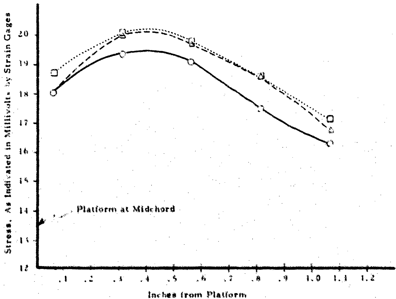
Figure 2. Stress distribution in first bending mode on suction surface at midchord.
