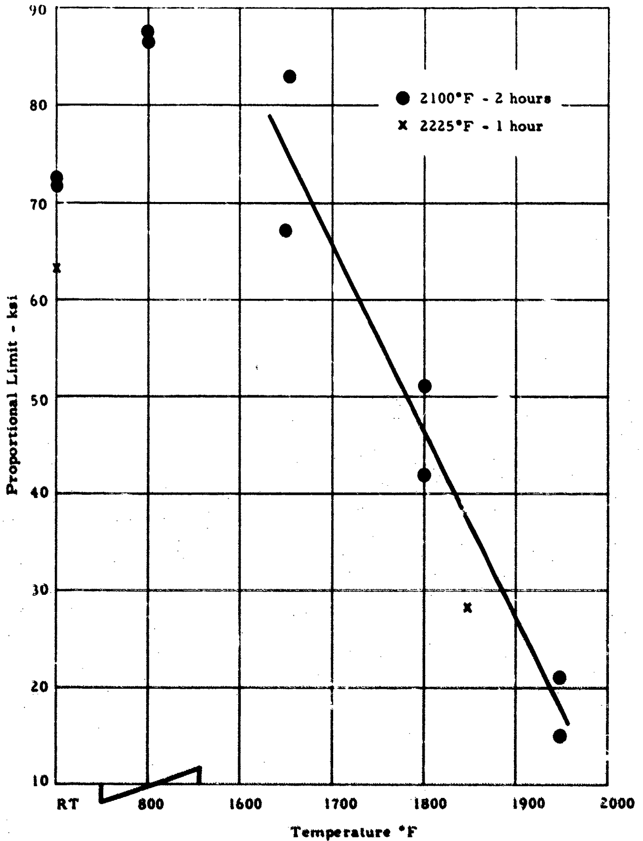
Figure 13. Elevated temperature tensile proportional limit stress of MAR-M246 cast bars.
