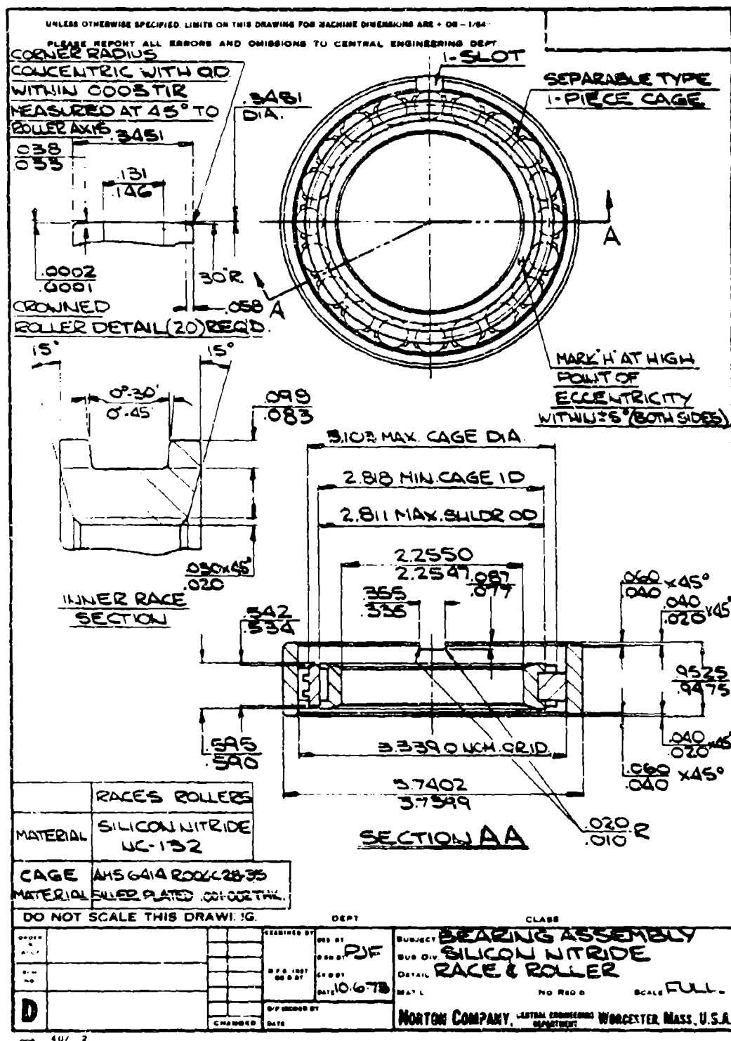
FIGURE 27 - Silicon Nitride Bearing Assembly
