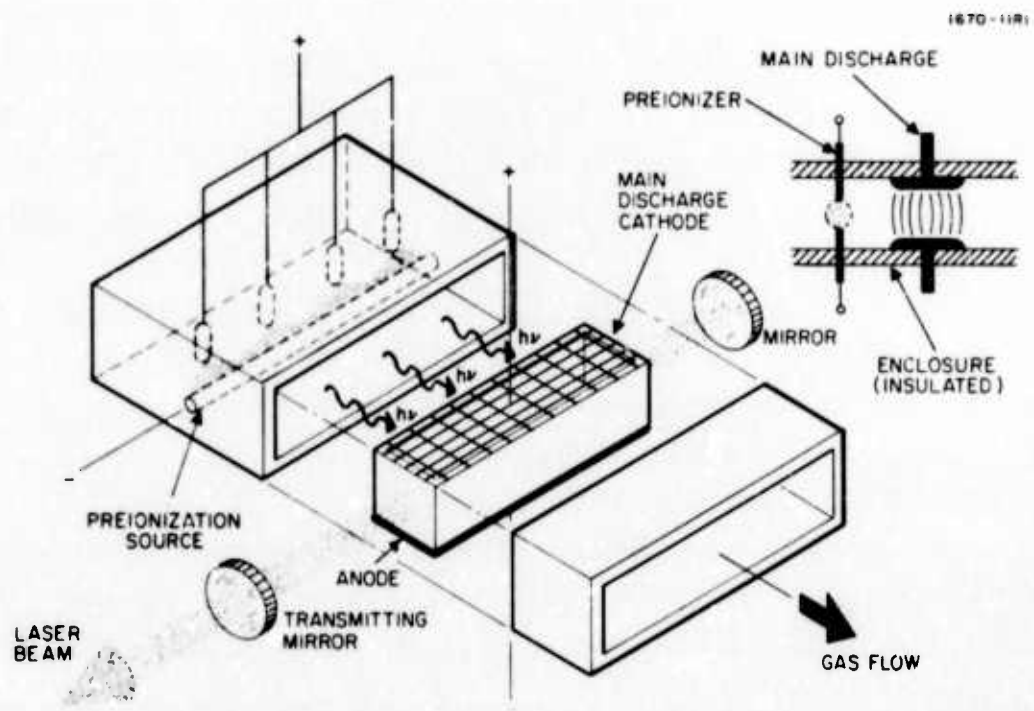
Fig. 1. Simplified schematic diagram of the UV photoionization concept.
