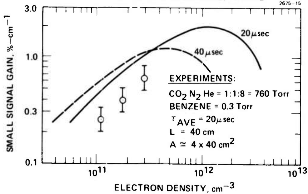
Fig. 34. Gain measurements in UV sustained CO 2 laser.
