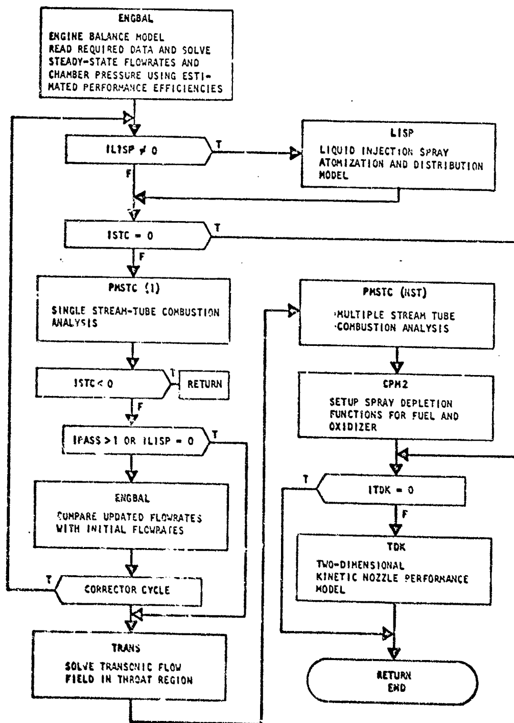
Figure 2. Simplified Flow Chart of PNDER Subprogram
