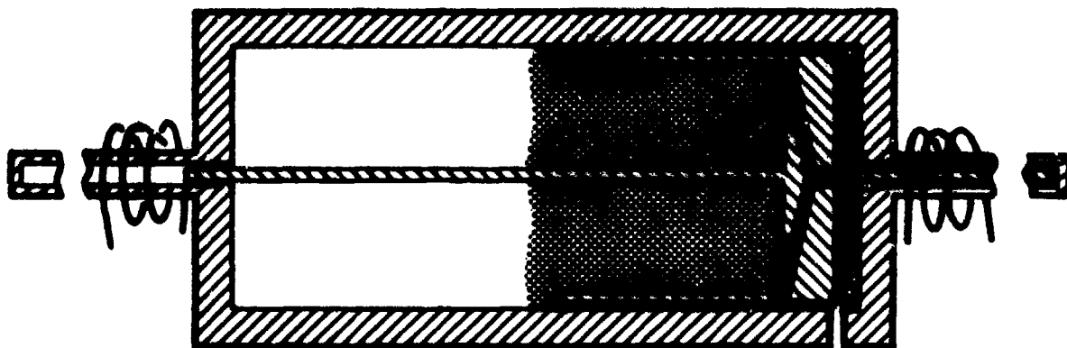
Figure 12. Gas Solubility Cell in Inverted Position
