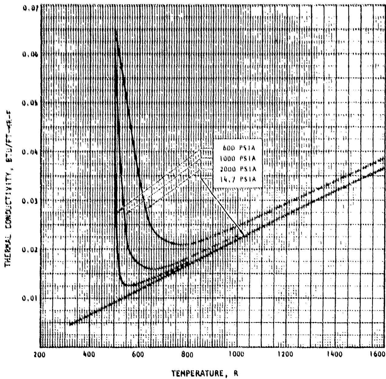
Figure B-9. Thermal Conductivity of Gaseous Nitrous Oxide
