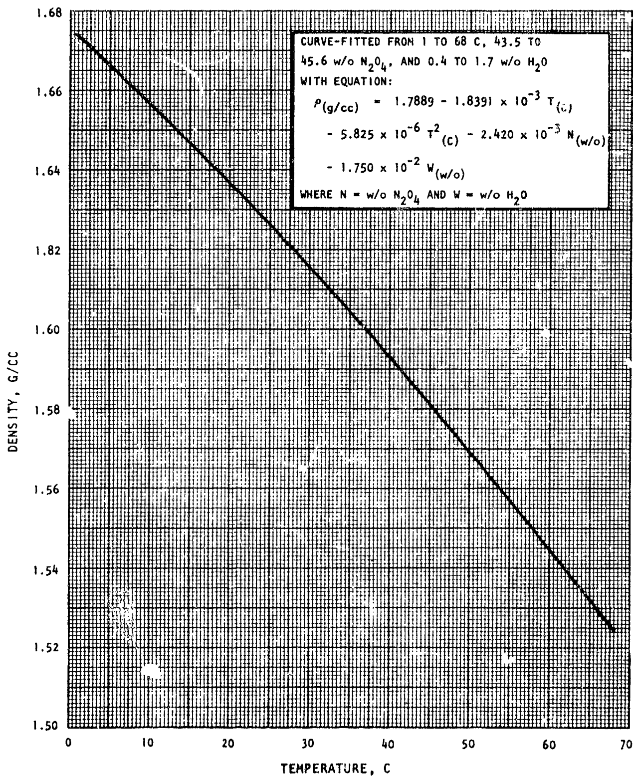
Figure A-1. Density of Saturated Liquid HDA
