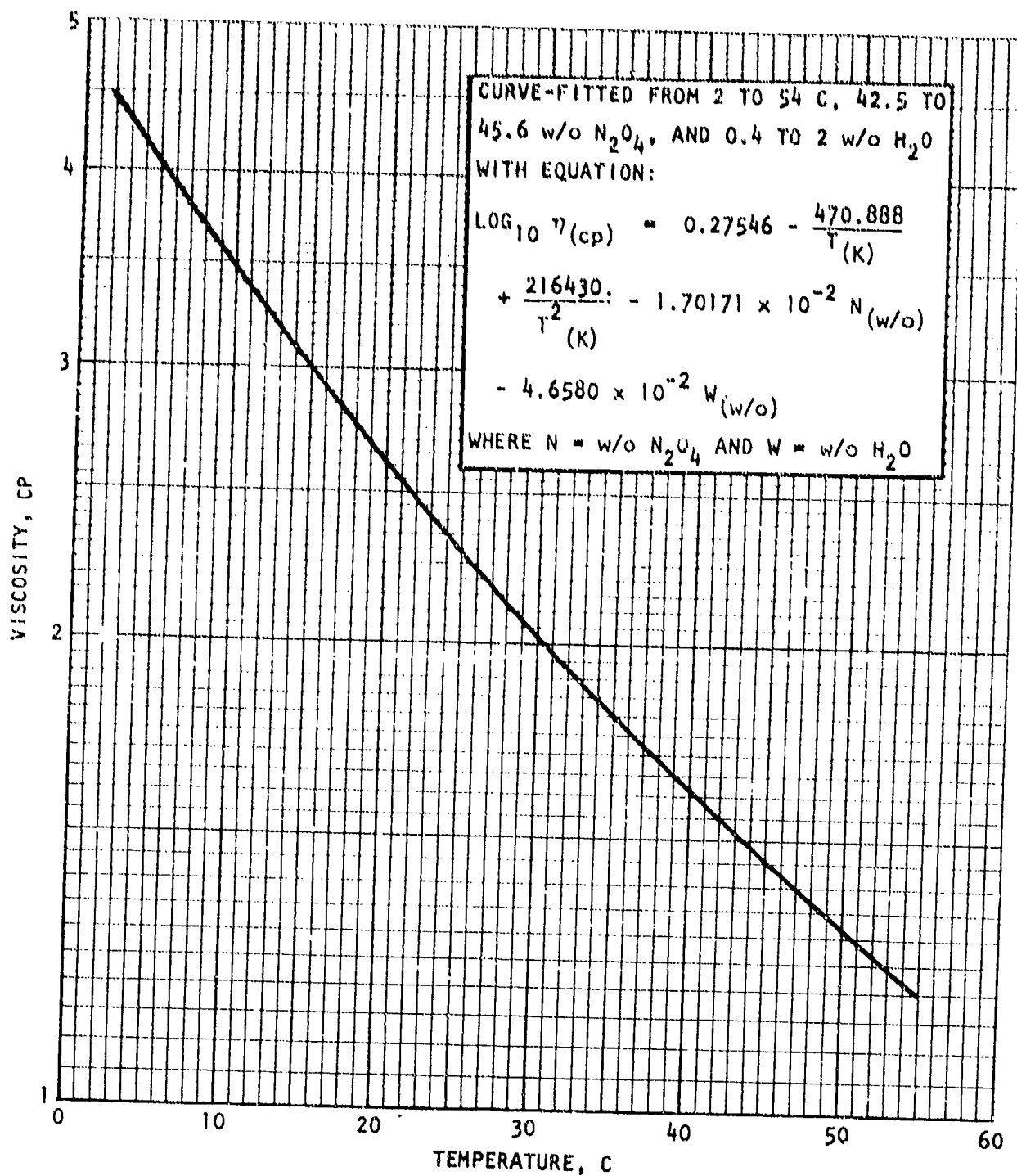
Figure A-5. Viscosity of Saturated Liquid HDA
