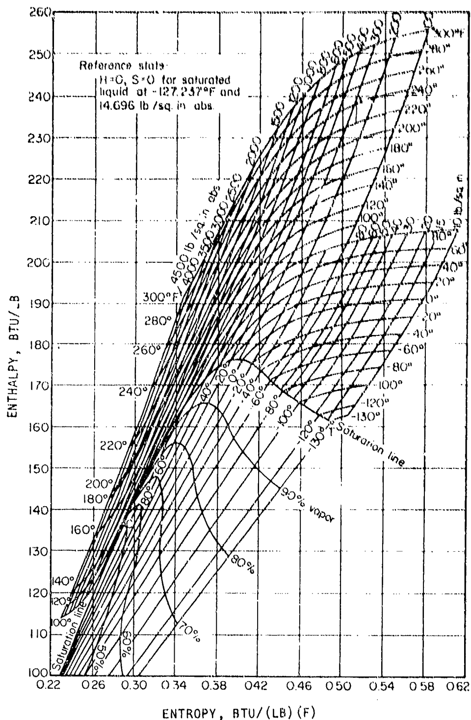
Figure B-7. Enthalpy-Entropy Diagram for Nitrous Oxide (Reprinted from Ref. B-23, as given in Ref. B-24)
