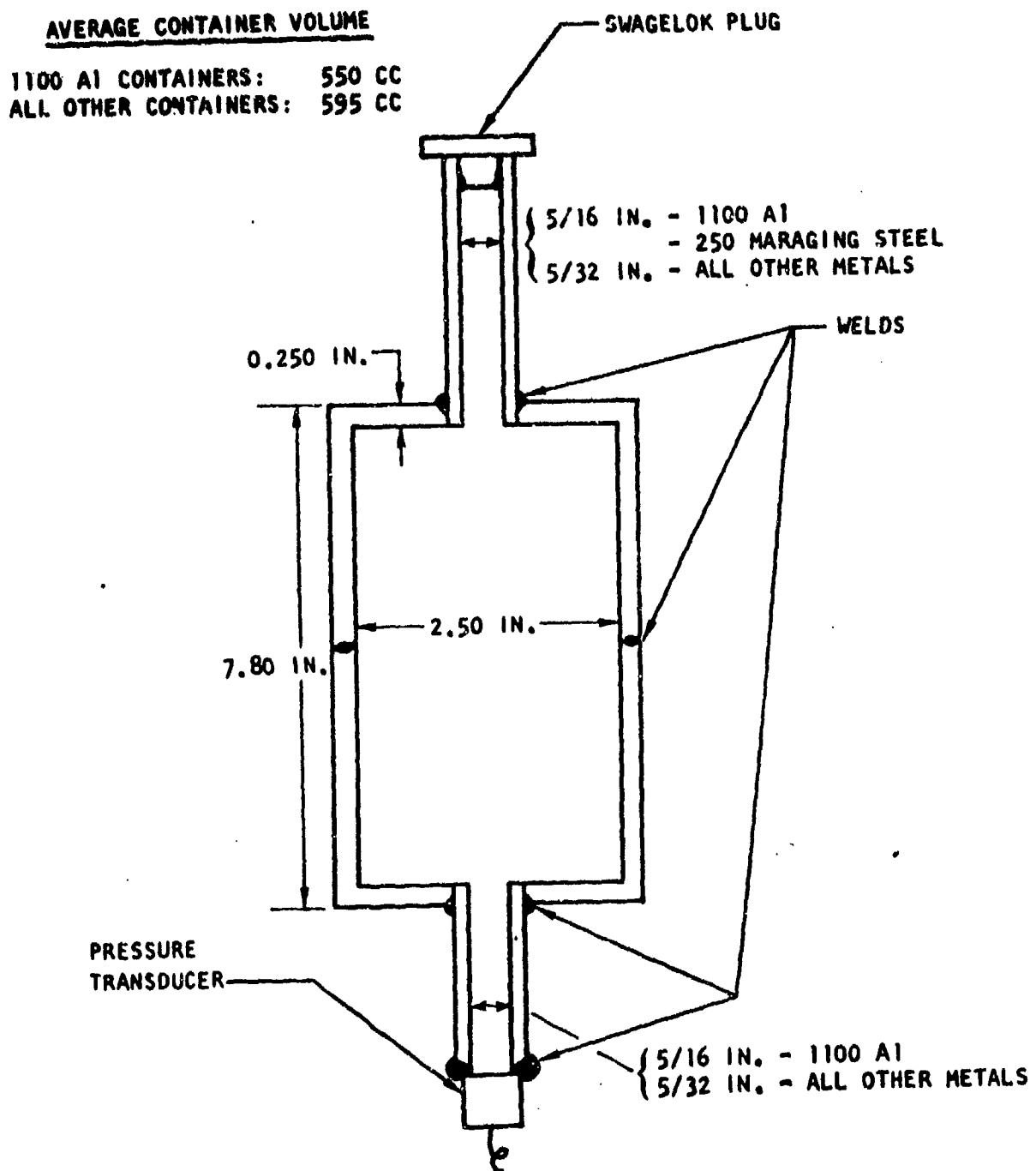
Figure 26. Storability Test Container
