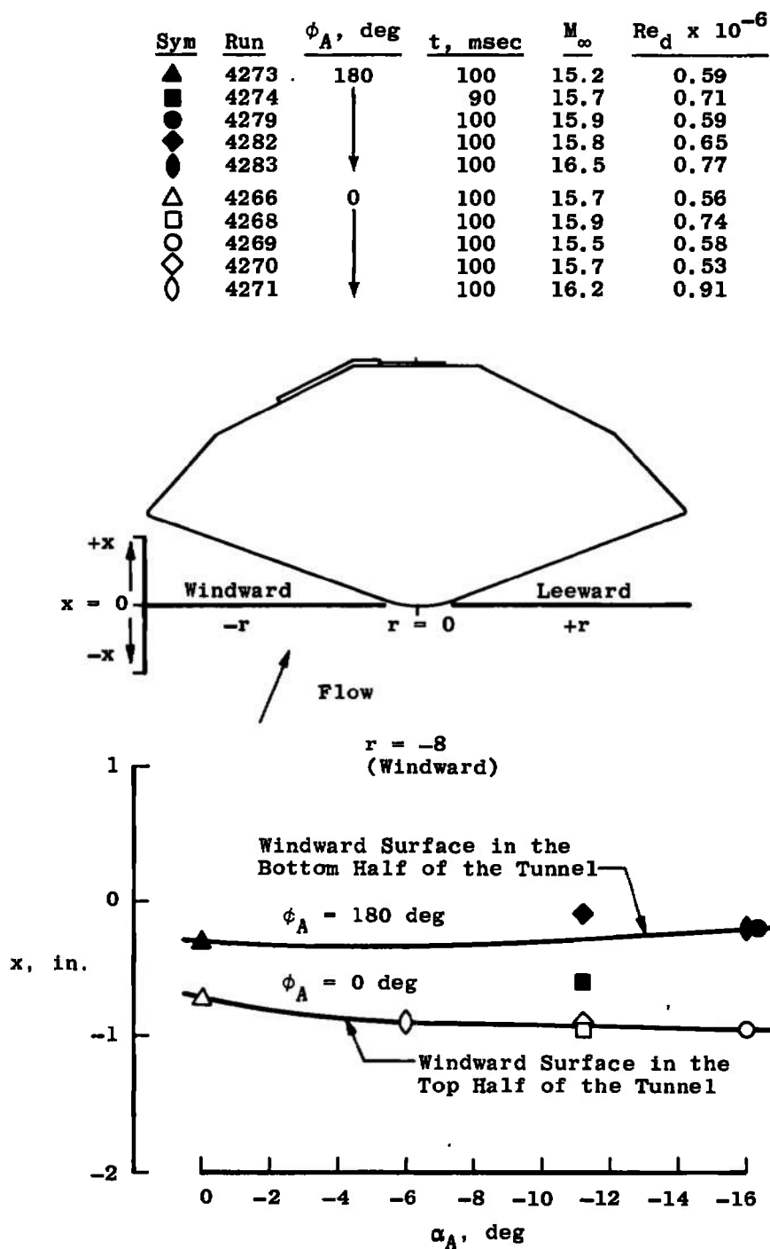
Figure A-3. Variation of bow shock location with angle of attack, r = -8 in.
