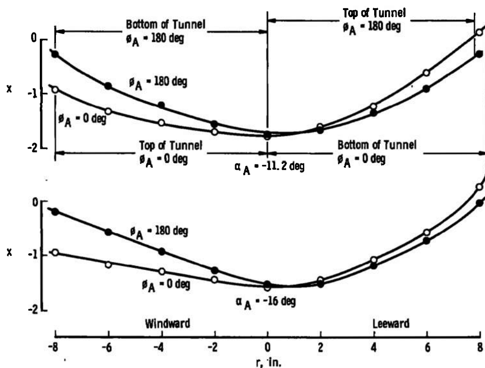
Figure A-5. Bow shock shapes at \alpha_A = -11.2 and -16 deg (model orientation).
