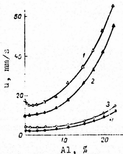
Fig. 2. The dependence of the combustion rate of a mixture of APC + PS + PAK-4 ( \alpha = 2.1 ) on the per cent of aluminum: 1, 2 - p = 100 at; 3, 4 - p = 10 at, 1, 3 - with 1% Fe_3O_2 , 2, 4 - with the catalytic agent.
