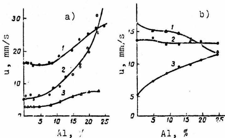
Fig. 3. The dependence of the combustion rate of mixtures of APC + PS + Al on the per cent of aluminum at different \alpha ( p = 40 at): a) d_{Al} \approx 3 \mu m (1 - \alpha = 0.5 ; 2 - \alpha = 2.1 ; 3 - \alpha = 0.15 ); b) d_{Al} \approx 20 \mu m (1 - \alpha = 0.5 ; 2 - \alpha = 1 , 3 - \alpha = 2.1 ).
