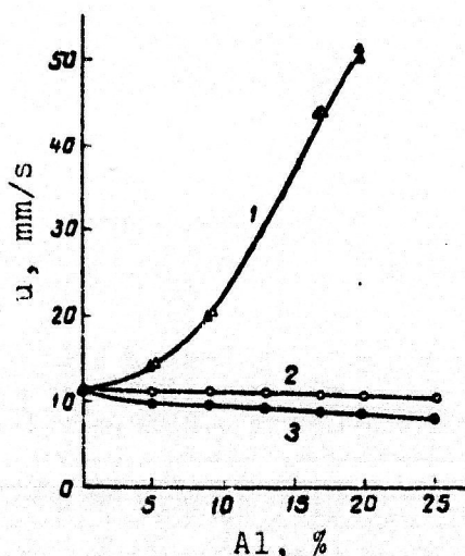
Fig. 4. Dependence of the combustion rate of a PPC + PC + Al mixture ( \alpha = 2 ) on the per cent of aluminum ( p = 40 at): 1 - d_{Al} \approx 3 \mu m ( \Delta - with 1% Fe_2O_3 ; \blacktriangle - without catalytic agent); 2, 3 - d_{Al} \approx 20 \mu m (2 - with 1% Fe_2O_3 ; 3 - without catalytic agent).
