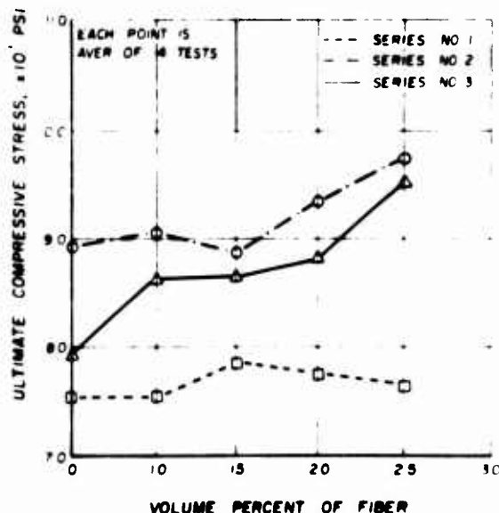
Figure 3. The effect of steel fibers on the compressive strength of 3 x 6 in. cylinders.
