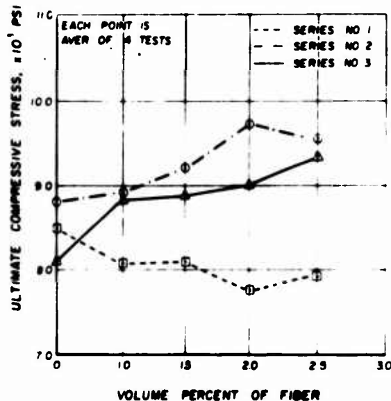
Figure 2. The effect of steel fibers on the compressive strength of 4 x 8 in. cylinders.
