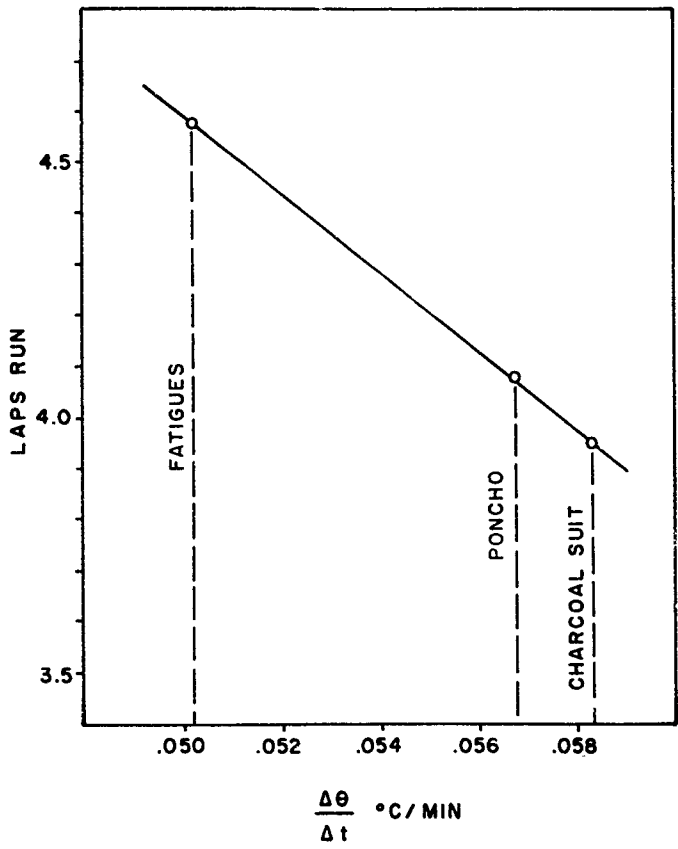
Figure 4. Distance Run as a Function of Heat Load
