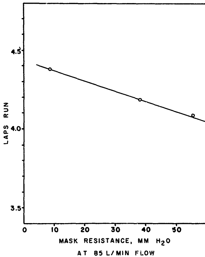
Figure 3. Distance Run as a Function of Mask Resistance
