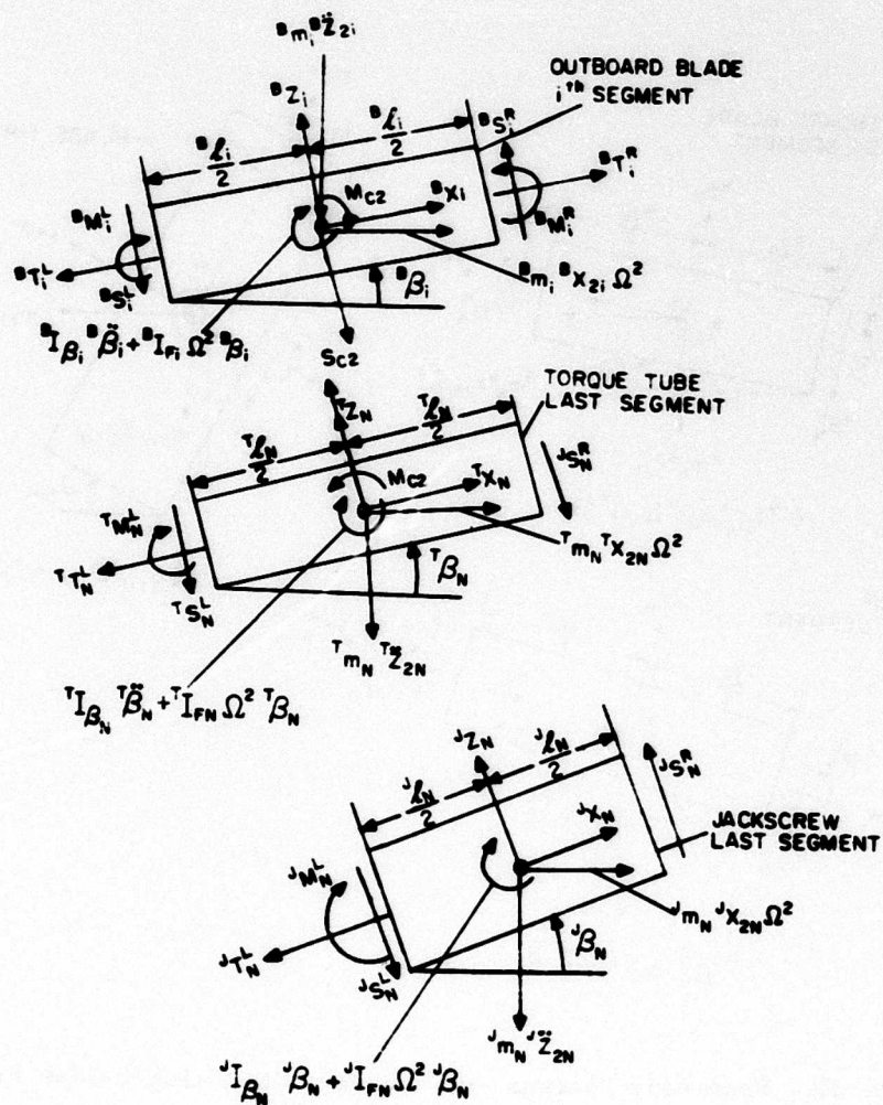
Figure 37. Free-Body Diagrams for Boundary Conditions 2 and 5 (See Figure 7).
