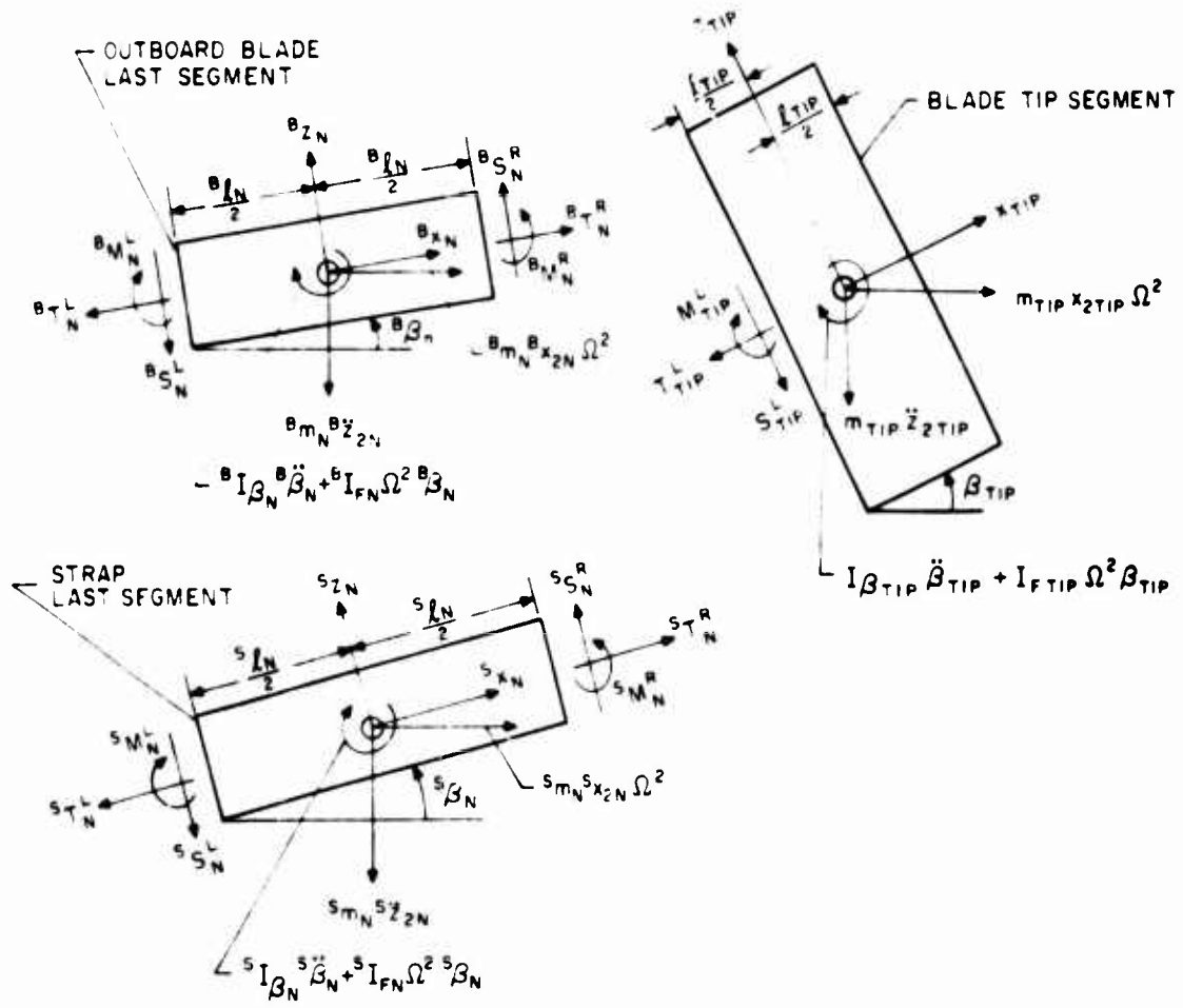
Figure 38. Free-Body Diagram for Boundary Condition 6 (See Figure 7).
