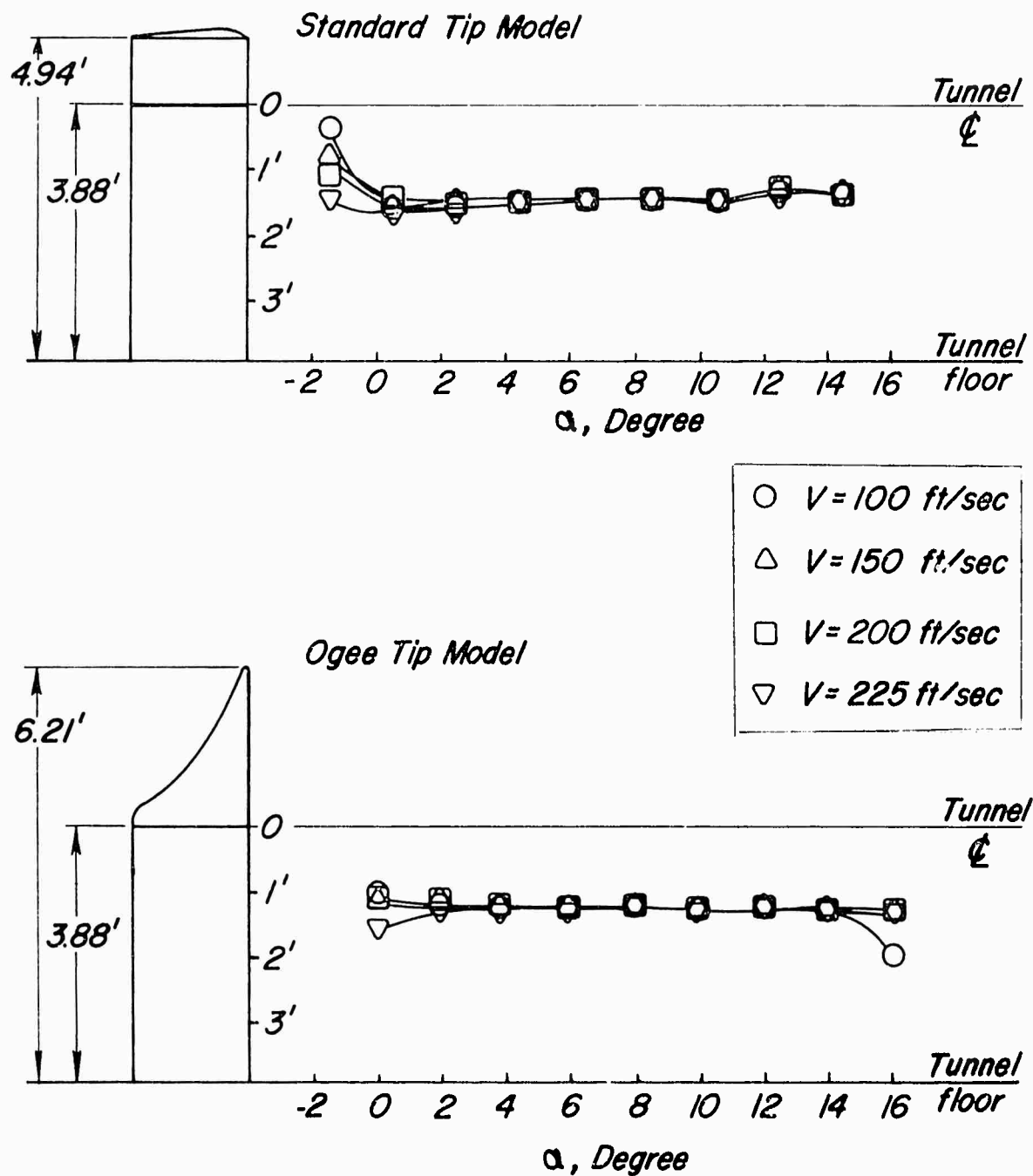
Figure 16. Variation of the Spanwise Lift Center Vs. Angle of Attack for the Standard-Tip and Ogee-Tip Configurations.
