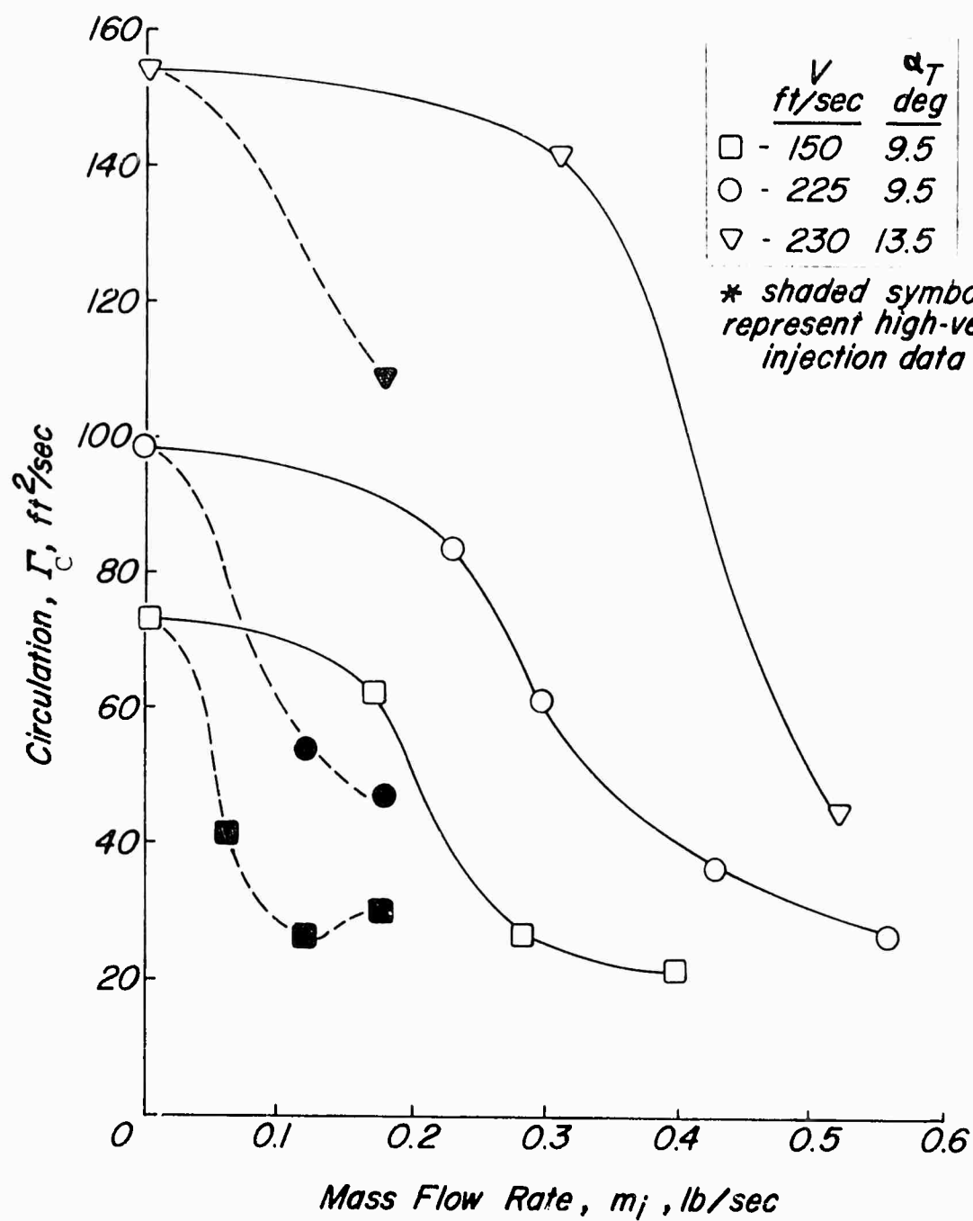
Figure 7. Circulation Vs. Mass Flow Rate at High-Velocity Injection.
