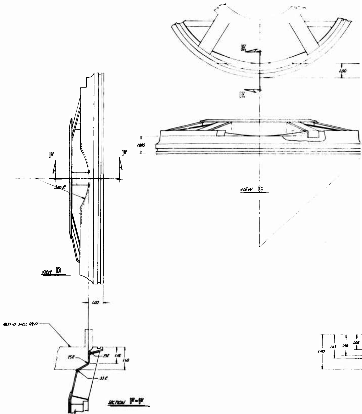
Figure 11. Base Disc Assembly - Helicopter Transmission Housing (WRD Drawing No. 4692).
