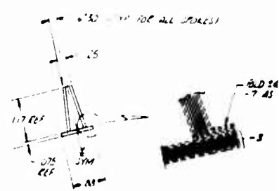
SECTION B-B TYP CROSS SECTION OF (S) SPARKS
