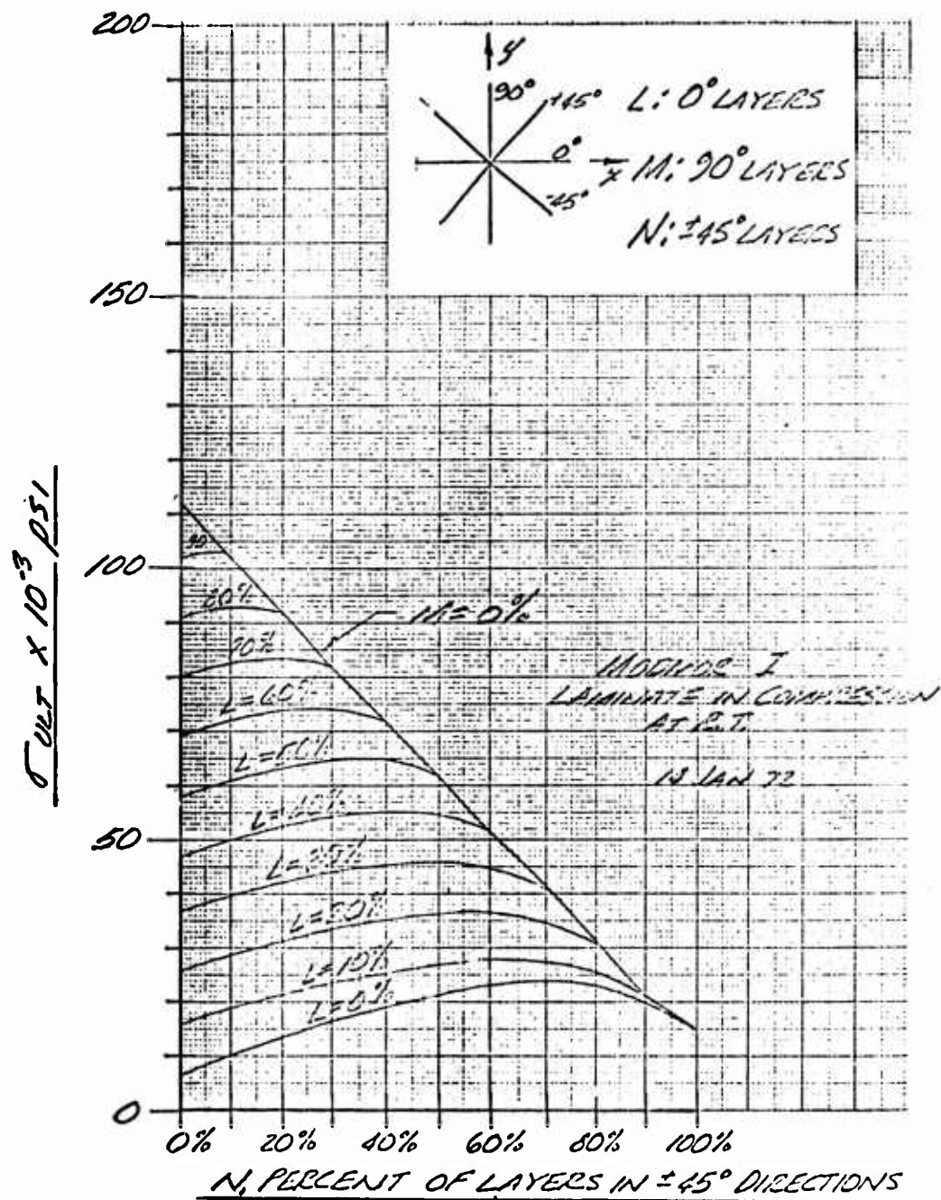
Figure 40. Ultimate Compression Strength of Modmor I/Epoxy [0^\circ, 90^\circ, \pm 45^\circ] Composite Laminate at RT.
