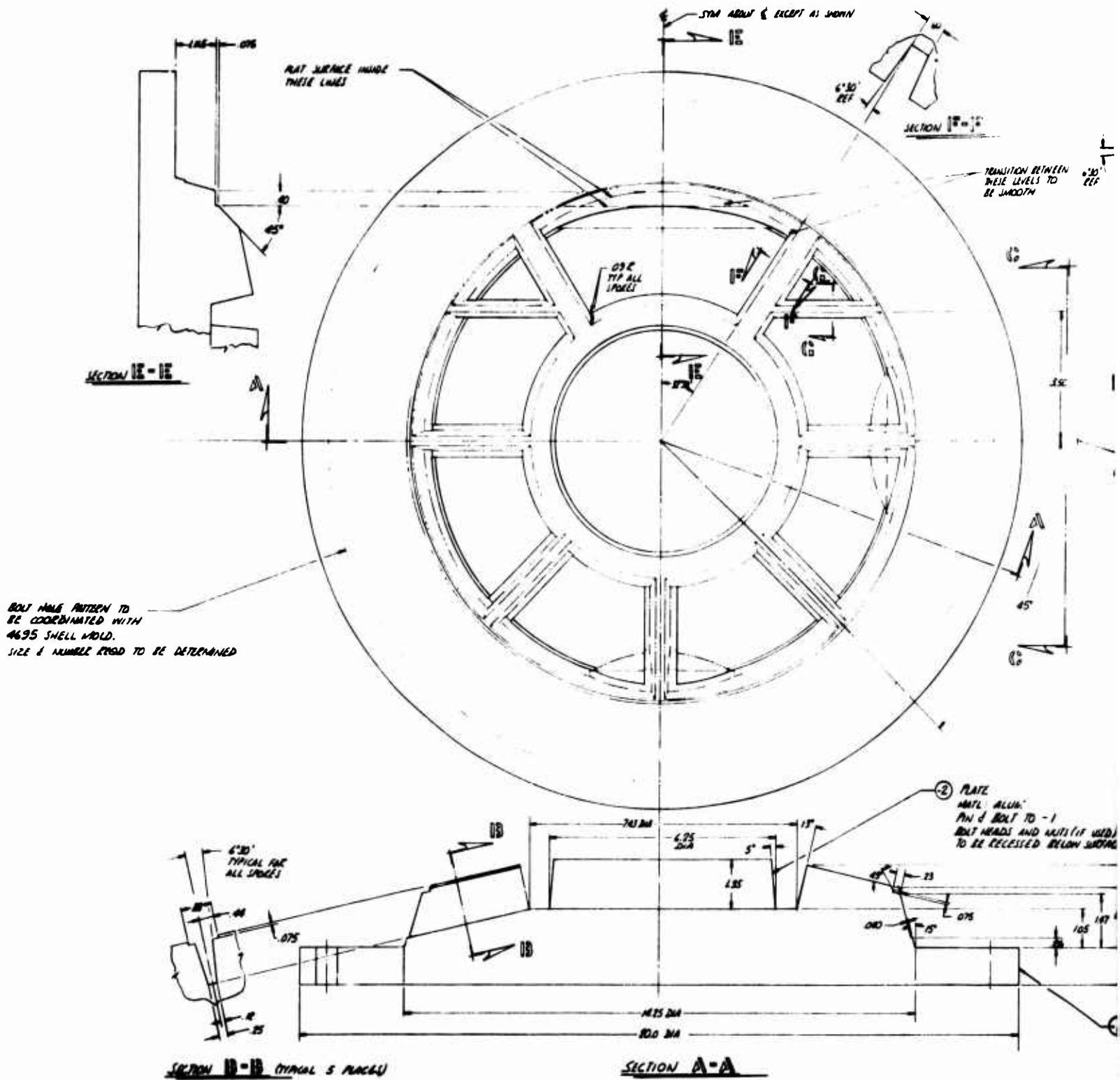
Figure 15. Base Disc Mold - Helicopter Transmission Housing (WRD Drawing No. 4696).
