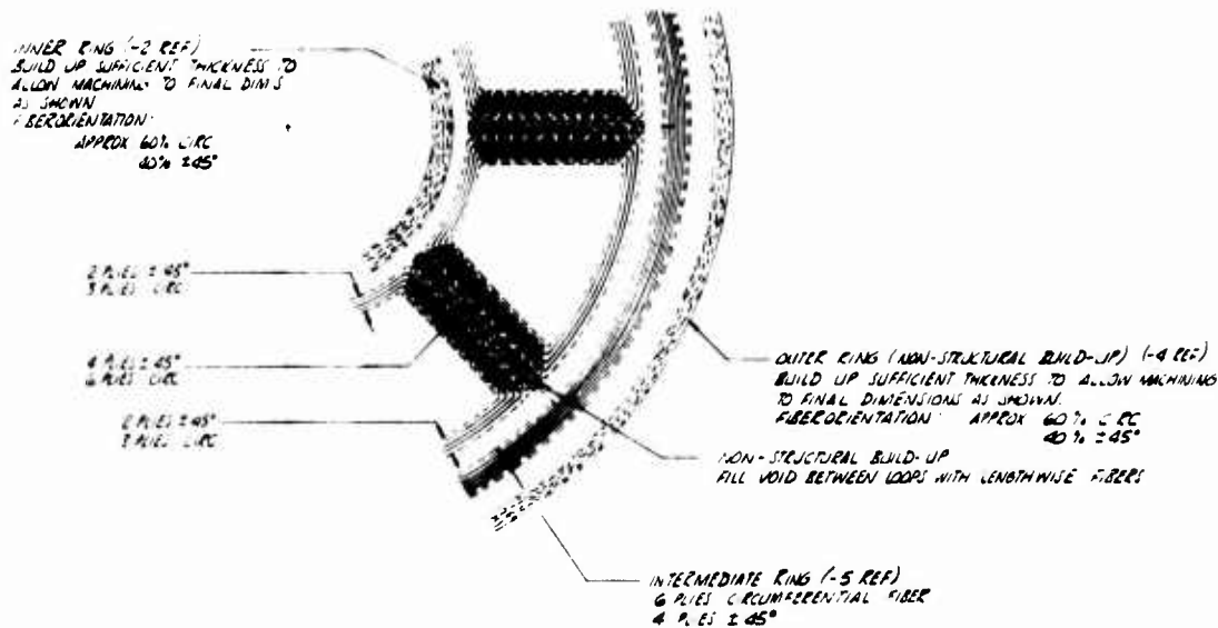
SCHEMATIC OF FIBER LAY-UP
