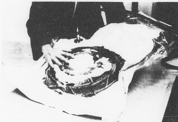
Figure 24. Bagged Wheel-Shaped Bearing Support After Removal From Autoclave Cure.
