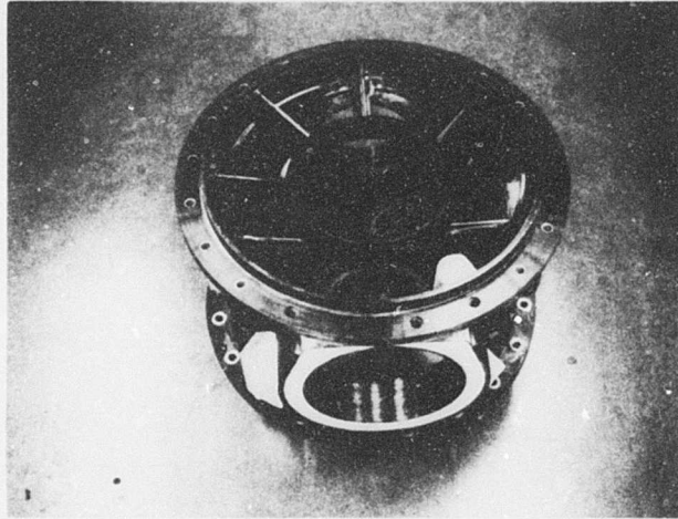
Figure 29. Completed Carbon Composite Transmission Housing.
