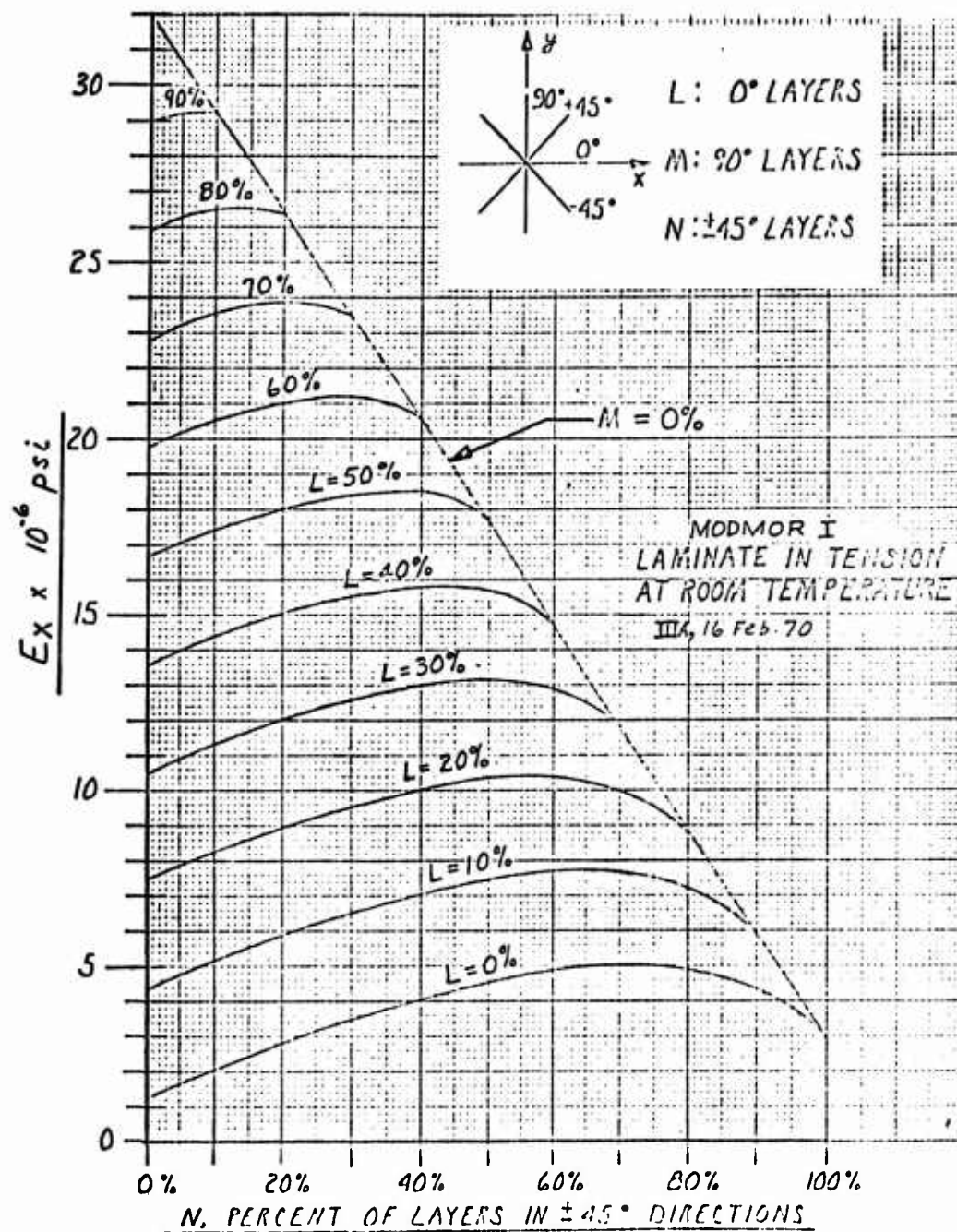
Figure 38. Tensile Modulus of Elasticity for Modmor I/Epoxy [0°, 90°, ± 45°] Composite Laminate.
