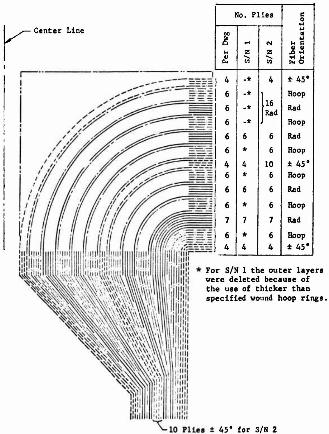
Figure 18. Fiber Layup Schedule for Upper Flange, Showing Difference Between S/N 1 and S/N 2.
