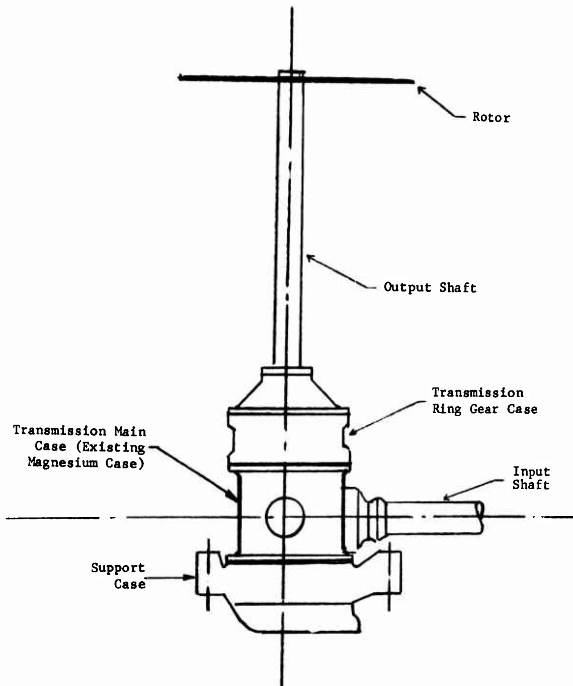
Figure 1. Location of the Transmission Case Within the Gear Case System.
