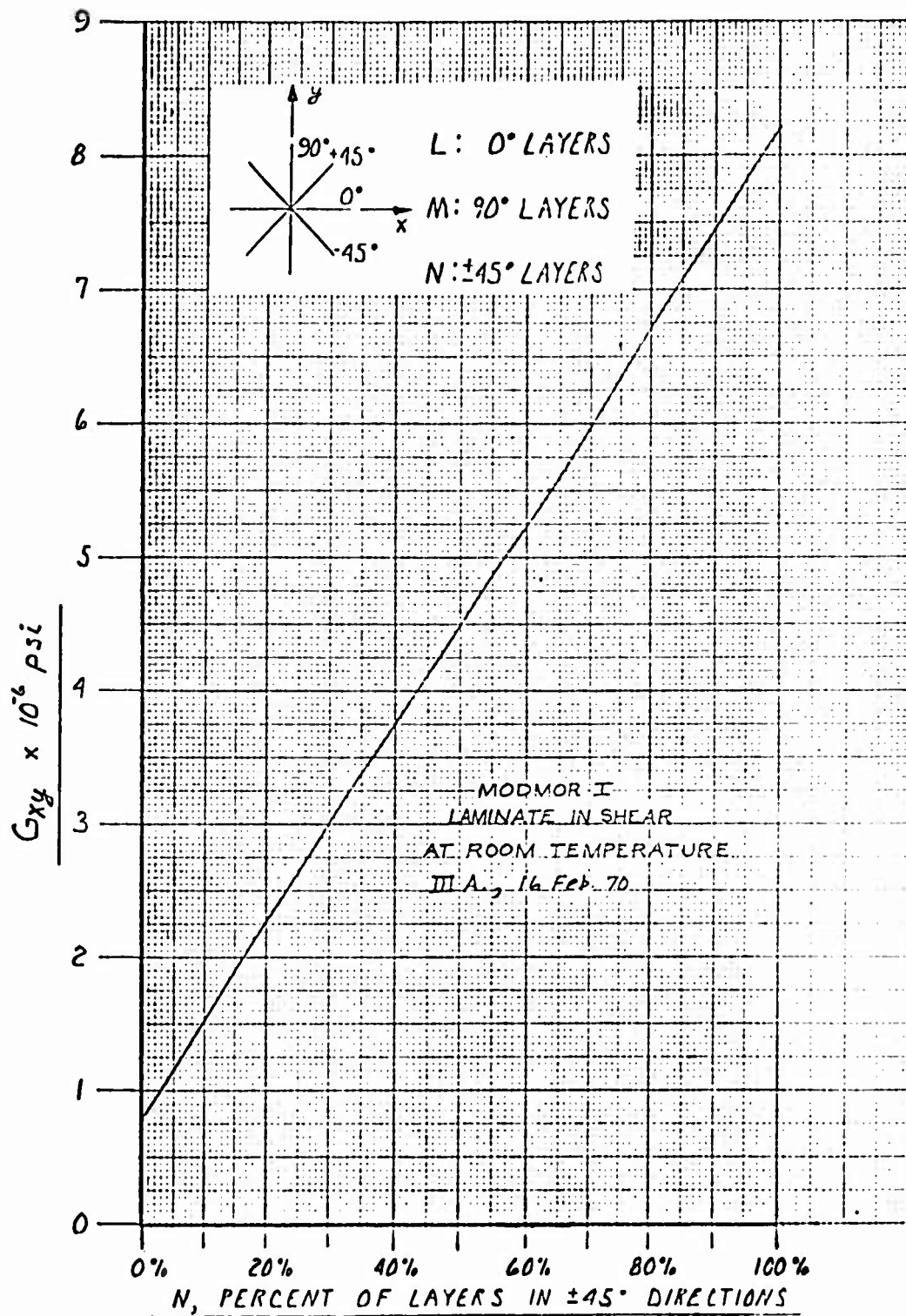
Figure 42. Shear Modulus for Modmor I/Epoxy [ 0^\circ , 90^\circ , \pm 45^\circ ] Composite Laminates.
