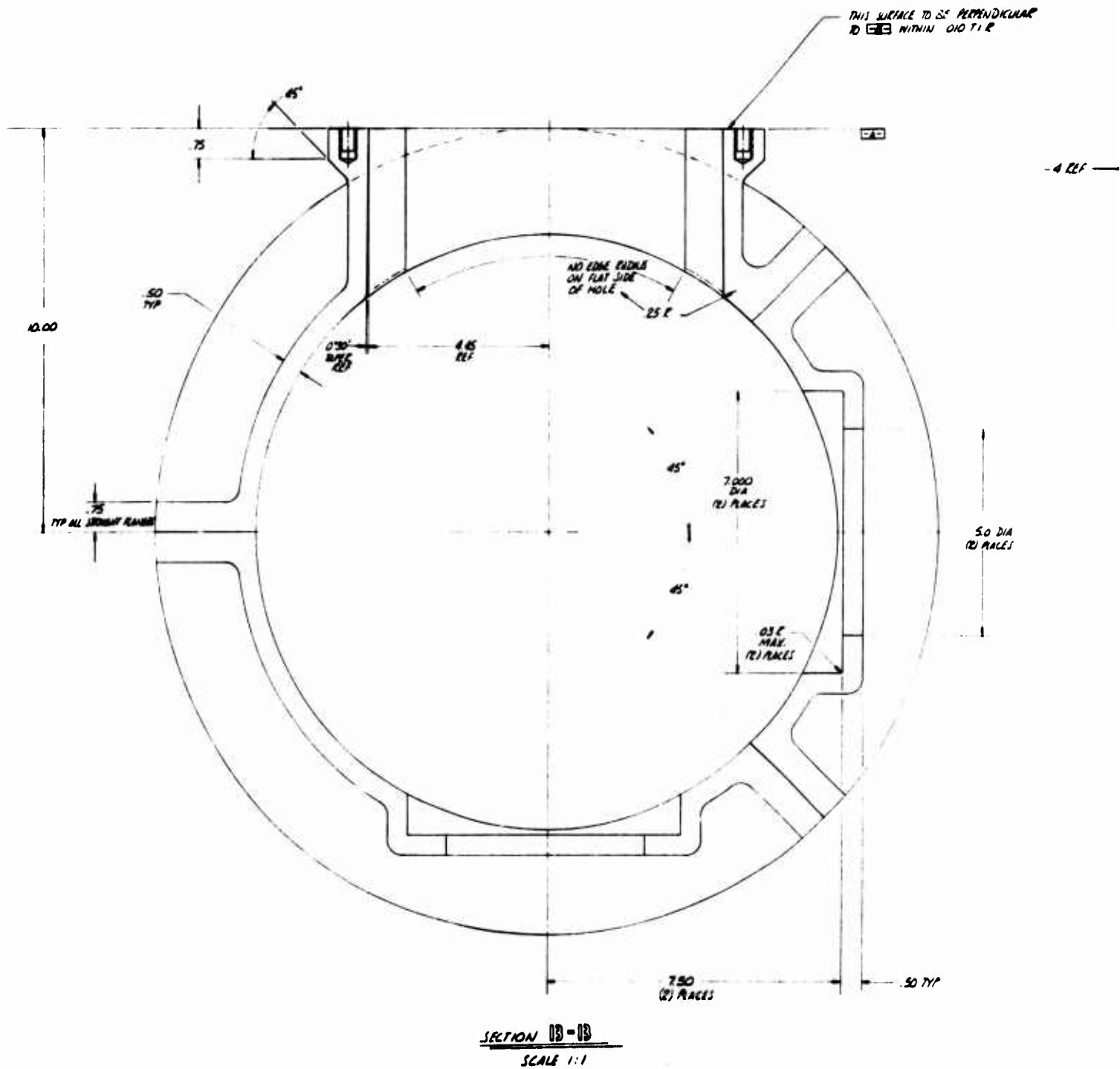
Figure 16. Shell Mold Assembly - Helicopter Transmission Housing (WRD Drawing No. 4695).
