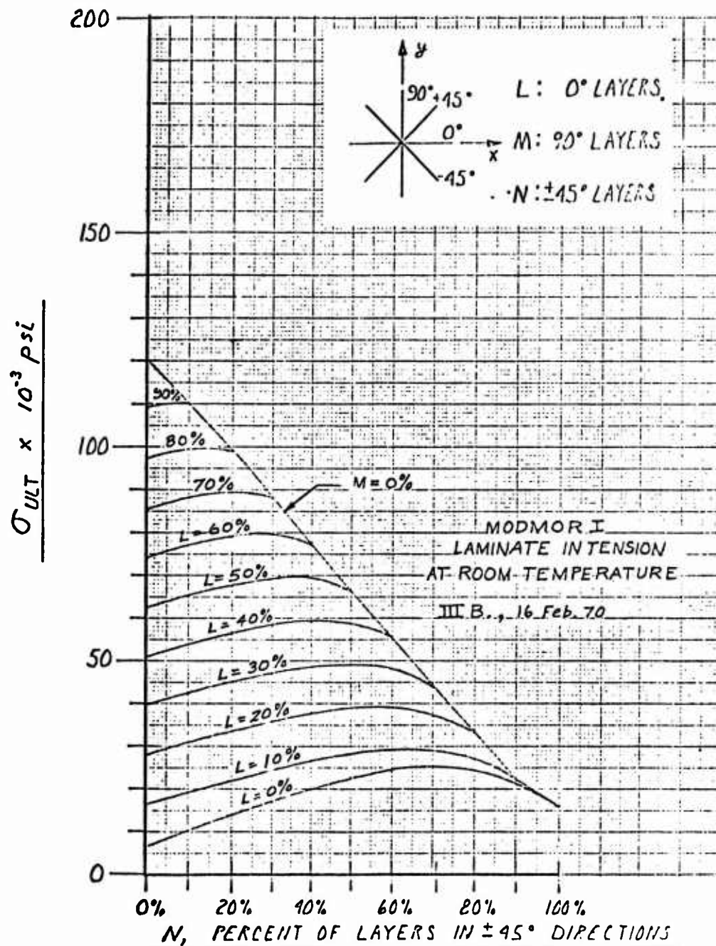
Figure 36. Ultimate Tensile Strength of Modmor I/Epoxy [0^\circ, 90^\circ, \pm 45^\circ] Composite Laminate.
