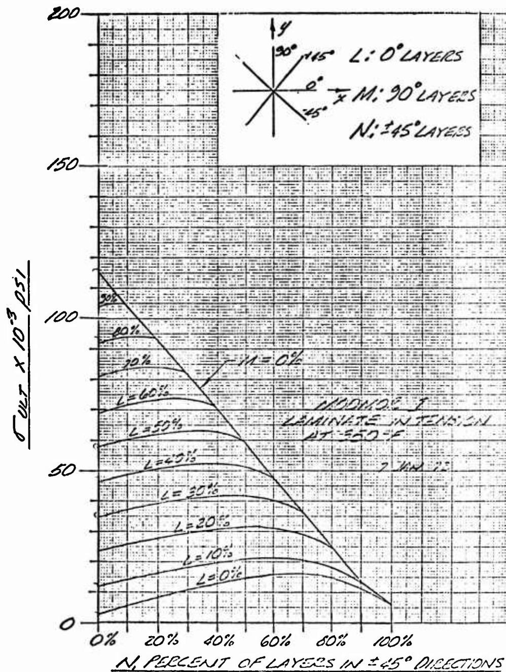
Figure 37. Ultimate Tensile Strength of Modmor I/Epoxy [0°, 90°, \pm 45^\circ ] Composite Laminate at 350°F.
