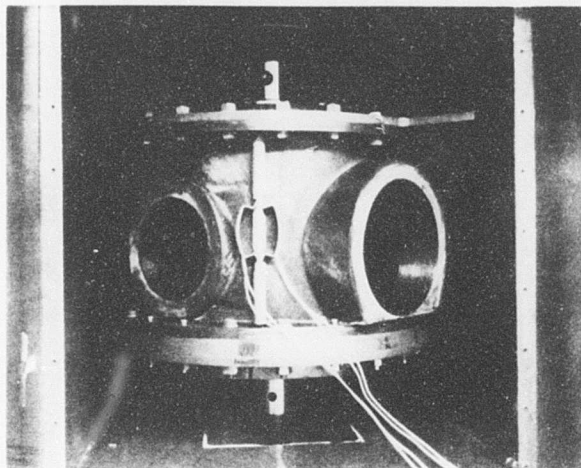
Figure 32. Tension Stiffness Test.
