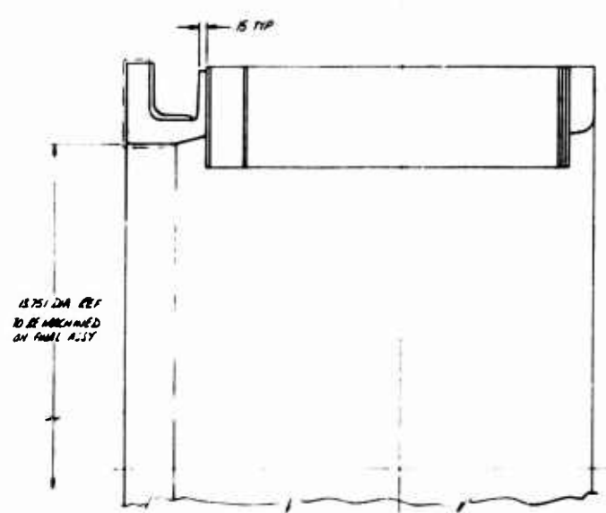
SECTION 13-13
