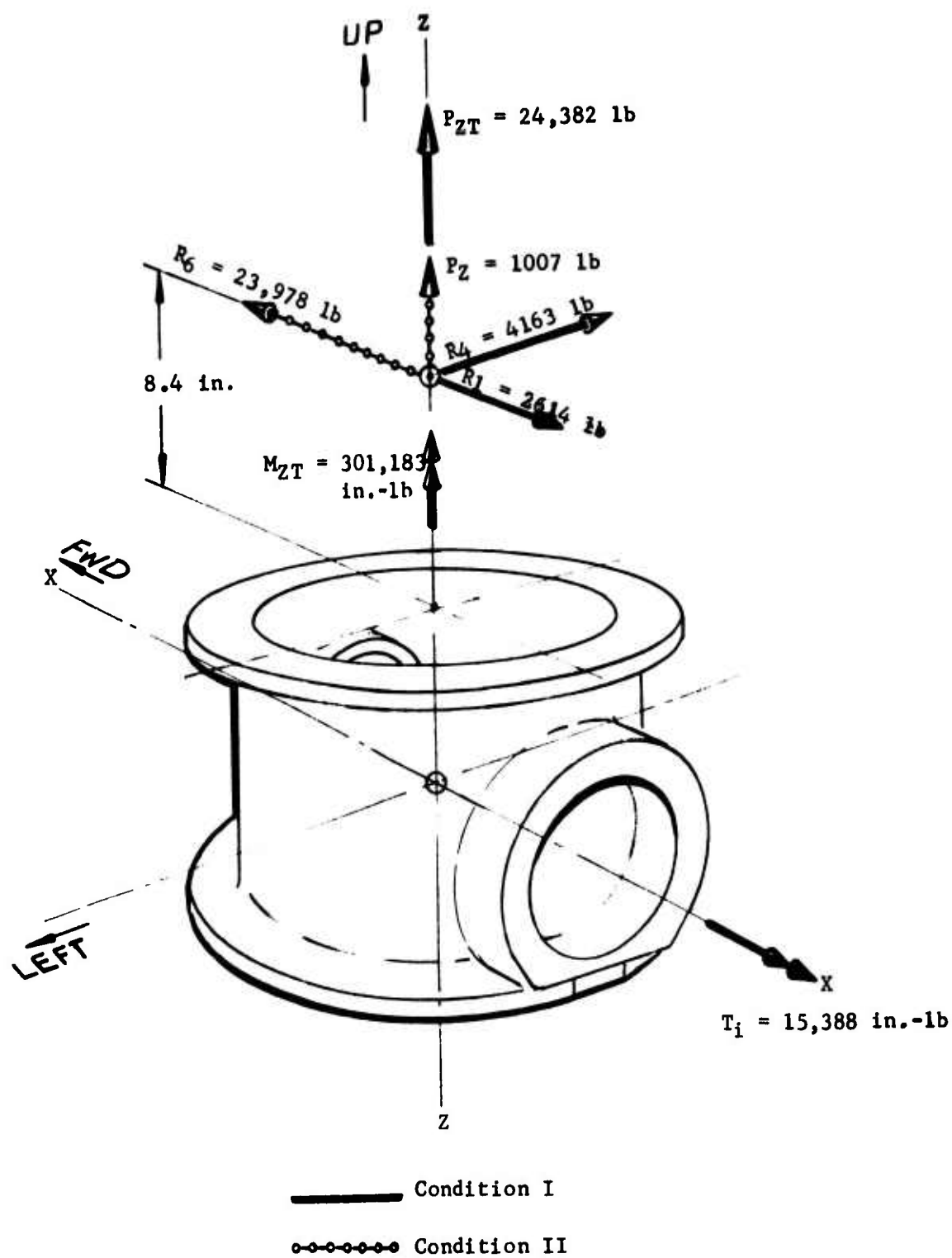
Figure 14. Critical Design Limit Loads.
