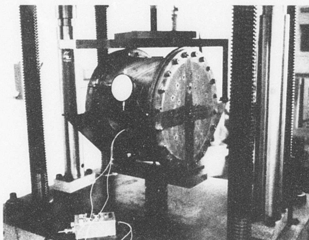
Figure 33. Torsion Stiffness Test.
