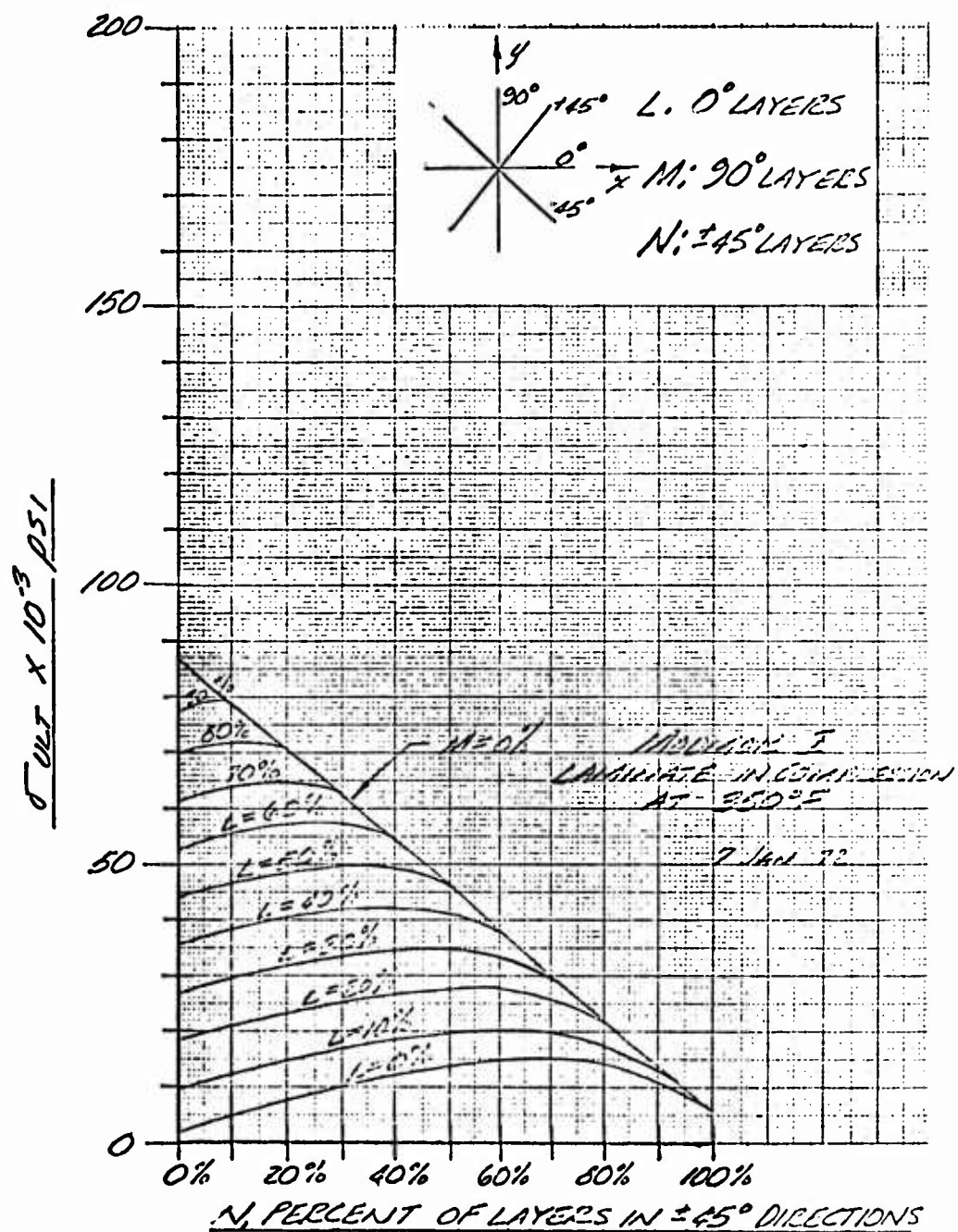
Figure 41. Ultimate Compression Strength of Modmor I/Epoxy [0^\circ, 90^\circ, \pm 45^\circ] Composite Laminate at 350°F.
