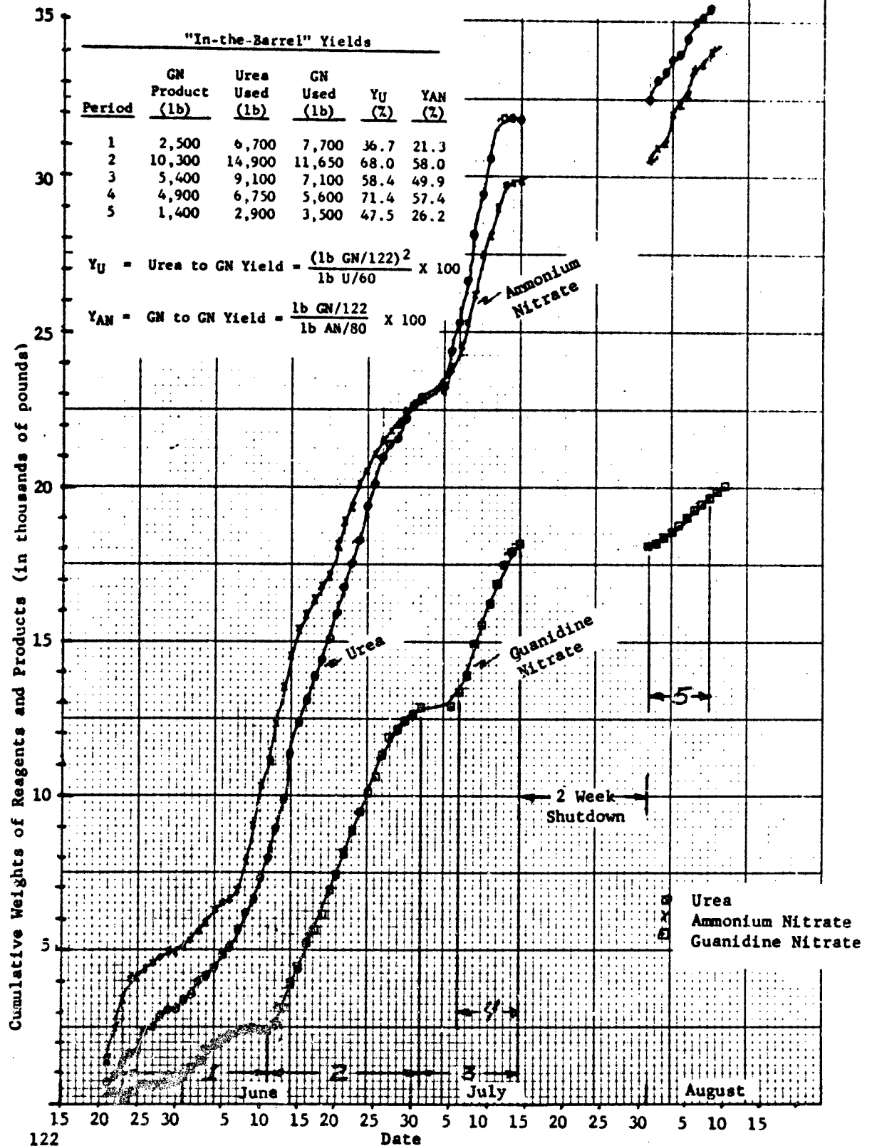
Figure 11. Cumulative Plot of Reactants Used and Guanidine Nitrate Produced Versus Date
