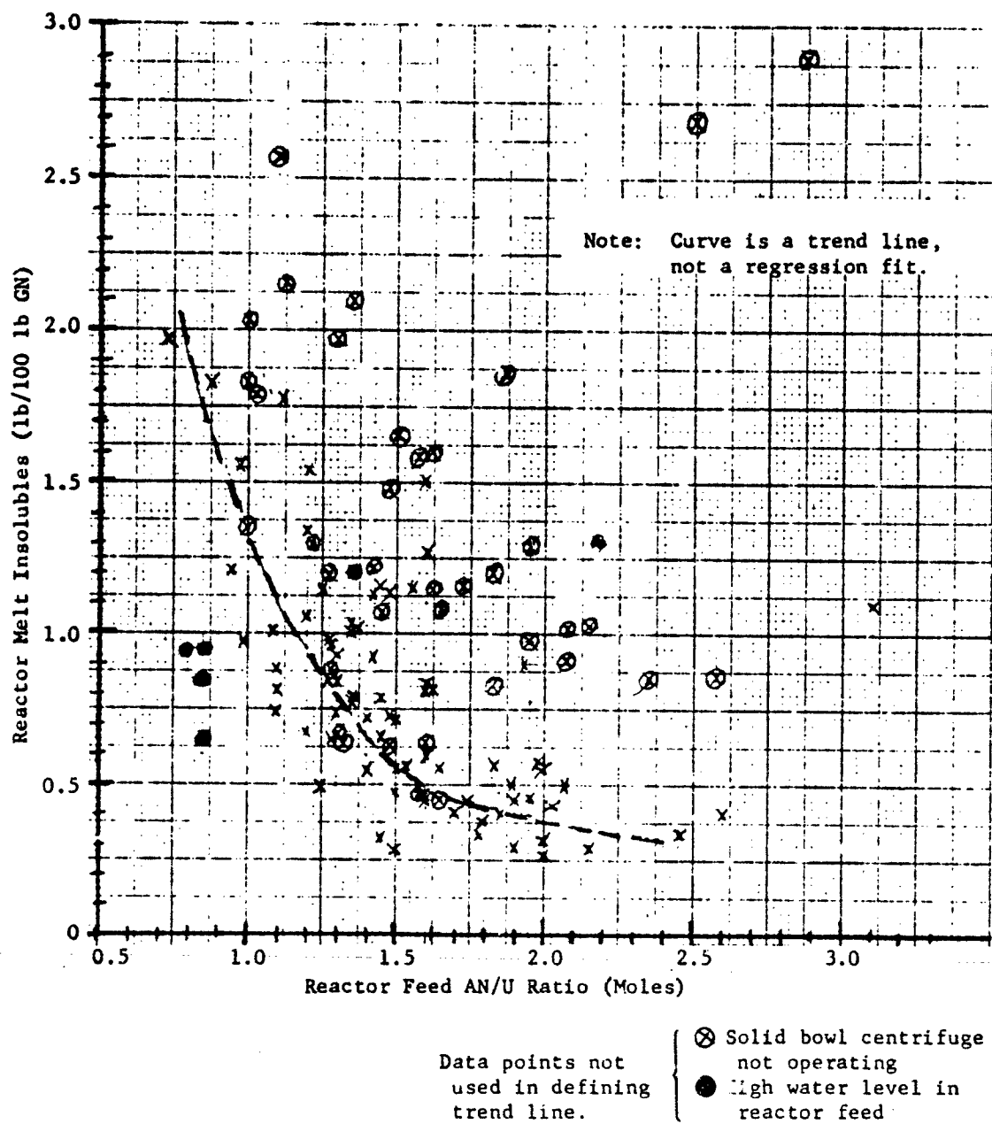
Figure 21. Effect of Reactor Feed AN/U Ratio on Insolubles Formation
