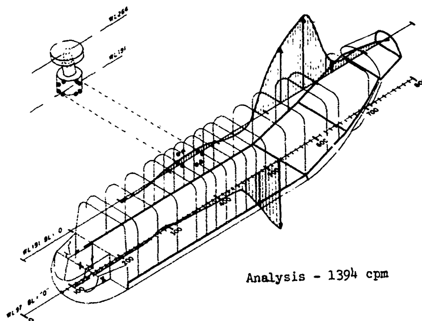
Figure 82 Phase II Correlation of Ramp Vertical Bending Mode, Rigid Ballast
