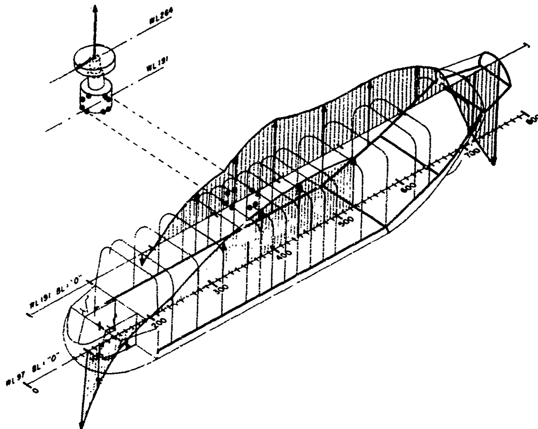
Figure 54 Phase II test - First Vertical Bending Mode 440 rpm
