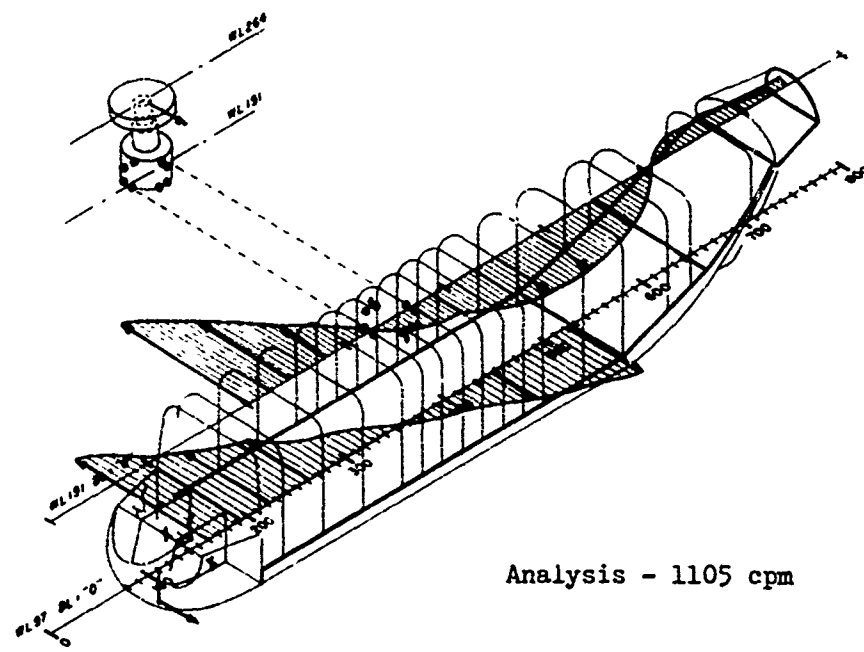
Figure 79 Phase II Correlation of Forward Cabin/Nose Block Lateral Mode, Rigid Ballast
