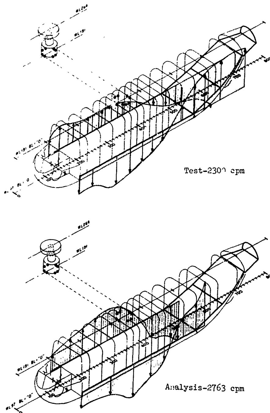
Figure 50 Phase I Correlation of Torsion Mode - 18 Bay
