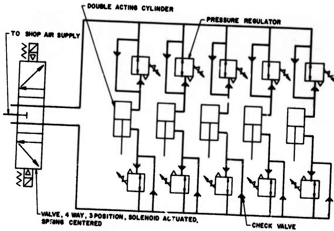
Figure 6. Pneumatic Schematic.
