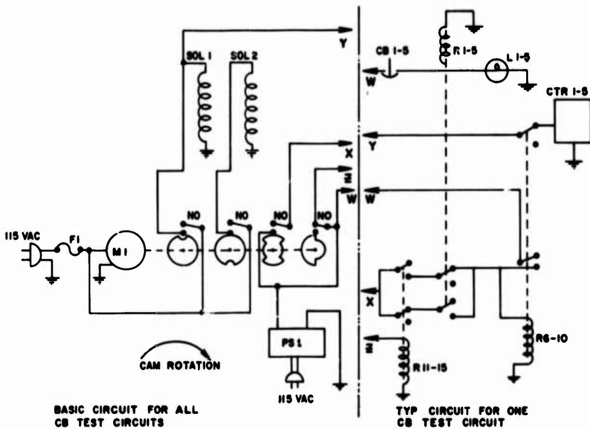
Figure 5. Electrical Schematic.
