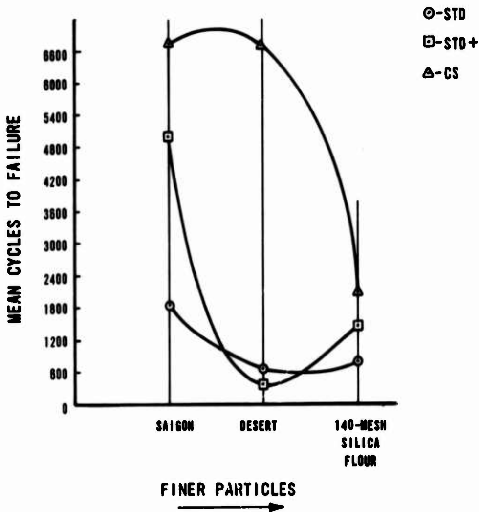
Figure 19. Mean Cycles to Failure Versus Sand Samples.
