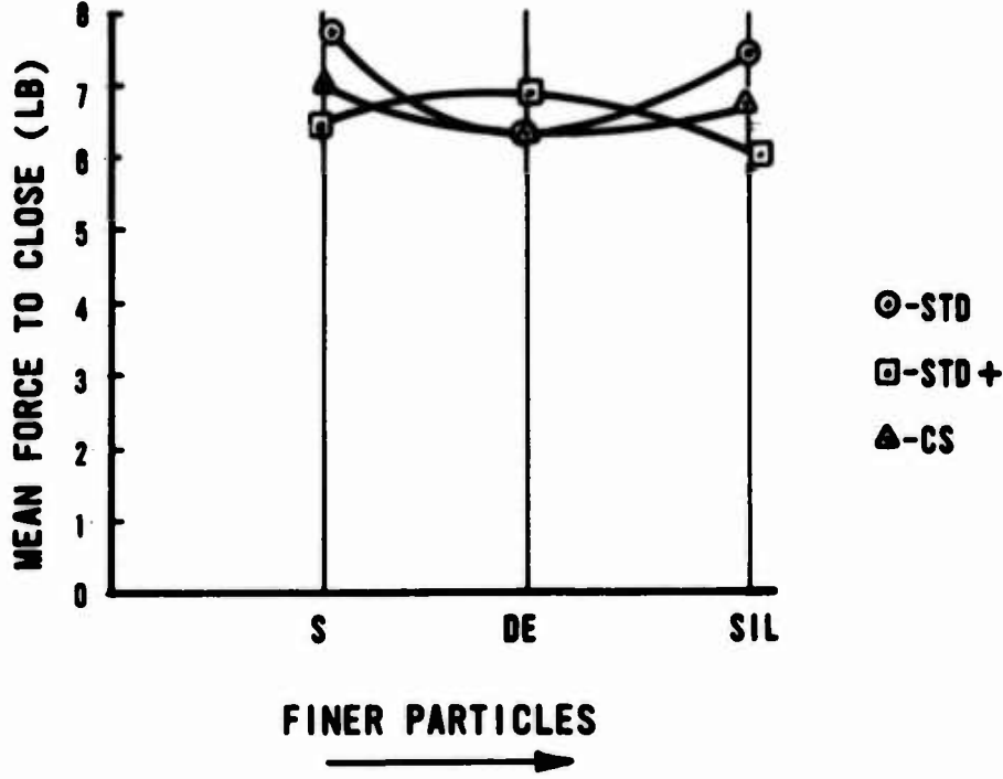
Figure 21. Mean Force To Close Versus Sand Samples.
