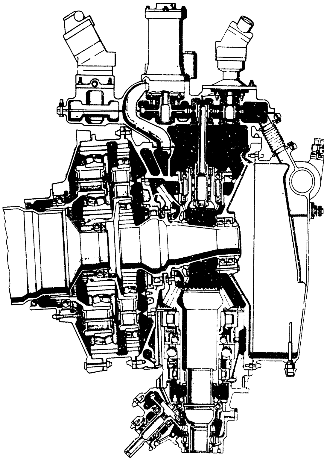
Figure 32. Cih-47C Aft Transmission Cross Section.
