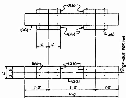
56-WOOD BEAM 4 -IB1
