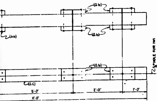
6-WOOD TIE BEAM- B2
