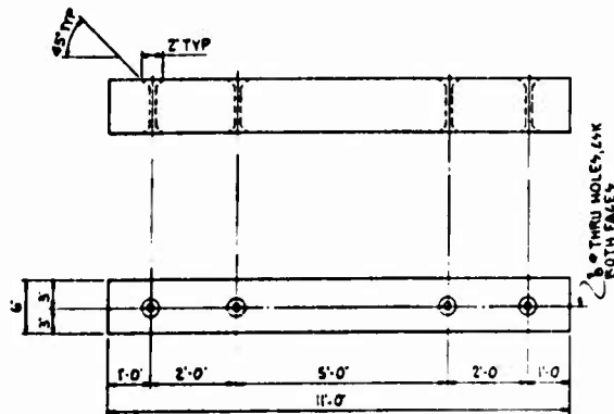
4-WOOD END BEAM 4 -IB3
