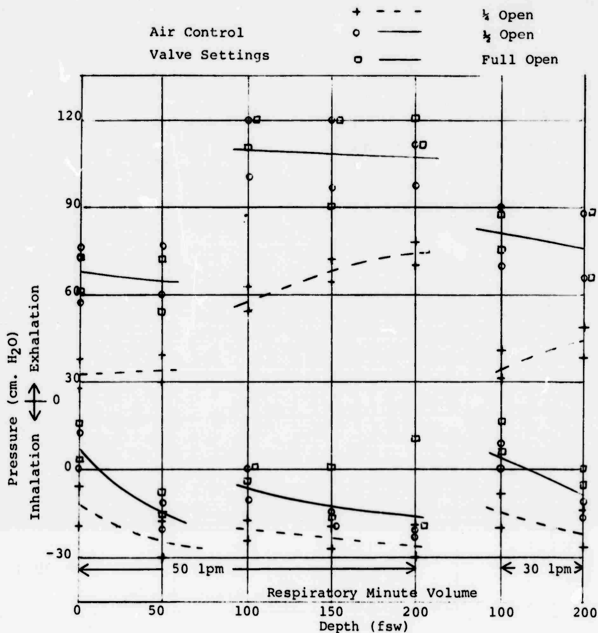
Figure 10 Peak Helmet Pressures on Inhalation and Exhalation Relative to the Suprasternal Notch Level of the Test Manikin (20 cm below mouth level)
