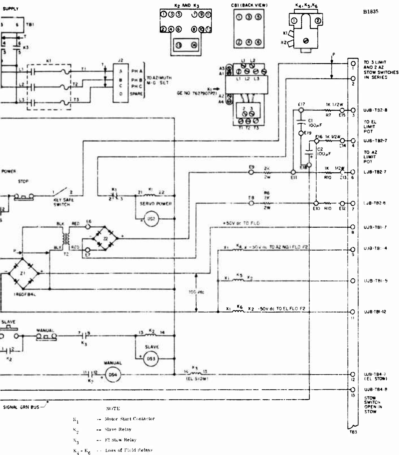
Figure 37. Antenna Positioning Control Circuitry
