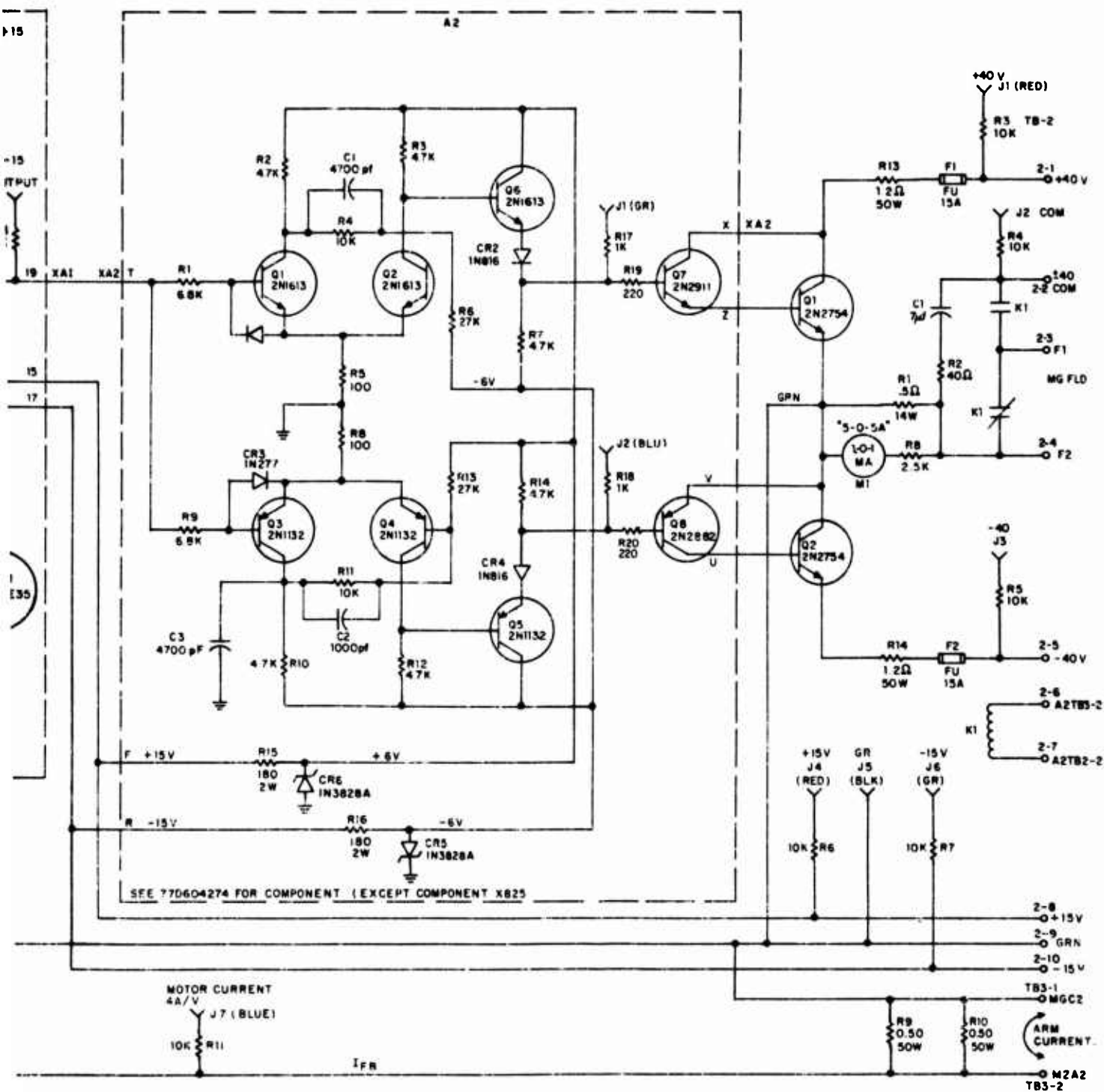
Figure 34. Azimuth Servo
