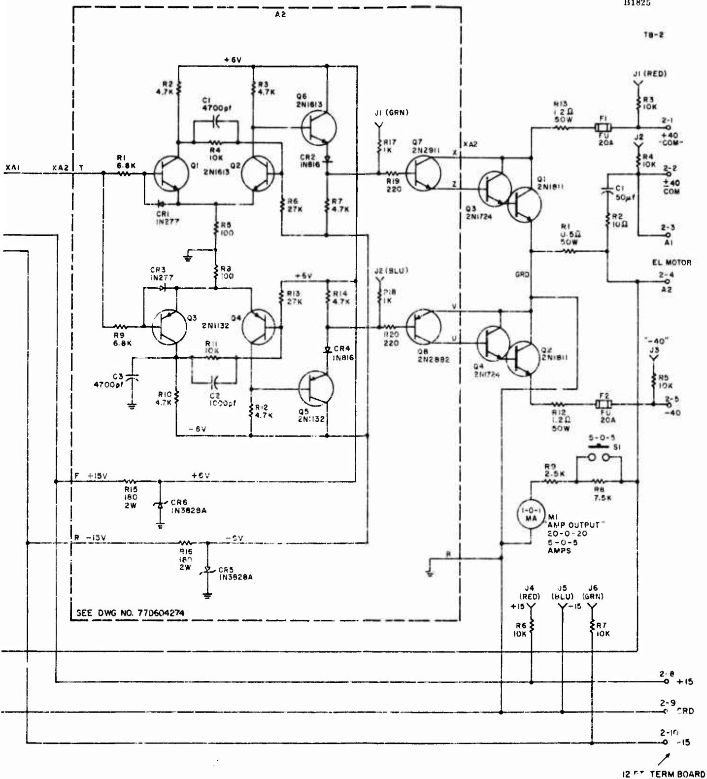
Figure 33. Elevation Servo Amplifier
