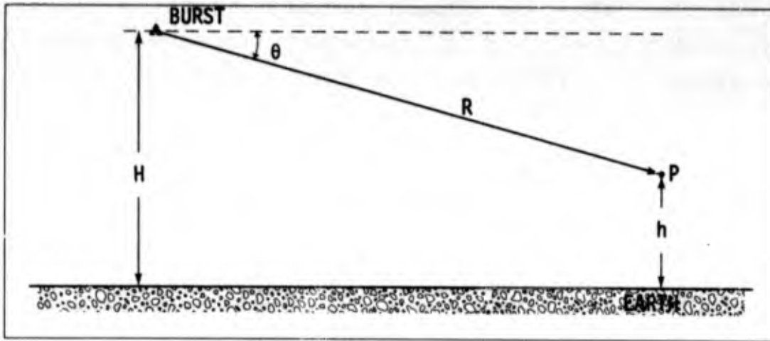
Figure 1. Assumed geometry of problem.
