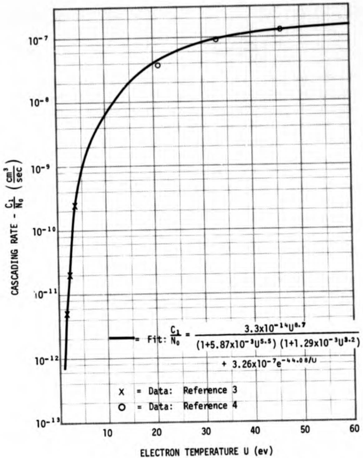
Figure 3. Cascading rate, C_1 , as a function of temperature U .
