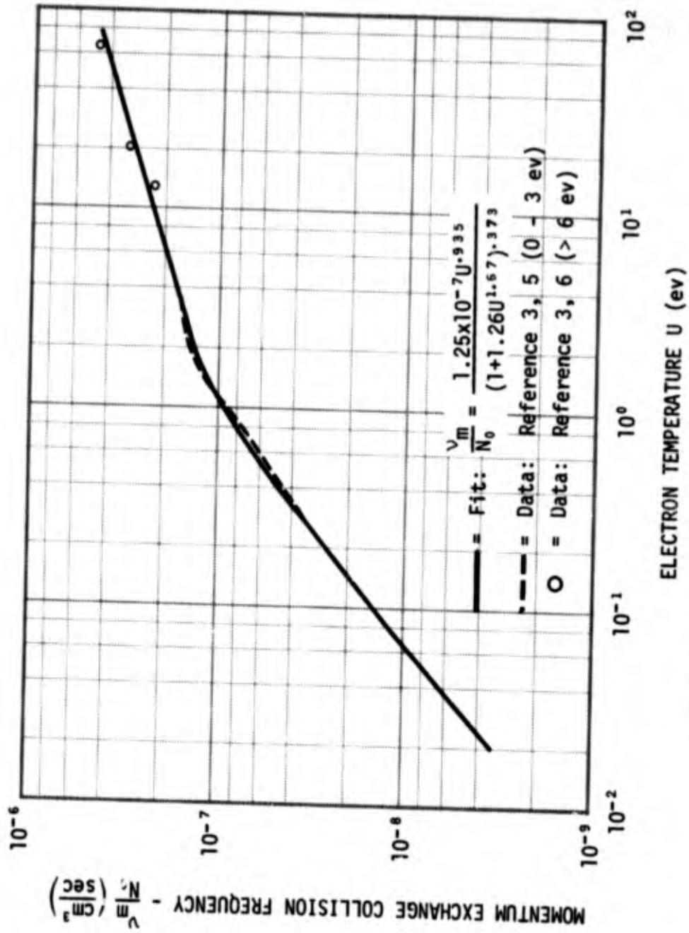
Figure 5. Momentum exchange collision frequency, \nu_m , as a function of U.
