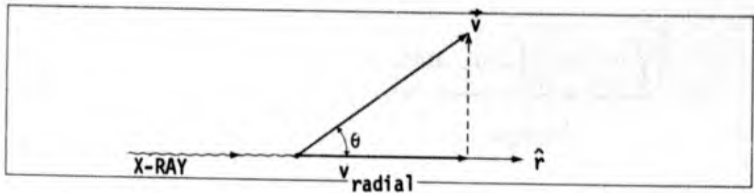
Figure 2. Electron production geometry.
