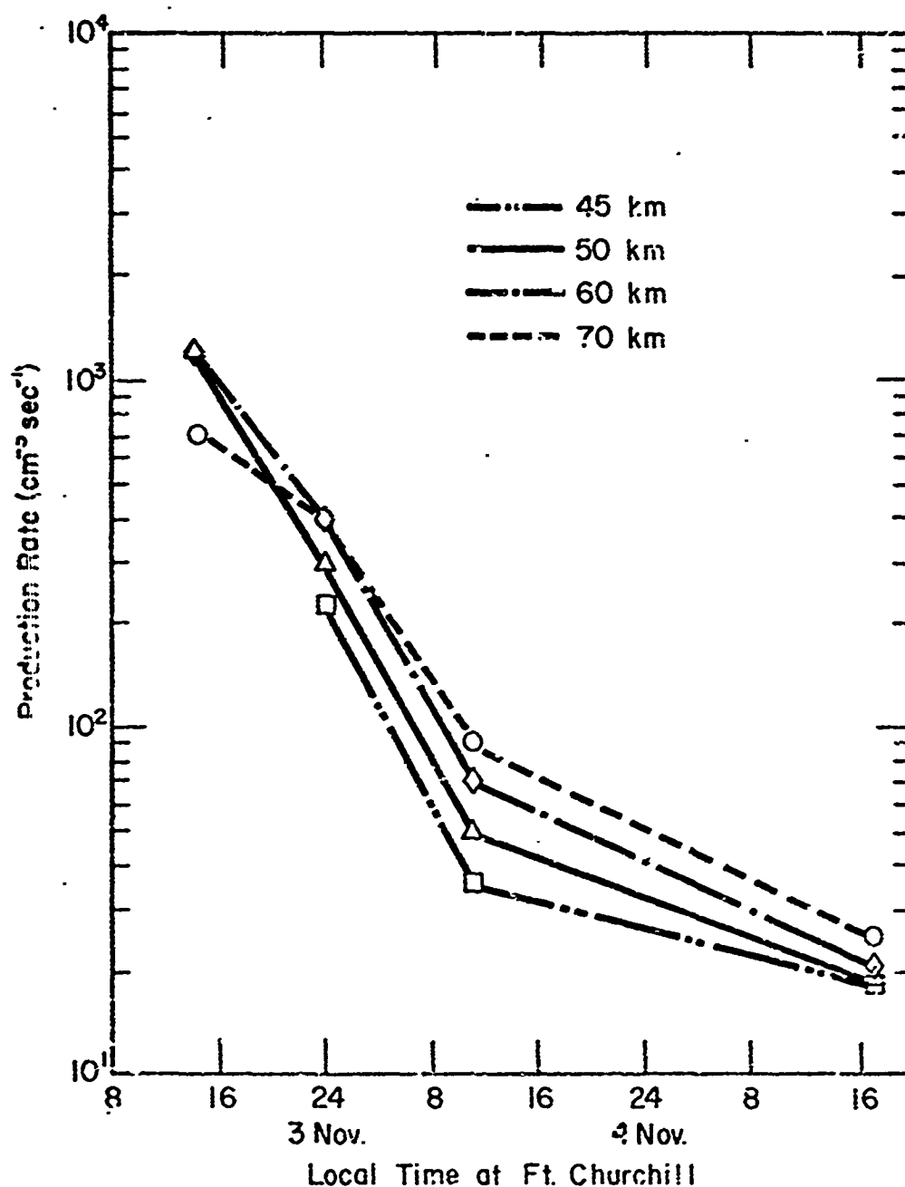
Fig. 4-2. Production rates during the November 2, 1969 PCA from extrapolation of the preliminary rates of Swider and Gardner (1972).
