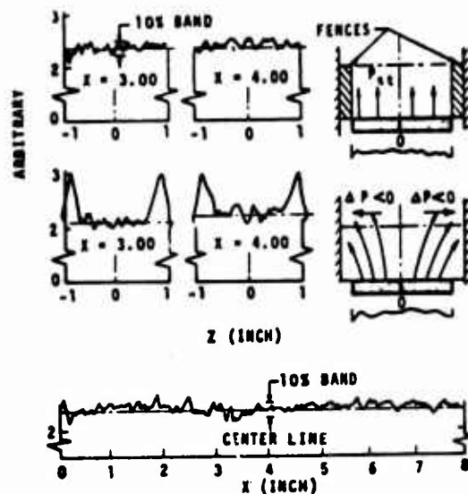
Figure 2. Flow Uniformity Through Porous Plate
