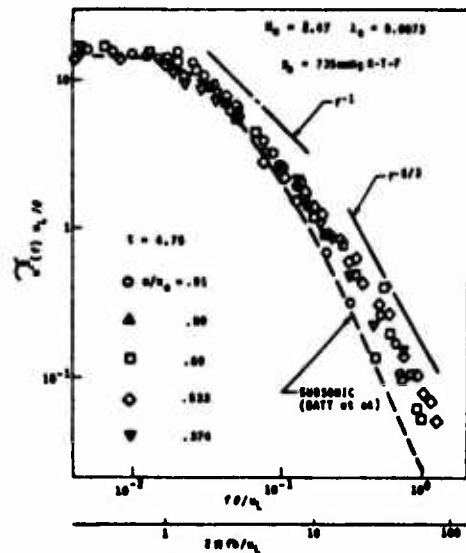
Figure 9. Comparison of Supersonic and Incompressible Streamwise Velocity Fluctuation Spectra
