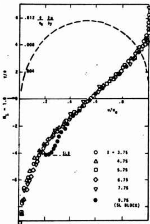
Figure 3. TFML Velocity and Velocity Gradient Profiles
