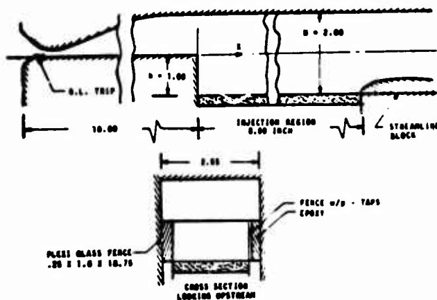
Figure 1. Test Section Configuration
