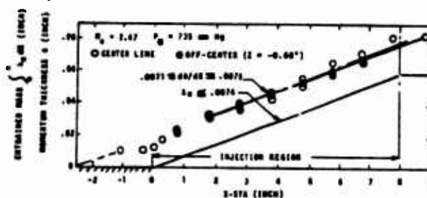
Figure 5. TFML-Comparison of Momentum Thickness Distribution vs. Entrained Mass Distribution
