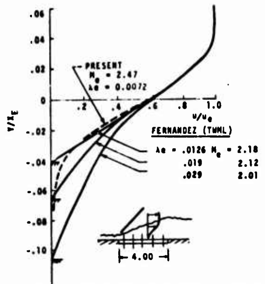
Figure 7. Comparison of Velocity Profiles with Variable Mass Injection Rates Through Flat Plate Model.
