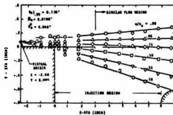
Figure 4. TFML Longitudinal Velocity Distributions
