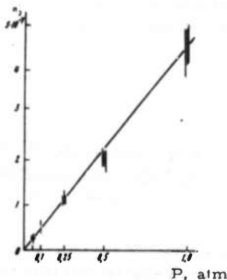
Fig. 1. Relationship of refractive index n_2 in \text{BCl}_3 to gas pressure.
