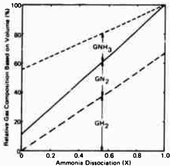
Figure 3. The effect of ammonia dissociation on the decomposition products of hydrazine.
