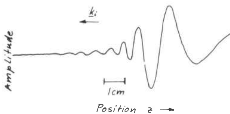
Figure 6. Double pump ion oscillations.
