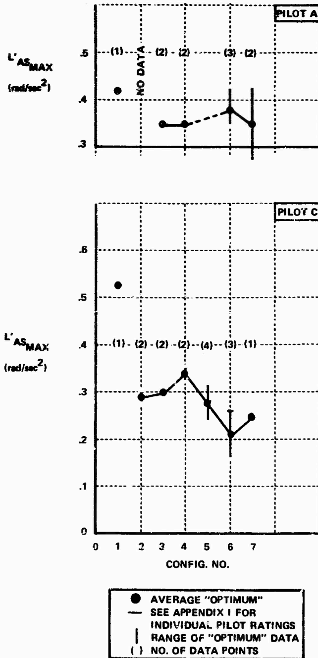
Figure 5-7 VARIATION OF L'AS_{MAX} WITH "OPTIMUM" CONFIGURATIONS FOR ILS TRACKING IN NEGLIGIBLE TURBULENCE (PILOTS A AND C)
