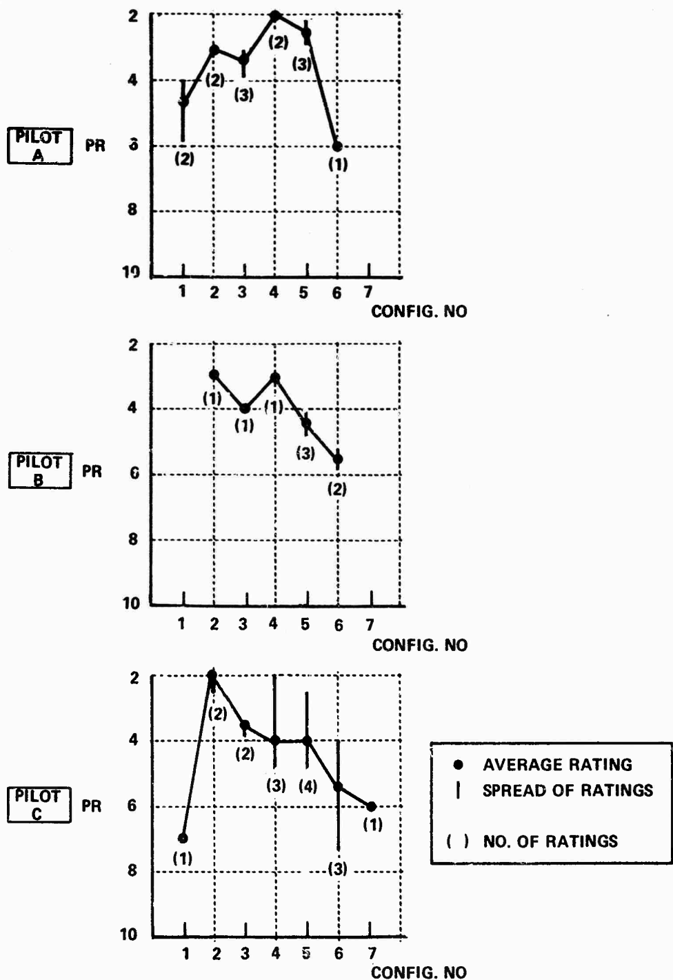
Figure 4-6 SUMMARY OF INDIVIDUAL PILOT RATINGS FOR "OPTIMUM" CONFIGURATIONS, UNLIMITED LATERAL CONTROL POWER
