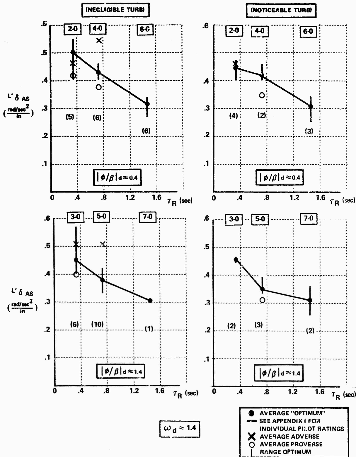
Figure 4-5 EFFECT OF \tau_R ON LATERAL CONTROL SENSITIVITY
