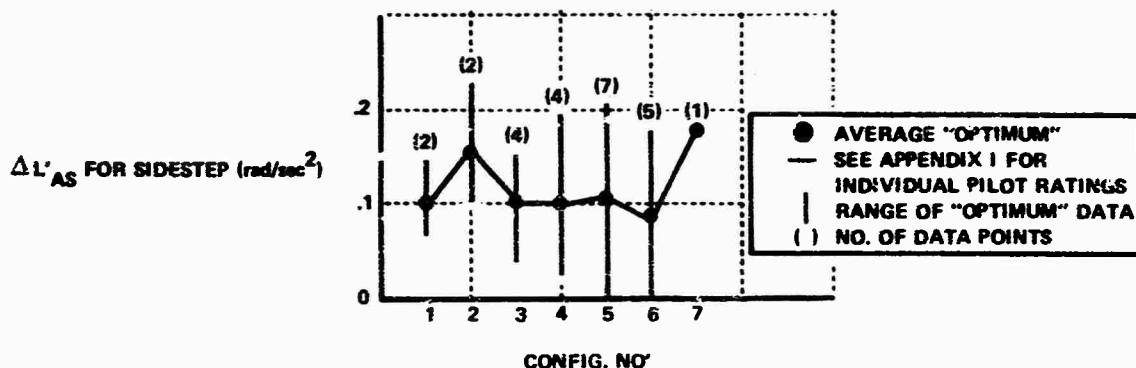
Figure 5-5 \Delta L'_{AS} REQUIRED FOR SIDESTEP MANEUVER IN NEGLIGIBLE TURBULENCE ("OPTIMUM" CONFIGURATIONS)
