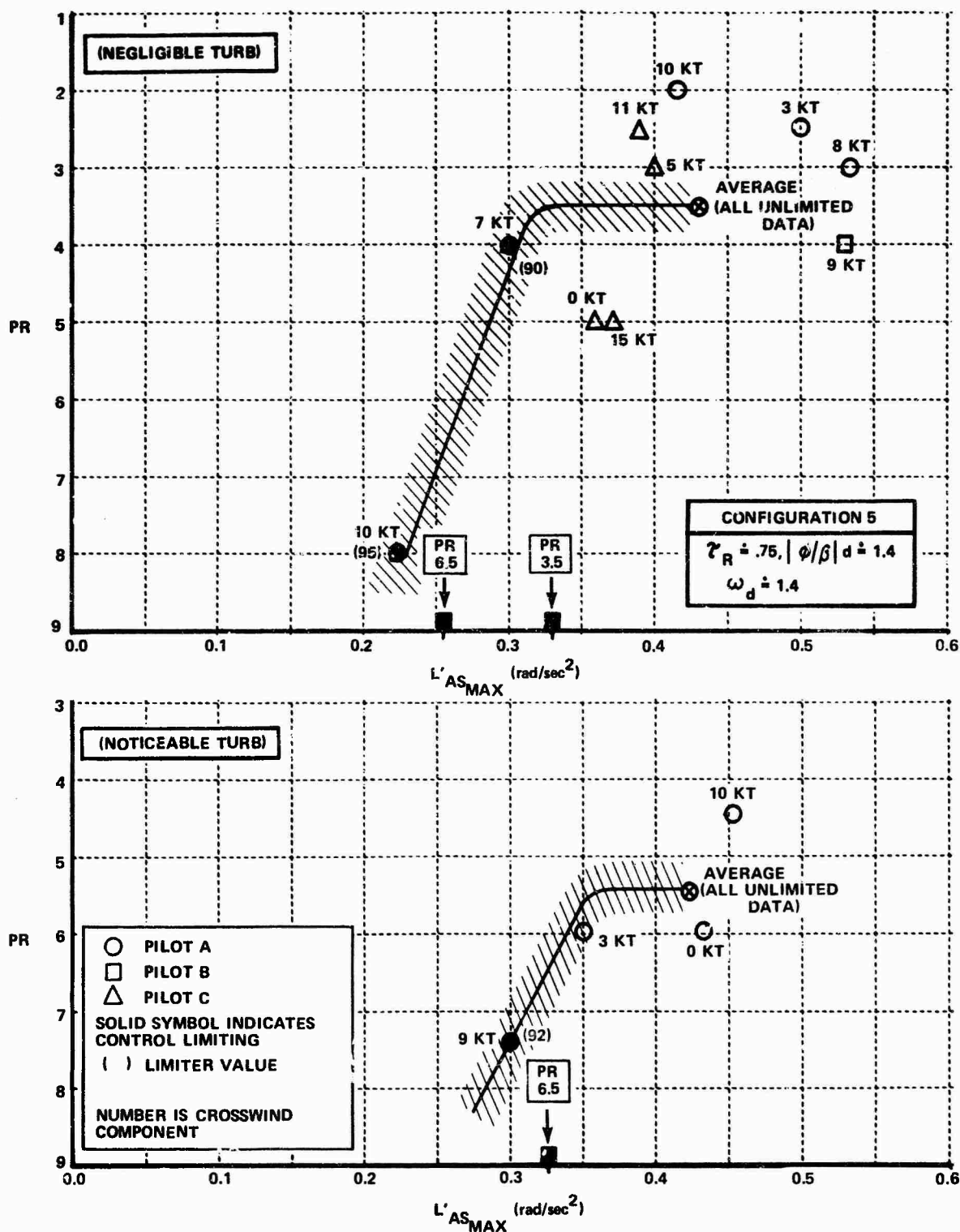
Figure 5-11 PILOT RATING VS MAXIMUM ROLL CONTROL USED (CONFIGURATION 5)
