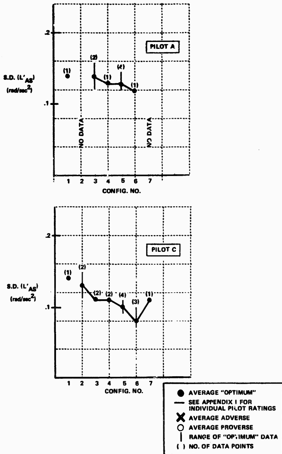
Figure 5-4: VARIATION OF S.D. OF L'_{AS} WITH "OPTIMUM" CONFIGURATIONS FOR TOTAL APPROACH IN NEGLIGIBLE TURBULENCE (PILOTS A AND C)
