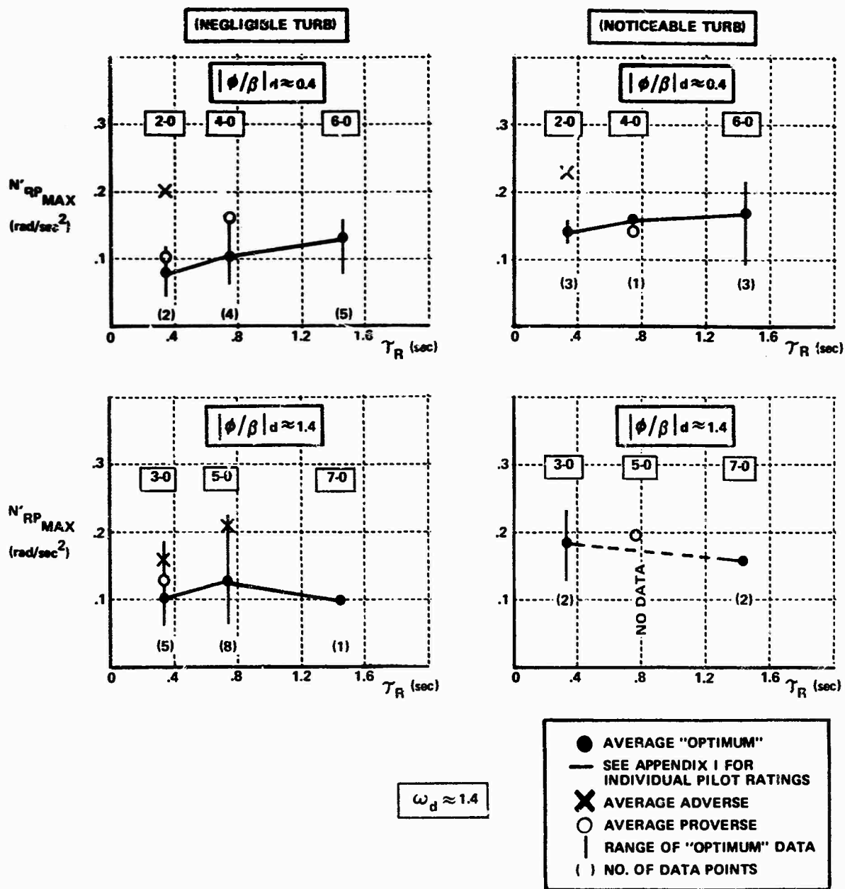
Figure 5-8 EFFECT OF T_R ON N'_{RP \text{ MAX}} FOR TOTAL APPROACH (TURBULENCE EFFECTS SEPARATED)
