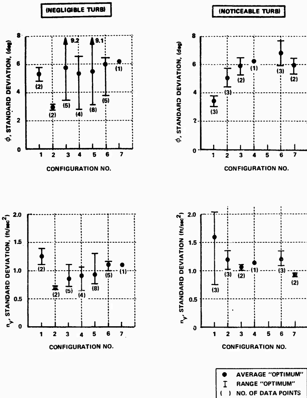
Figure 6-2 STANDARD DEVIATIONS OF \phi AND n_y IN ILS TRACKING FOR ALL "OPTIMUM" UNLIMITED CONFIGURATIONS
