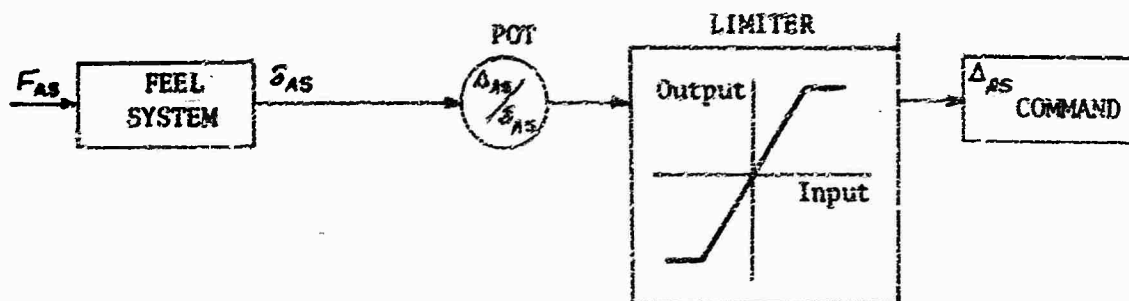
Figure 2-1 Aileron Limiter Schematic
