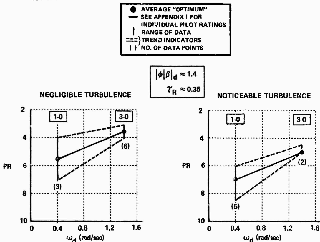
Figure 4-2a EFFECT OF \omega_d ON PILOT RATING (TURBULENCE EFFECTS SEPARATED)
