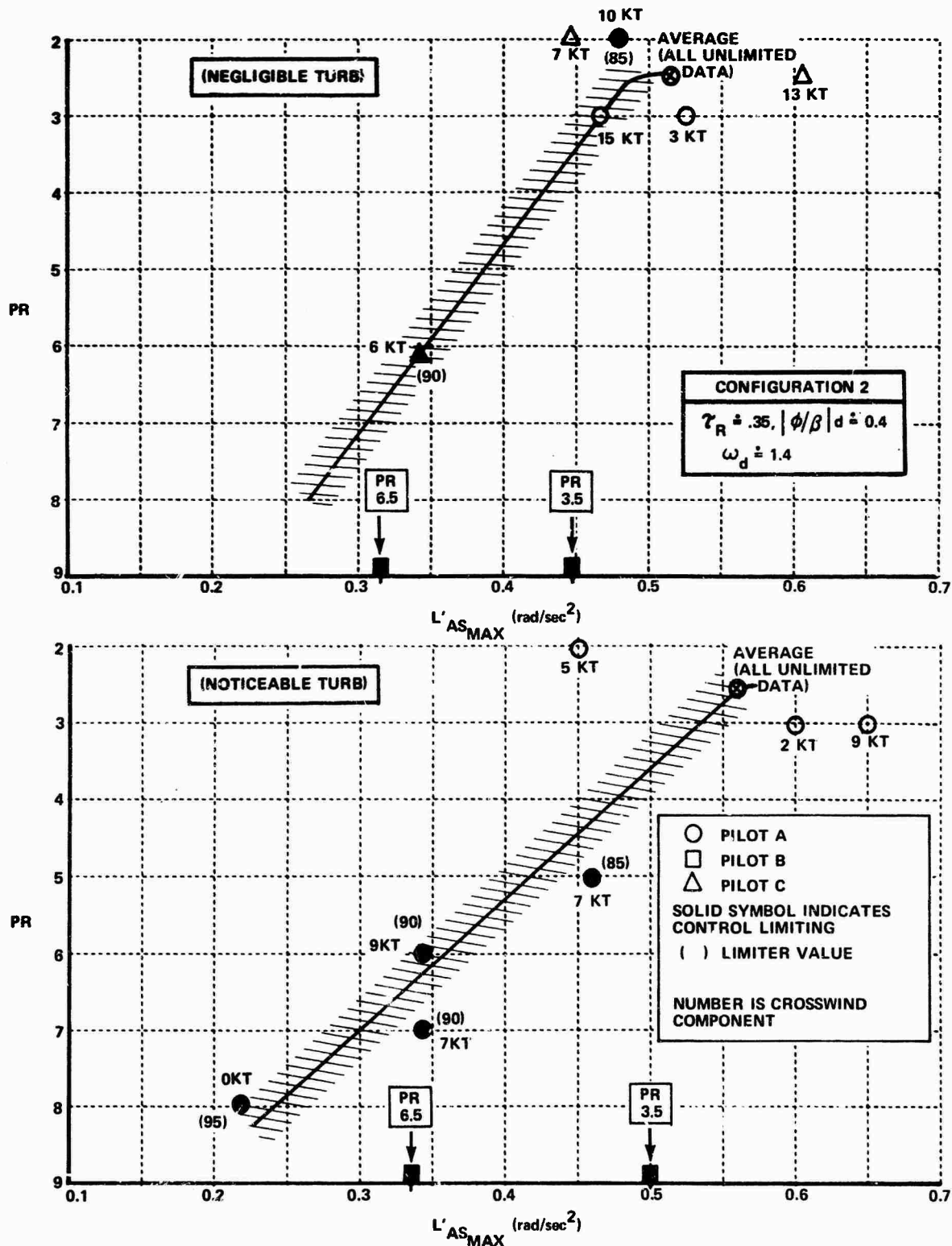
Figure 5-9 PILOT RATING VS MAXIMUM ROLL CONTROL POWER USED (CONFIGURATION 2)
