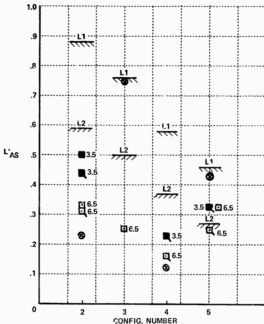
Figure 7-4 MIL-F-83300 MINIMUM LEVEL 1 AND LEVEL 2 ROLL CONTROL POWER REQUIREMENTS AGAINST PR \pm 3.5 and PR \pm 6.5 CONTROL POWERS OF EXPERIMENT
