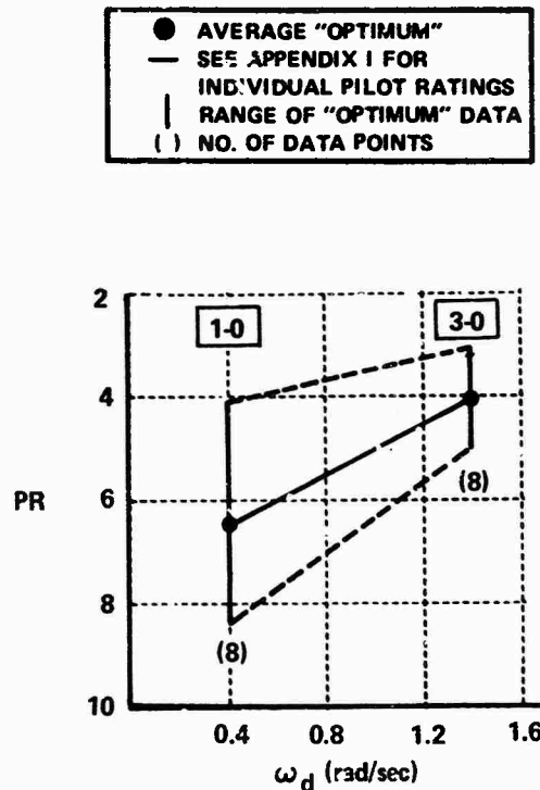
Figure 4-2b EFFECT OF \omega_d ON PILOT RATING (ALL EVALUATIONS)
