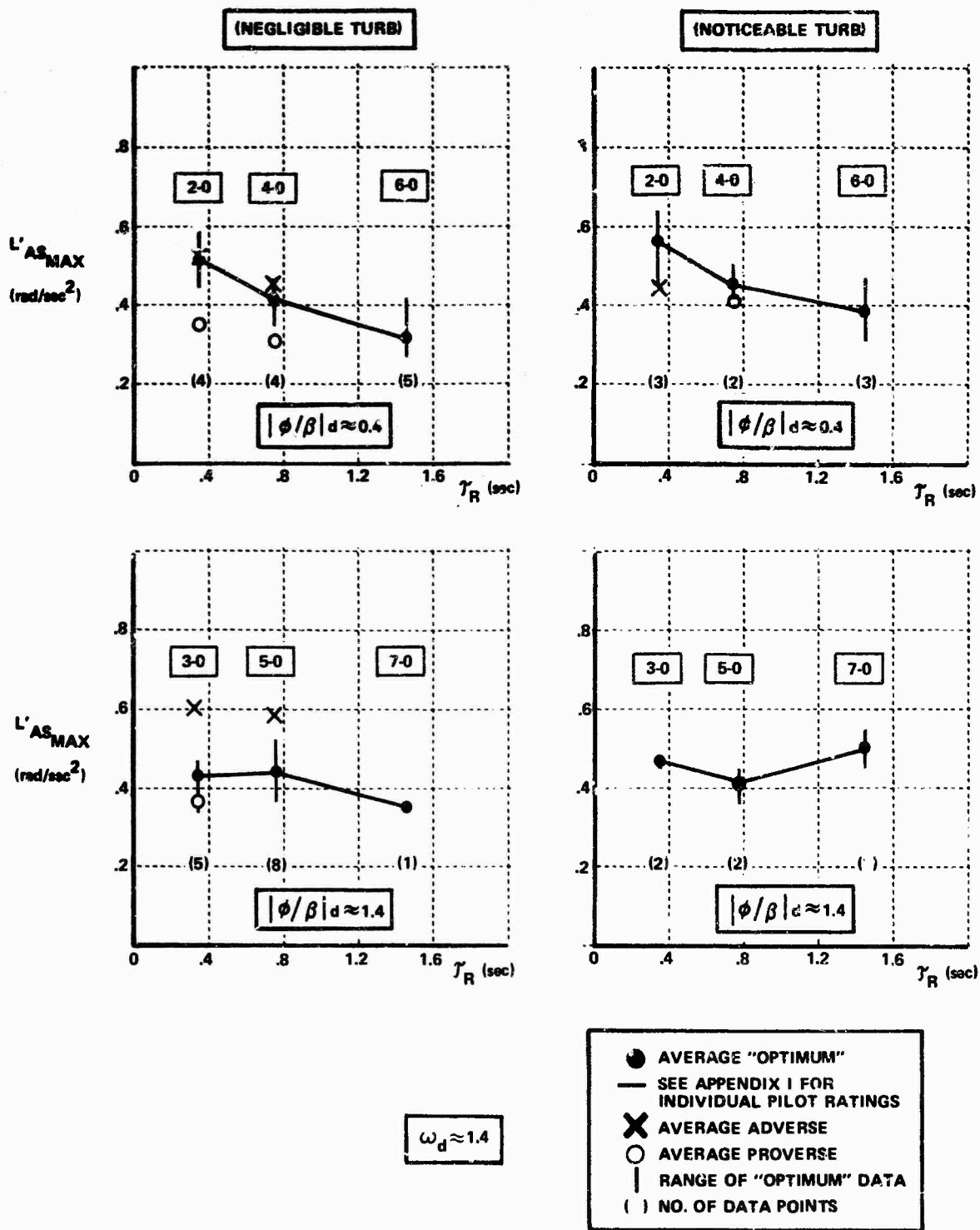
Figure 5-1 EFFECT OF T_R ON L'_{AS_{MAX}} FOR TOTAL APPROACH (TURBULENCE EFFECTS SEPARATED)
