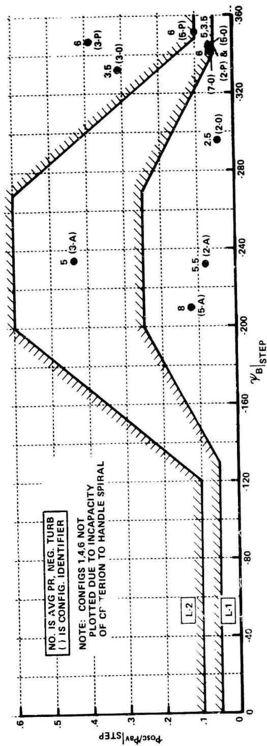
Figure 7-6 COMPARISON OF EVALUATION CONFIGURATIONS WITH P_{osc}/P_{av} REQUIREMENT OF MIL-F-8785B (REF. 3), NEG. TURBULENCE
