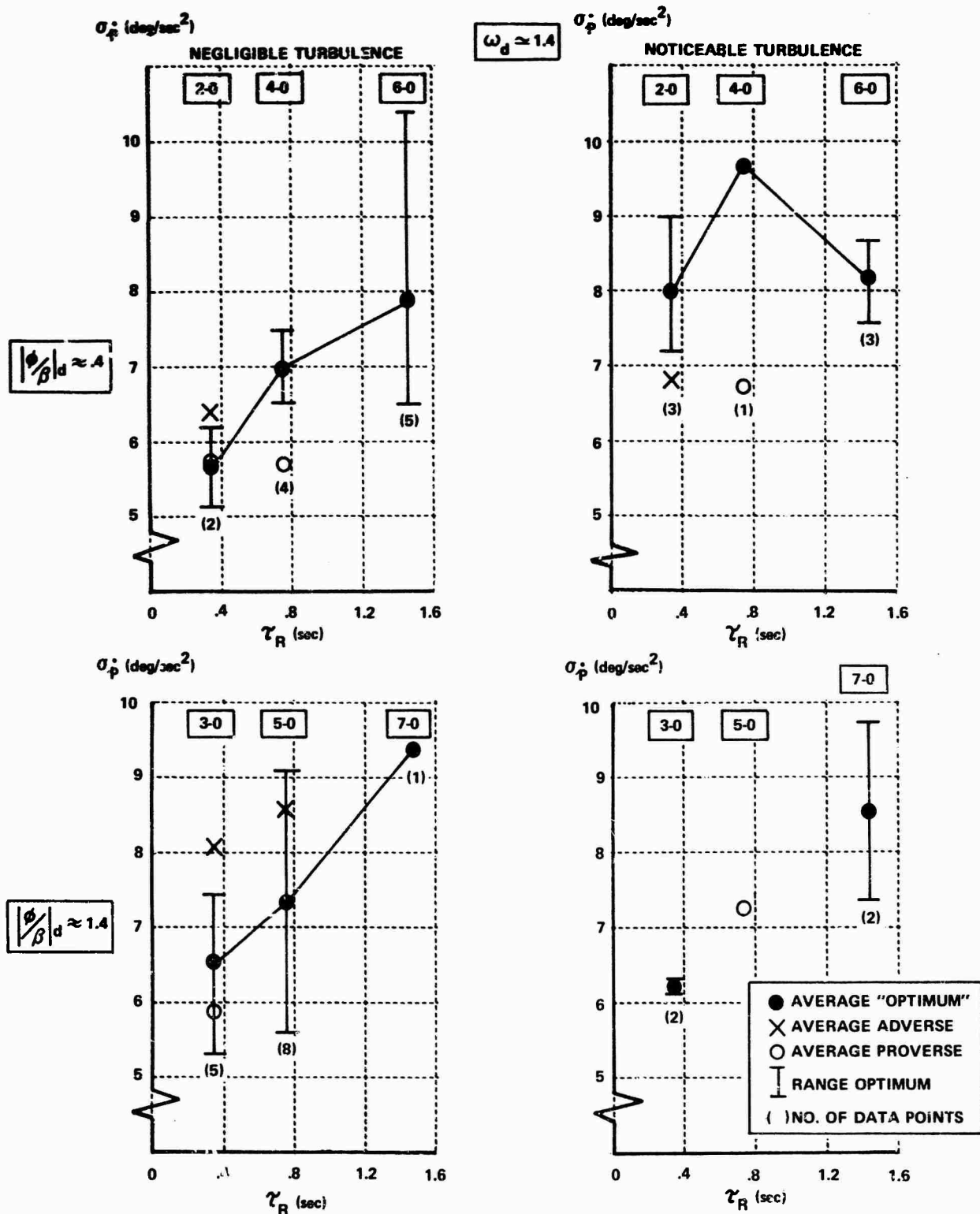
Figure 6-5 EFFECT OF MODAL CHARACTERISTICS AND TURBULENCE ON THE STANDARD DEVIATION OF \dot{\phi} IN ILS TRACKING TASK
