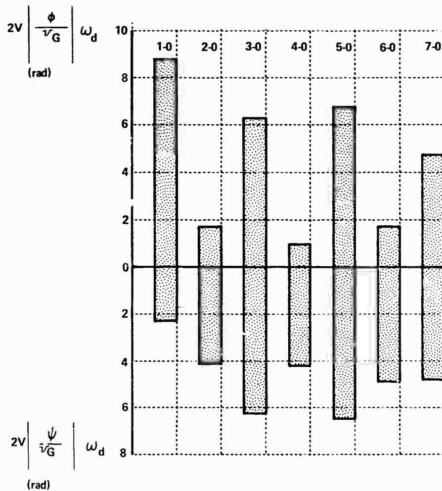
Figure 7-2 RELATIVE ROLL AND YAW ATTITUDE RESPONSE TO LATERAL GUSTS FOR THE BASE CONFIGURATIONS
