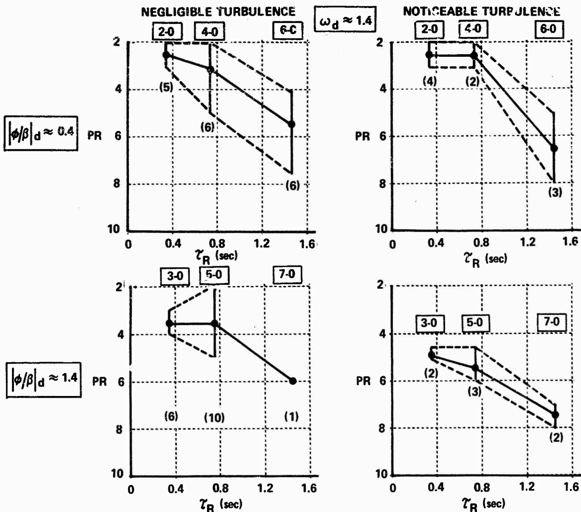
Figure 4-1a EFFECT OF \tau_R ON PILOT RATING (TURBULENCE EFFECTS SEPARATED)
