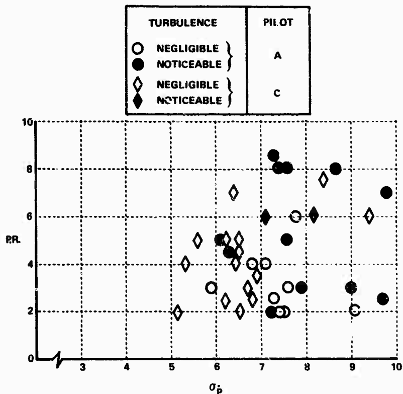
Figure 6-6 STANDARD DEVIATION OF \dot{p} , PILOTS A AND C, ALL OPTIMUM CONFIGURATIONS
