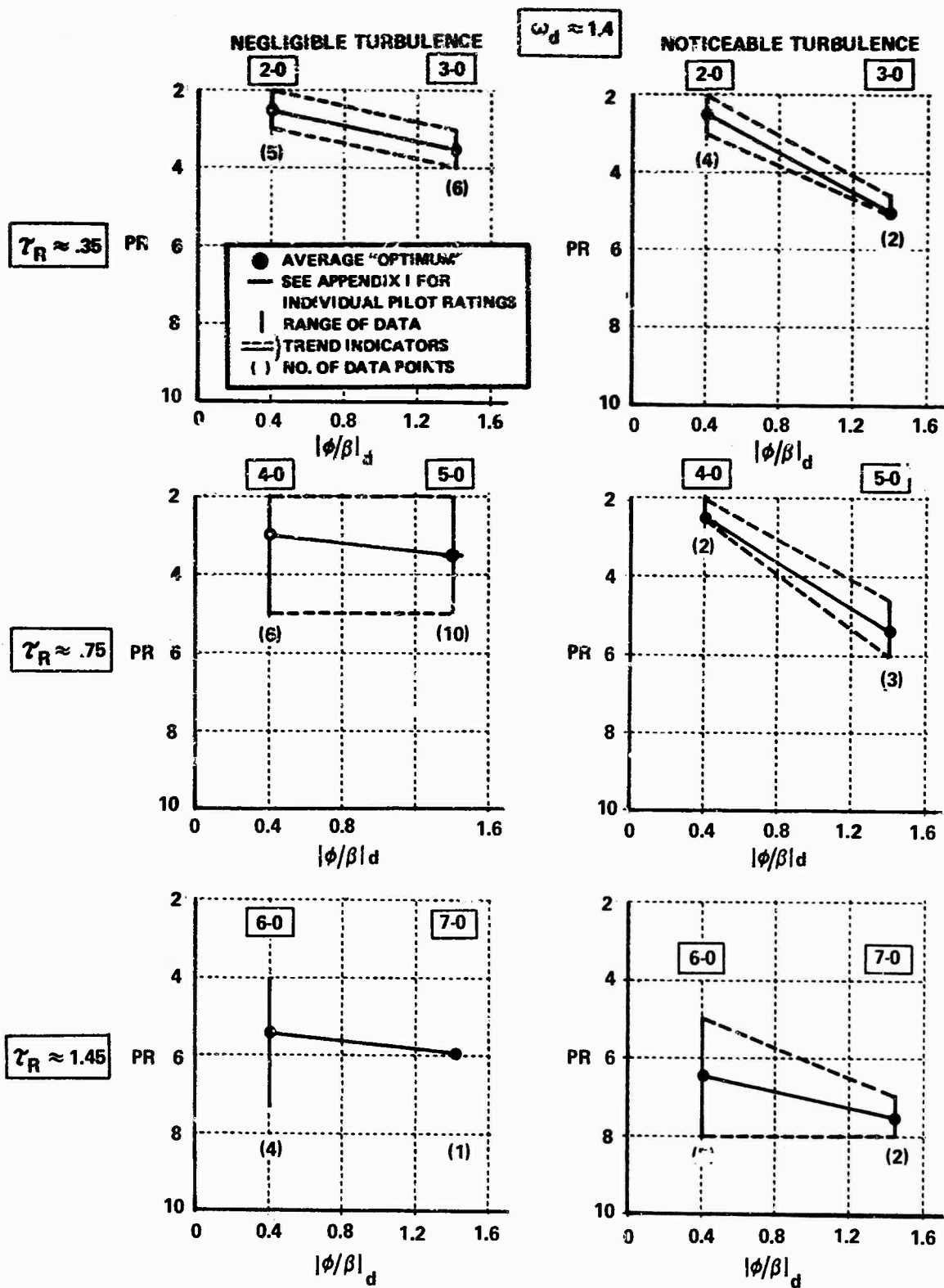
Figure 4-3 EFFECT OF |\phi/\beta|_d ON PILOT RATING (TURBULENCE EFFECTS SEPARATED)
