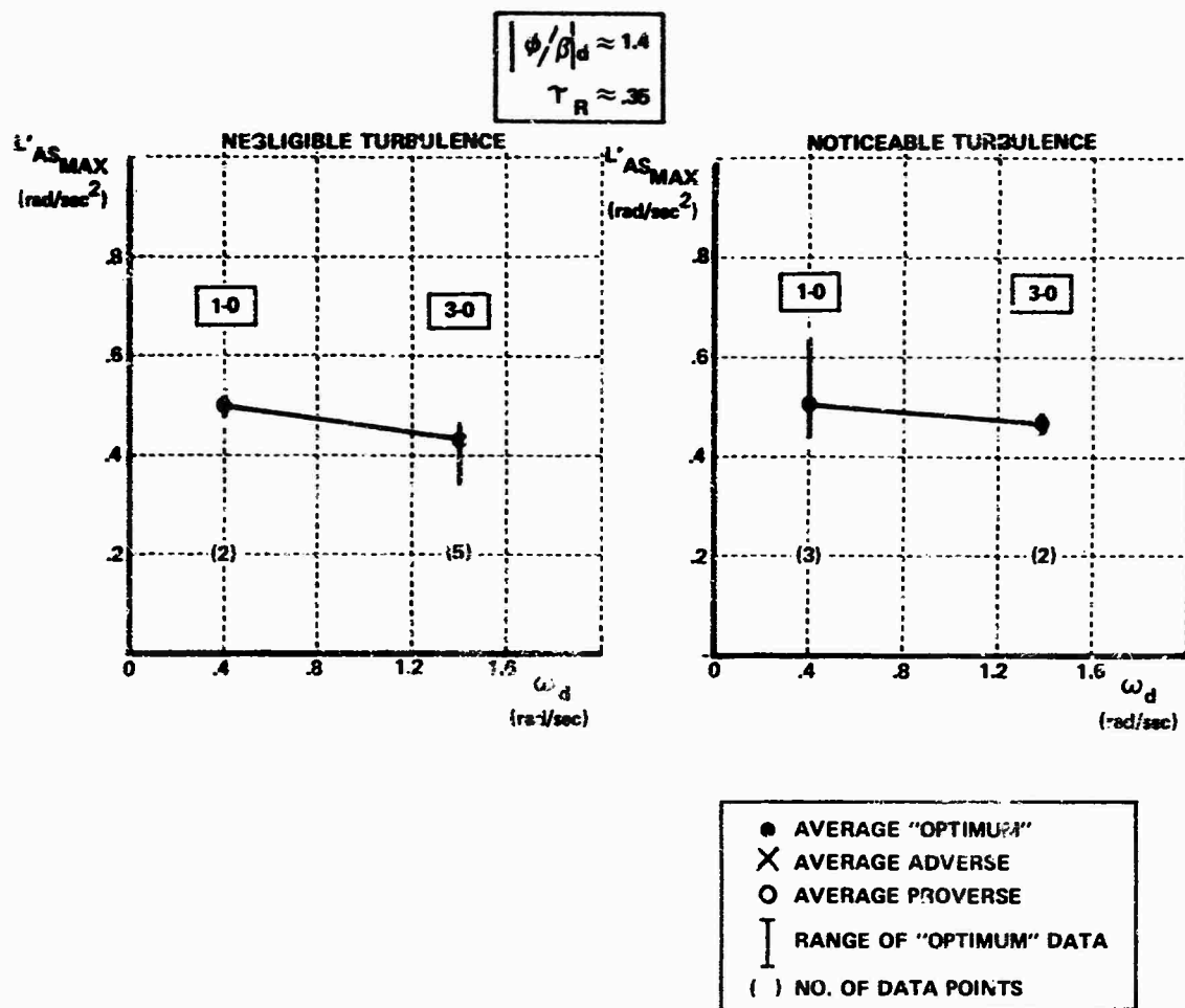
Figure 5-3 EFFECT OF \omega_d ON L'_{AS_{MAX}} FOR TOTAL APPROACH
