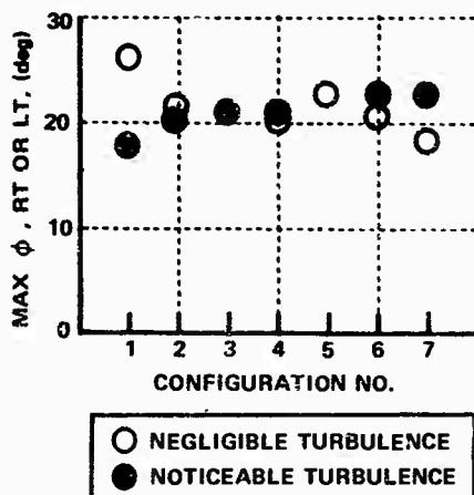
Figure 6-3 MAXIMUM BANK ANGLE FOR TOTAL APPROACH, AVERAGE OF ALL PILOTS
