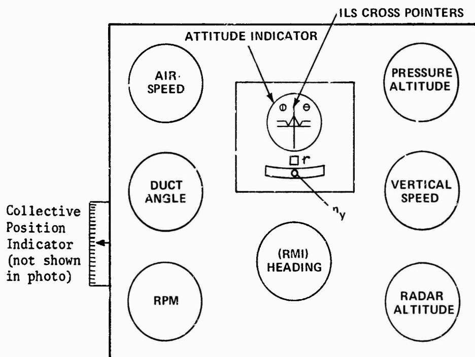
Figure 3-2 EVALUATION PILOT'S INSTRUMENT DISPLAY
