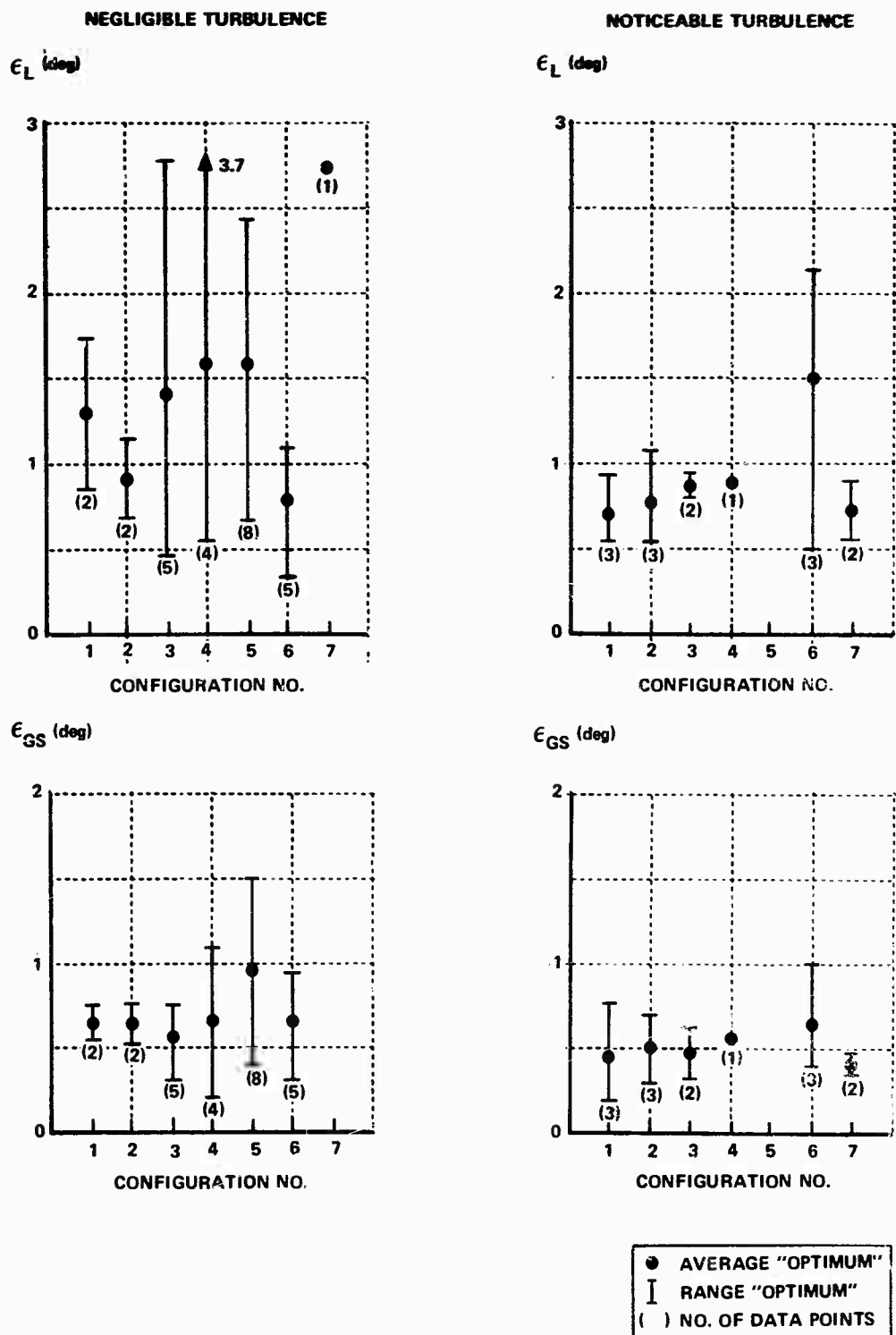
Figure 6-1 RMS DEVIATIONS OF LOCALIZER AND GLIDE SLOPE ILS TRACKING FOR ALL "OPTIMUM" UNLIMITED CONFIGURATIONS
