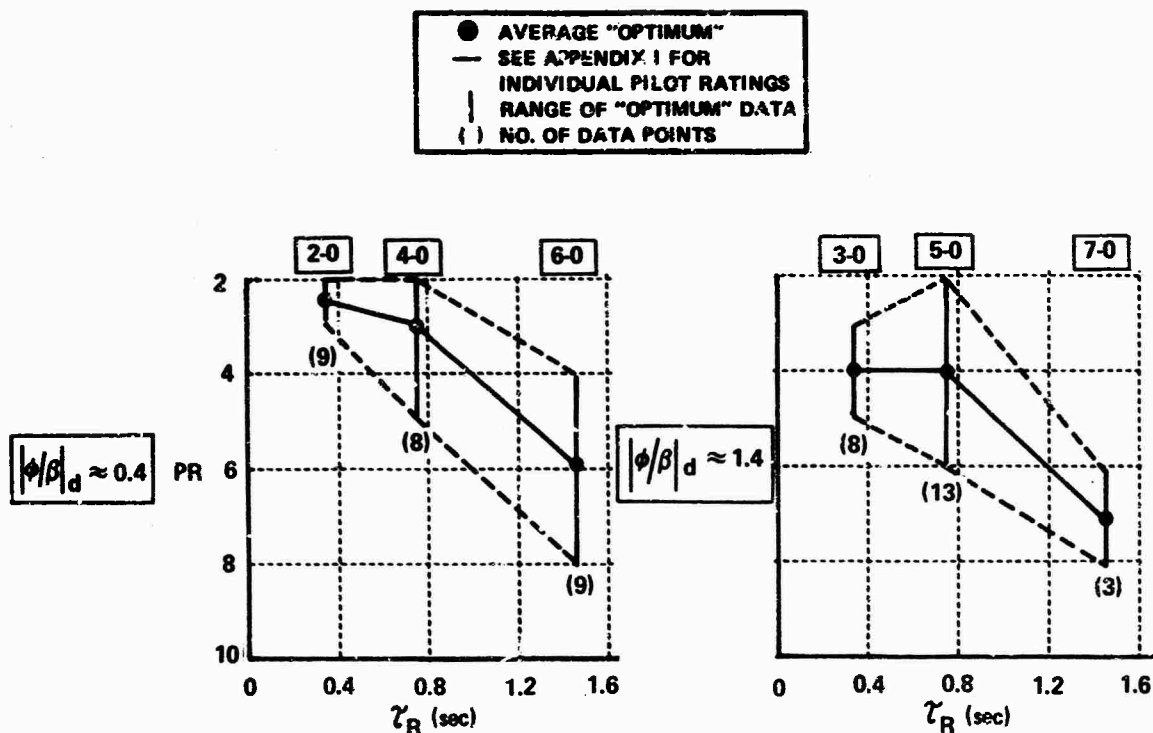
Figure 4-1b EFFECT OF \tau_R ON PILOT RATING (ALL EVALUATIONS)
