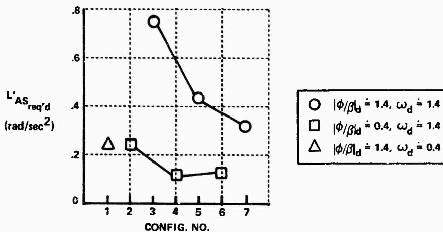
Figure 5-6 ROLL CONTROL POWER REQUIRED FOR "WING-DOWN" RUNWAY TRACKING IN 10 KT CROSSWIND
