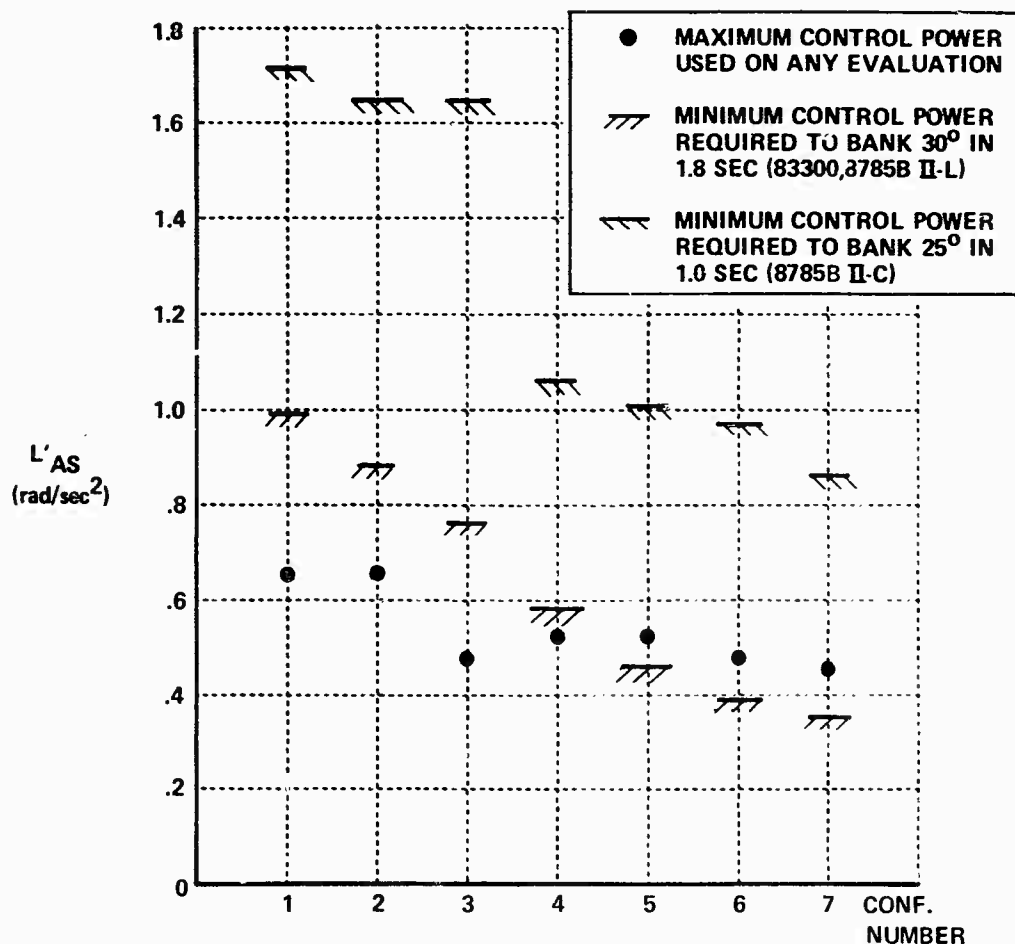
Figure 7-3 MINIMUM LEVEL 1 ROLL CONTROL POWER REQUIREMENTS OF MIL-F-8785B, MIL-F-83300 AGAINST MAXIMUM CONTROL POWER USED
