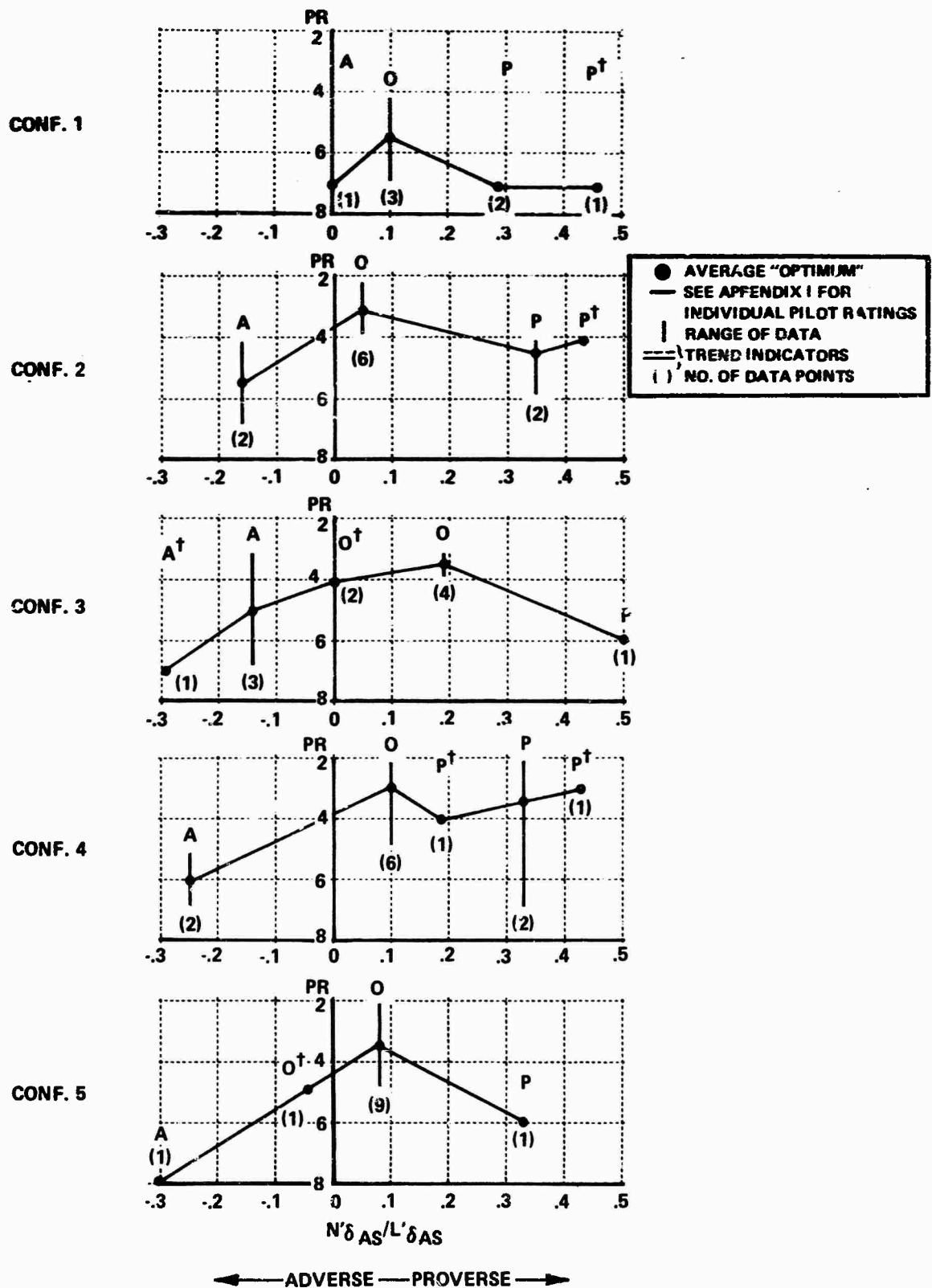
Figure 4-4 EFFECT OF N'\delta_{AS}/L'\delta_{AS} ON PILOT RATINGS (NEGLECTIBLE TURBULENCE)
