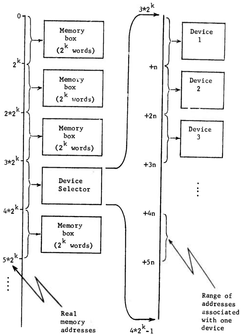
Figure 2-3: Typical memory implementation, showing relation between addresses and physical modules.
