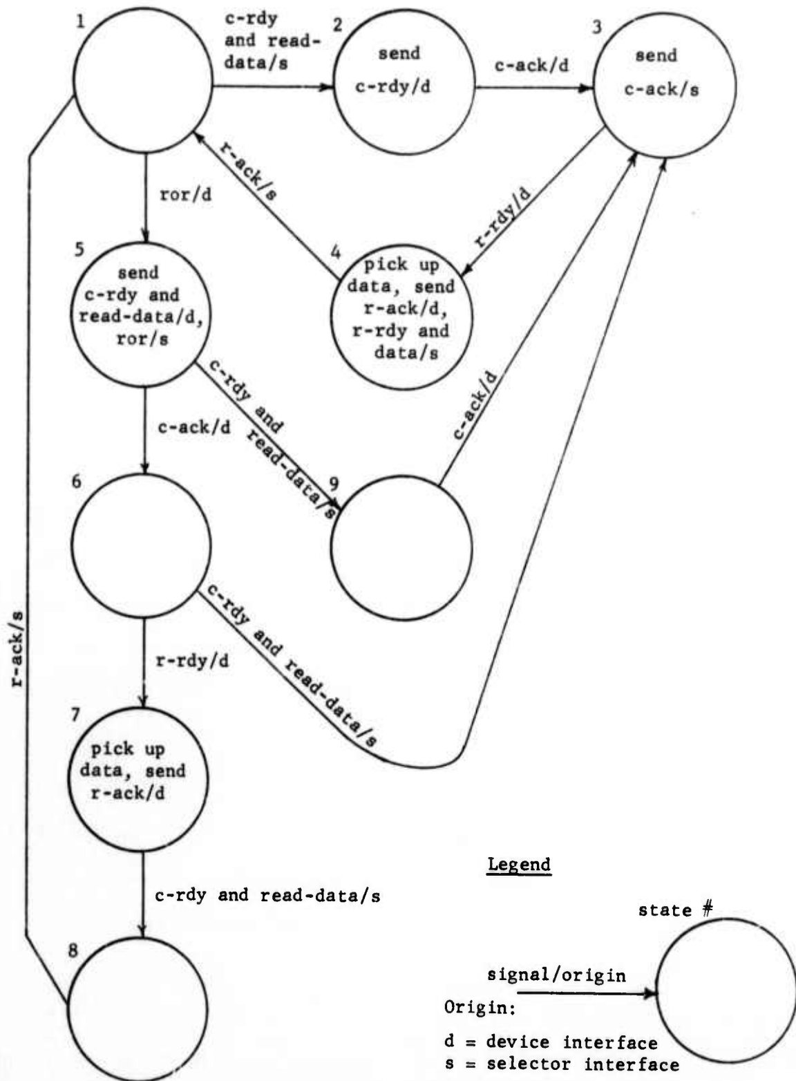
Figure A-1: Read data algorithm for buffer.
