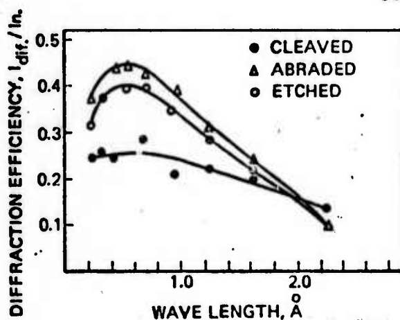
Figure 4b. The intensity ratio, diffracted/incident, at the peak of the diffraction curve for LiF as a function of wavelength and surface treatment.
