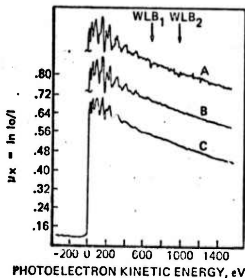
Figure 2. Plots of \ln T/T_0 vs the energy, E , of the ejected photoelectron for \sim 2.5\mu\text{m} thick Cu foil.
