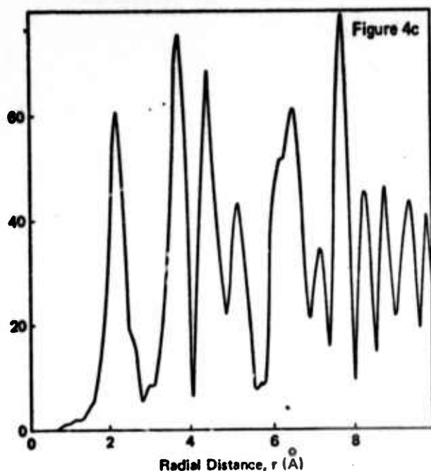
Figures 4a, b and c The real part, imaginary part and magnitude of the FFT for the data of Fig. 2. The vertical scale is proportional to the number of atoms on each coordination shell and has been multiplied by r^2 . The horizontal scale is the radial distance from the absorbing atom in Å.
