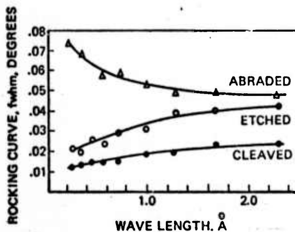
Figure 4a. The full width at half maximum intensity of the rocking curve for LiF crystals as a function of wavelength and surface treatment.
