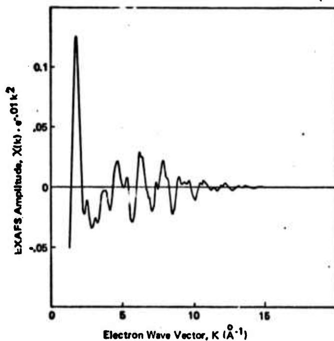
Figure 3 The data of Fig. 2 after a convergence function \exp(-.01K^2) has been applied.
