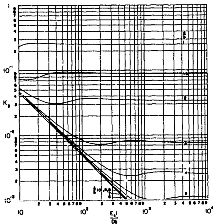
FIGURE 4.12. STRESS PARAMETER AT LOCATION 3 FOR \rho_s A_s / \rho_p b t = 3
