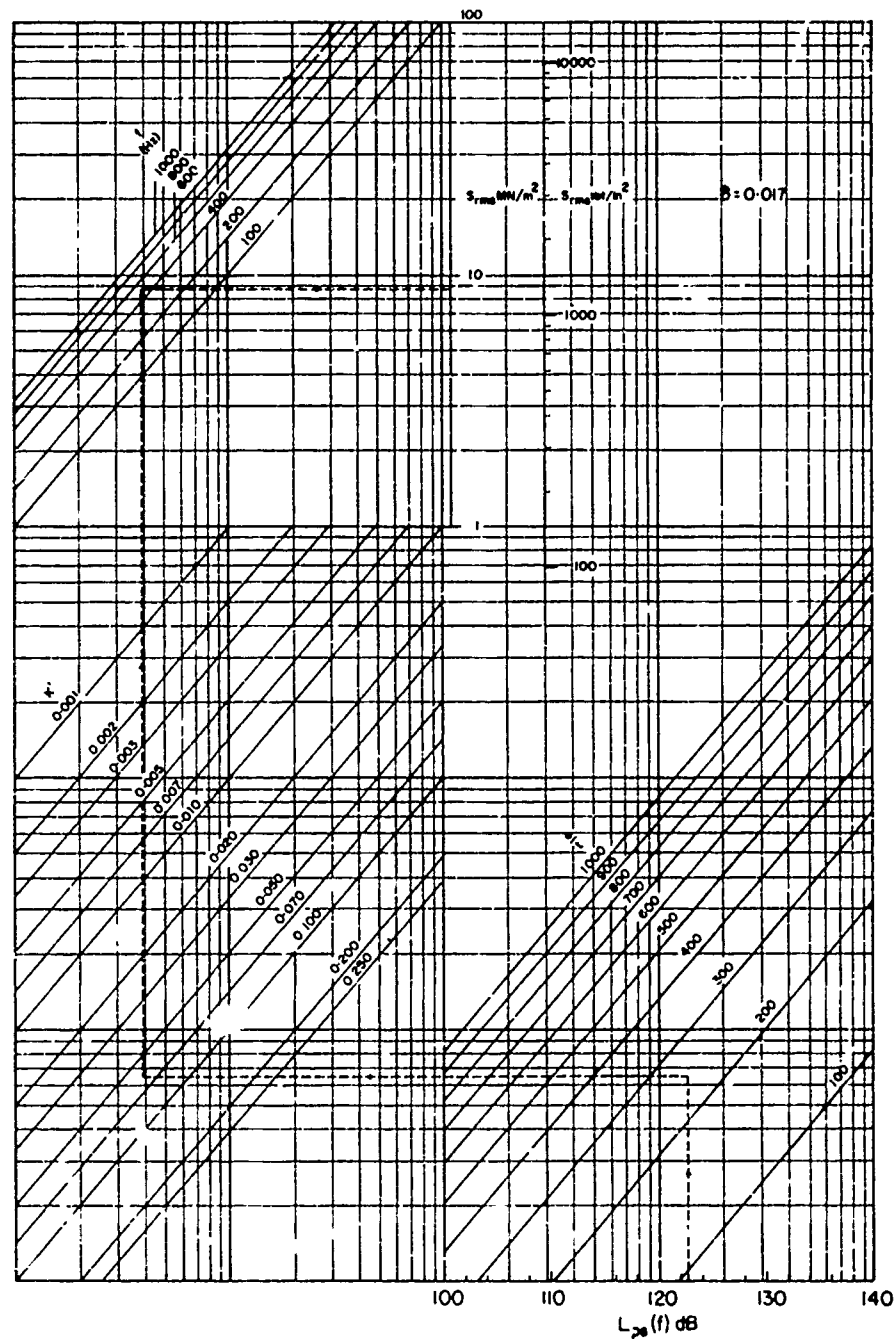
FIGURE 4.25. STRESS NOMOGRAPH
