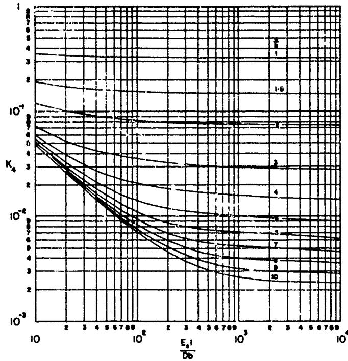
FIGURE 4.13. STRESS PARAMETER AT LOCATION 4 FOR \rho_s A_s / \rho_p b t = 0
