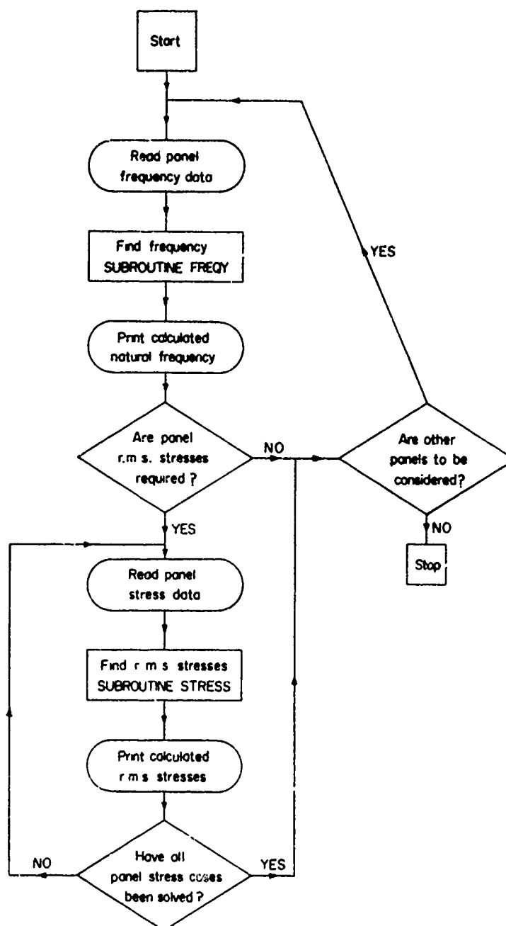
FIGURE 4 A 1 COMPUTER PROGRAM FLOW CHART
