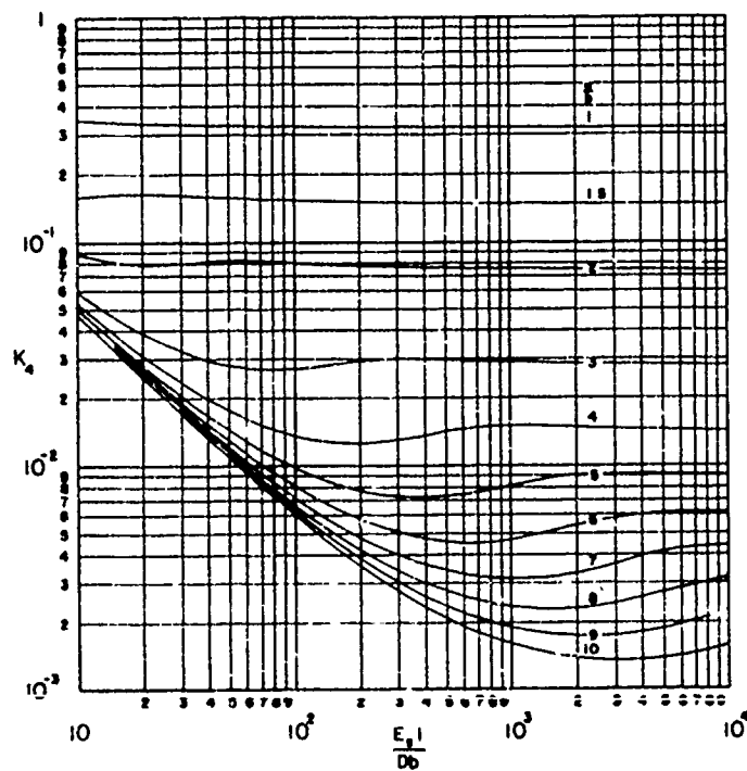
FIGURE 4.14. STRESS PARAMETER AT LOCATION 4 FOR \rho_s A_s / \rho_p b t = 1
