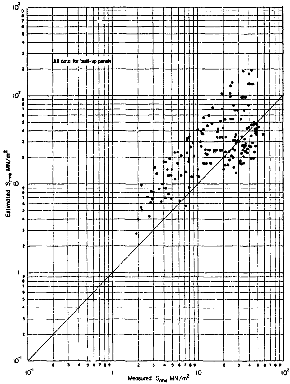
FIGURE 4.29 COMPARISON OF ESTIMATED AND MEASURED STRESS USING MEASURED FREQUENCY AND DAMPING RATIO FOR STRESS ESTIMATION
