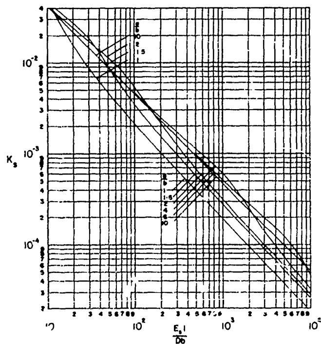
FIGURE 4.24. STRESS PARAMETER AT LOCATION S FOR \rho_s A_s / \rho_p b t = 3
