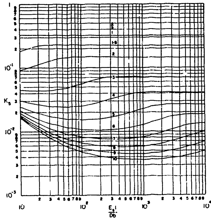
FIGURE 4.18. STRESS PARAMETER AT LOCATION S FOR \rho_s A_s / \rho_p b t = 1
