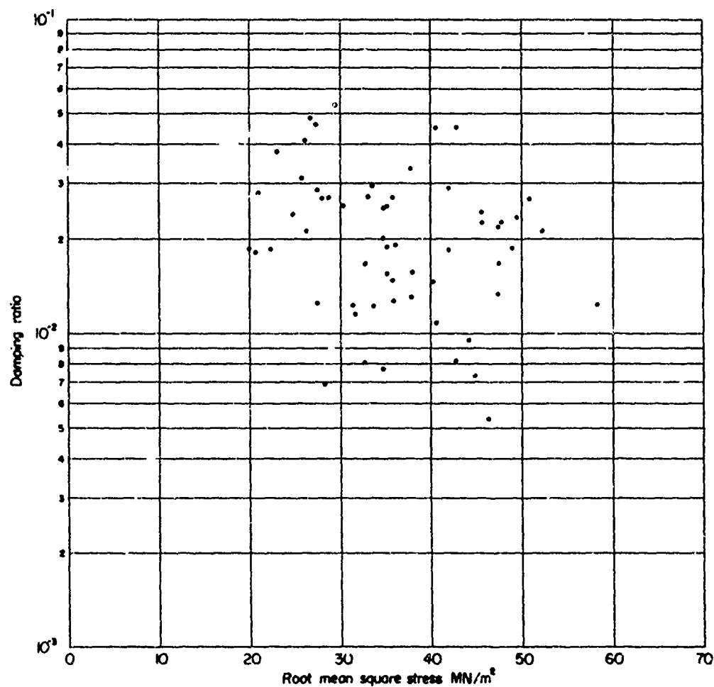
FIGURE 2.5. AMPLITUDE EFFECT ON DAMPING RATIO
