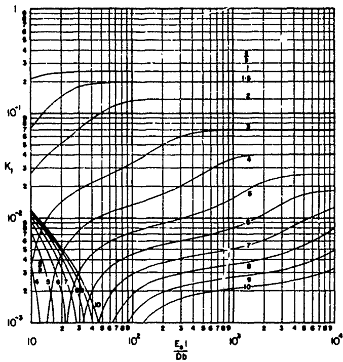
FIGURE 4.3. STRESS PARAMETER AT LOCATION 1 FOR \rho_s A_s / \rho_p b t = 2
