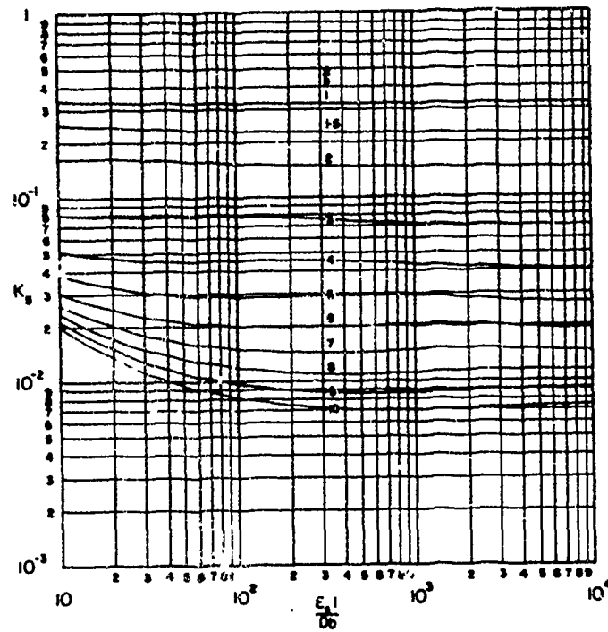
FIGURE 4.17. STRESS PARAMETER AT LOCATION S FOR \rho_s A_s / \rho_p b t = 0
