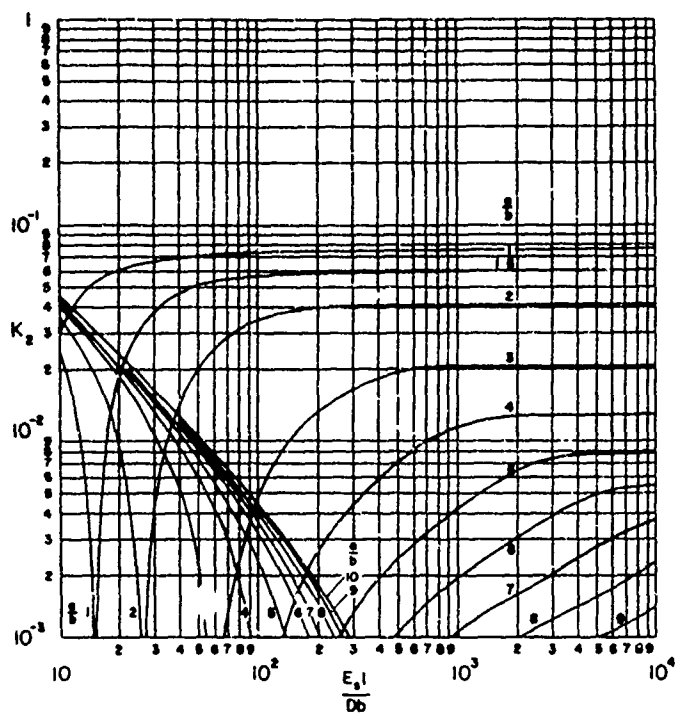
FIGURE 47 STRESS PARAMETER AT LOCATION 2 FOR \rho_s A_s / \rho_0 b t = 2
