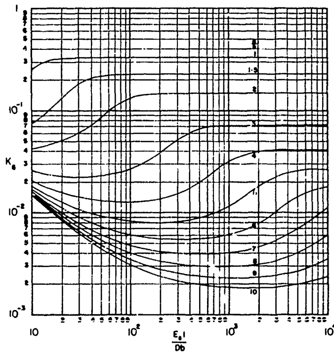
FIGURE 4.20. STRESS PARAMETER AT LOCATION 5 FOR \rho_s A_s / \rho_p b t = 3
