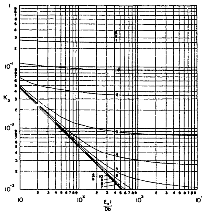
FIGURE 4.10. STRESS PARAMETER AT LOCATION 3 FOR \rho_s A_s / \rho_p bt = 1
