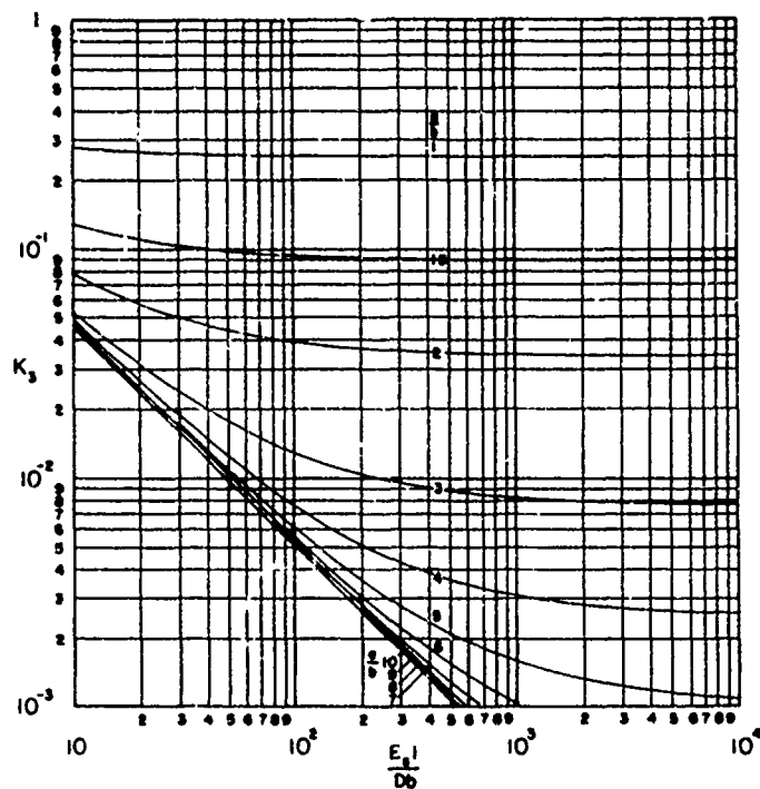
FIGURE 4.9. STRESS PARAMETER AT LOCATION 3 FOR \rho_s A_s / \rho_p bt = 0
