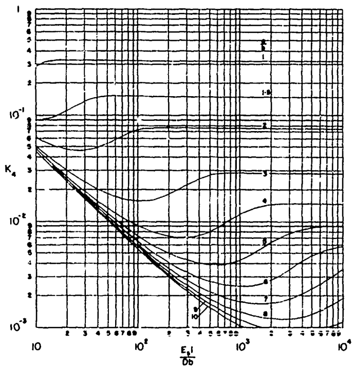
FIGURE 4.16 STRESS PARAMETER AT LOCATION 4 FOR \rho_s A_s / \rho_p b t = 3
