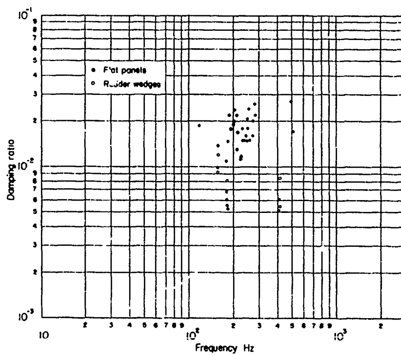
FIGURE 24 HONEYCOMB STRUCTURES
