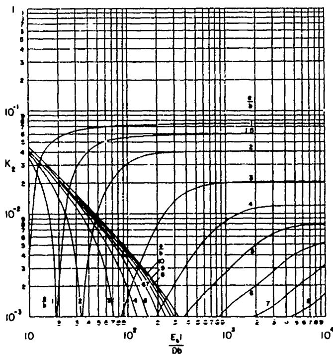
FIGURE 48 STRESS PARAMETER AT LOCATION 2 FOR \rho_s A_s / \rho_0 b t = 3
