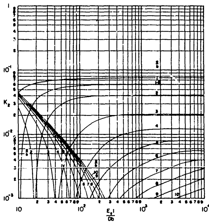
FIGURE 4.6. STRESS PARAMETER AT LOCATION 2 FOR \rho_s A_s / \rho_p b t = 0
