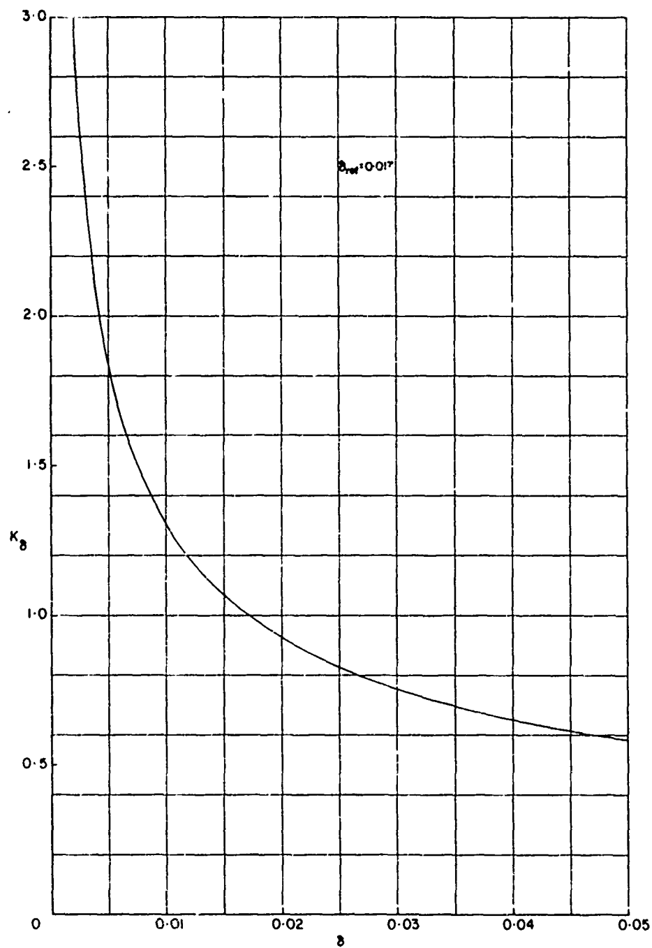
FIGURE 4.27. DAMPING RATIO CORRECTION FACTOR
