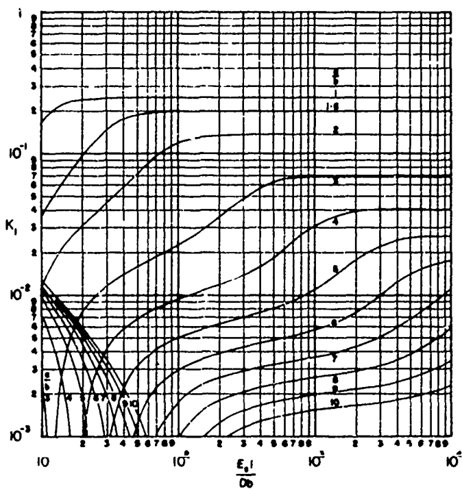
FIGURE 4.4. STRESS PARAMETER AT LOCATION 1 FOR \rho_s A_s / \rho_p b t = 3
