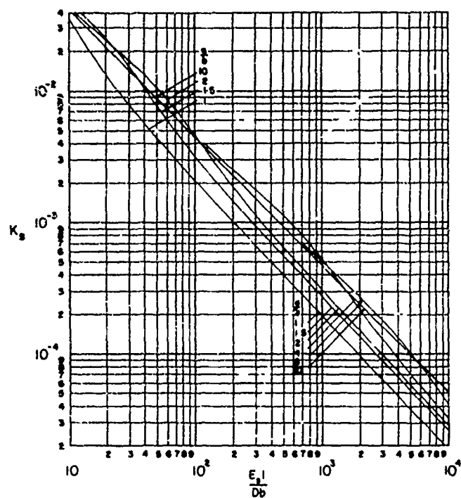
FIGURE 4.23. STRESS PARAMETER AT LOCATION S FOR \rho_s A_s / \rho_p b t = 2
