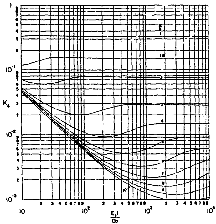
FIGURE 4.15. STRESS PARAMETER AT LOCATION 4 FOR \rho_s A_s / \rho_p b t = 2
