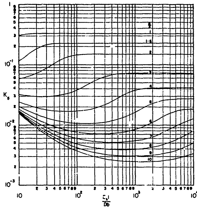
FIGURE 4.19. STRESS PARAMETER AT LOCATION 5 FOR \rho_s A_s / \rho_p b t = 2
