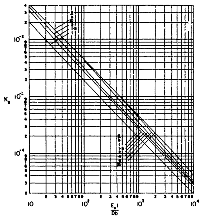
FIGURE 4.21. STRESS PARAMETER AT LOCATION S FOR \rho_s A_s / \rho_p b t = 0
