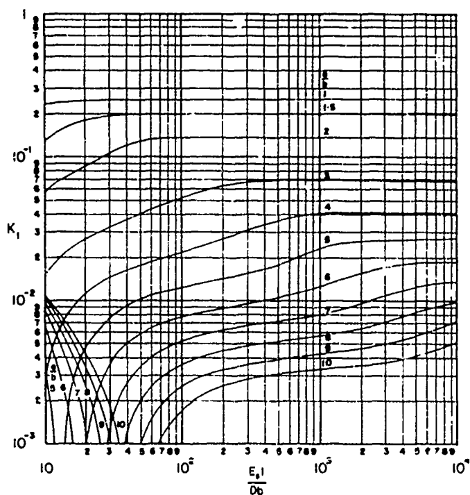
FIGURE 4.2. STRESS PARAMETER AT LOCATION I FOR \rho_s A_s / \rho_p b t = 1
