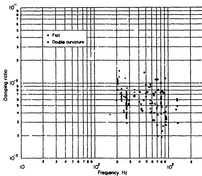
FIGURE 23. BUILT-UP STRUCTURES WITH INTEGRALLY MACHINED SKINS
