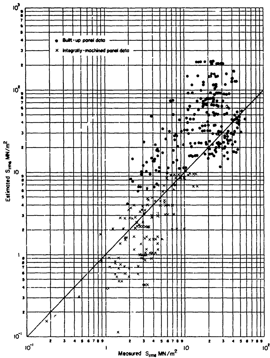
FIGURE 4.28 COMPARISON OF ESTIMATED AND MEASURED STRESS USING CALCULATED FREQUENCY AND \delta = 0.017 FOR STRESS ESTIMATION
