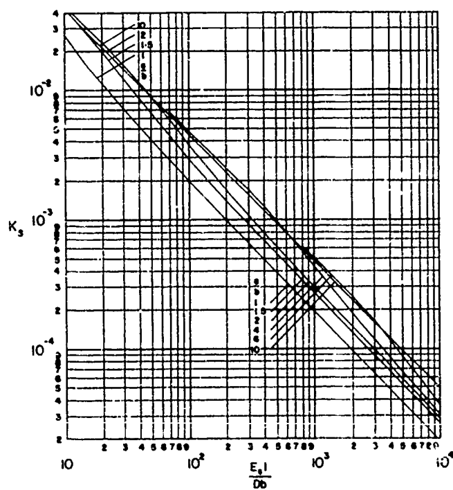
FIGURE 4.22. STRESS PARAMETER AT LOCATION S FOR \rho_s A_s / \rho_p b t = 1
