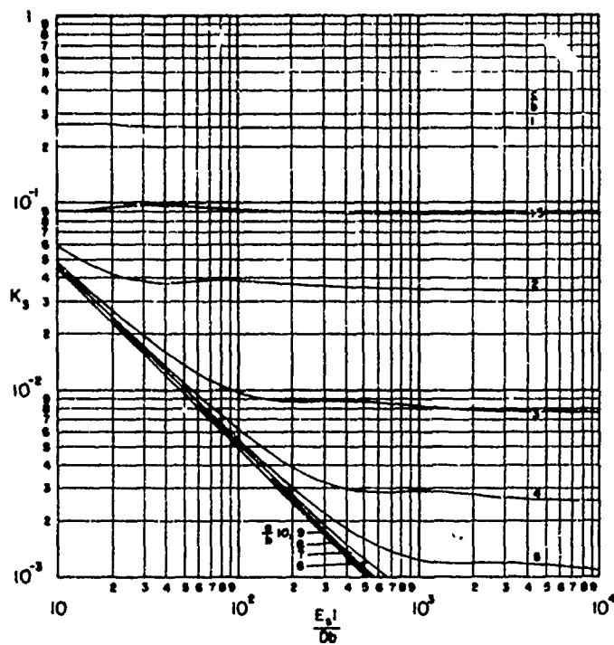
FIGURE 4.11. STRESS PARAMETER AT LOCATION 3 FOR \rho_s A_s / \rho_p b t = 2
