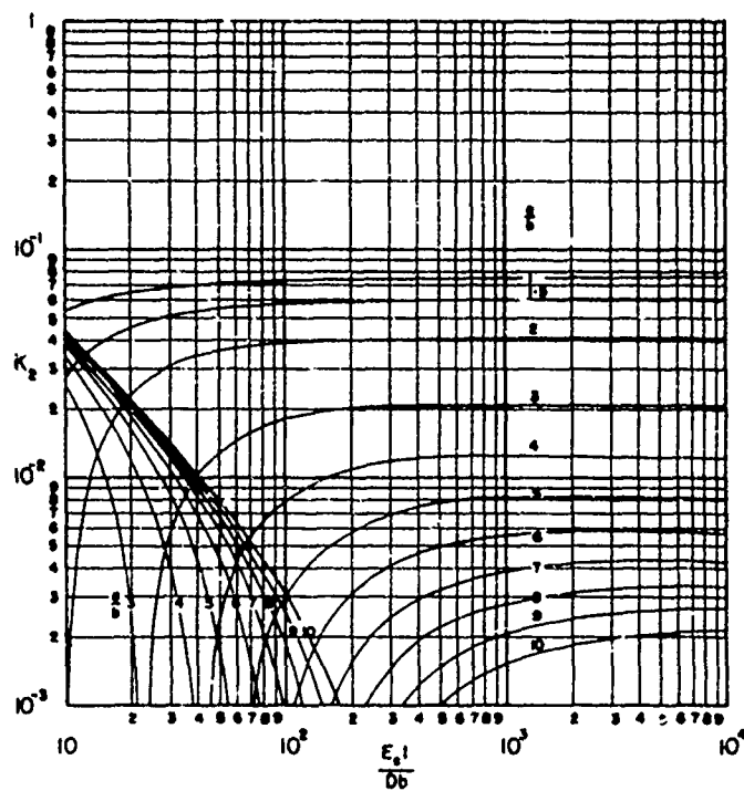
FIGURE 4.5. STRESS PARAMETER AT LOCATION 2 FOR \rho_s A_s / \rho_p b t = 0
