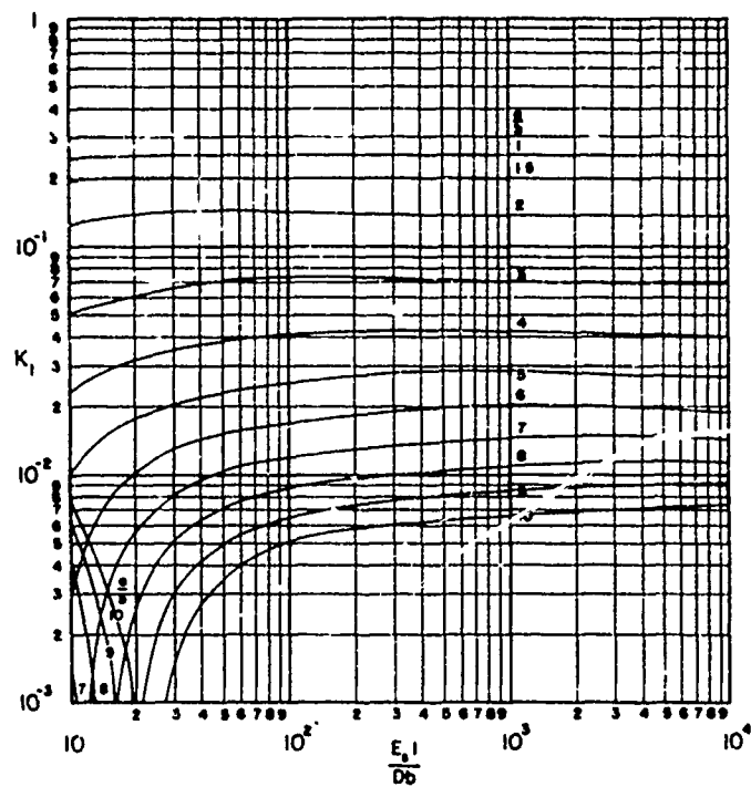
FIGURE 4.1. STRESS PARAMETER AT LOCATION I FOR \rho_s A_s / \rho_p b t = 0
