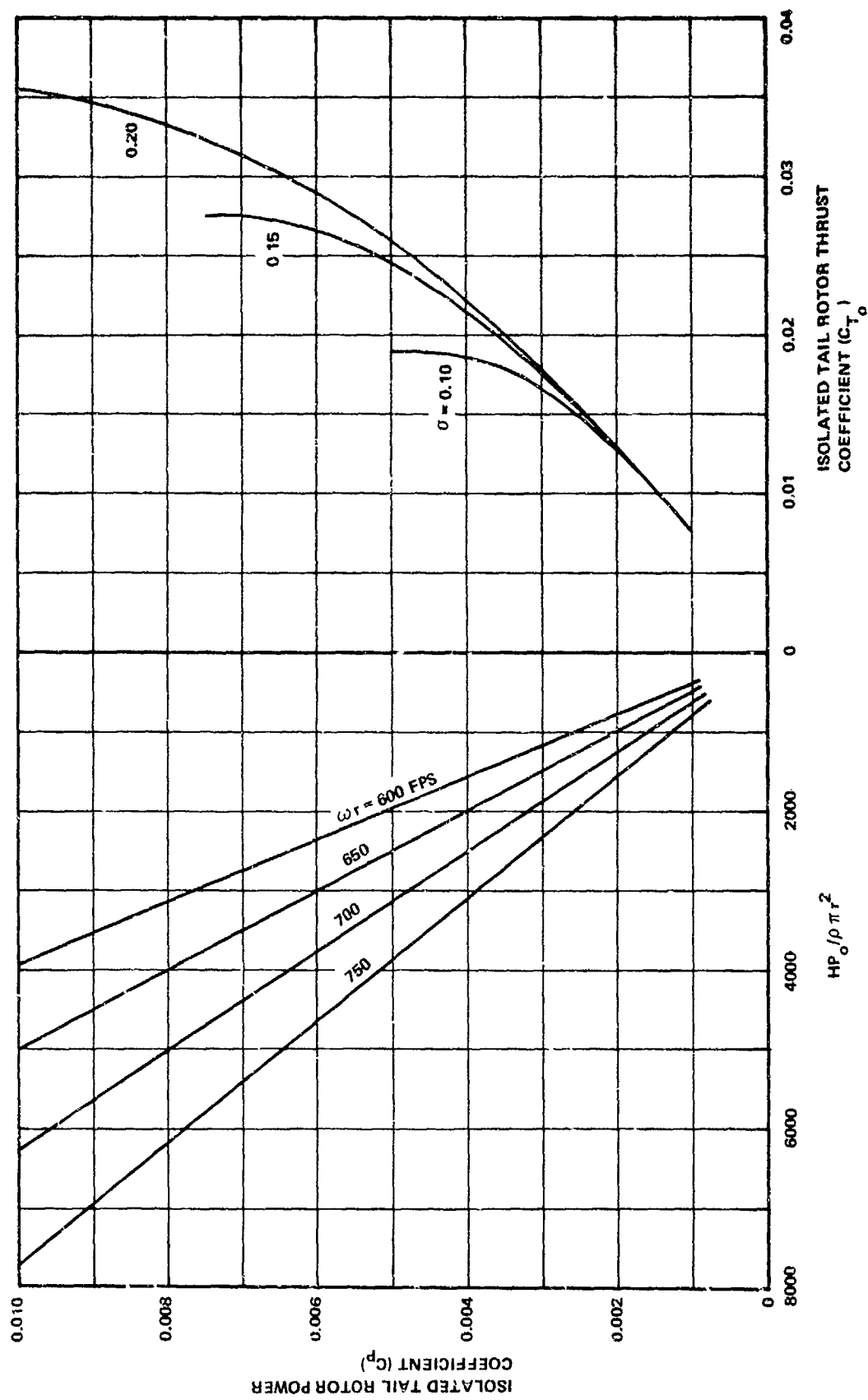
Figure 16-2. Determination of Maximum Static Thrust Horsepower at \mu = .046 , \psi = 90^\circ .
