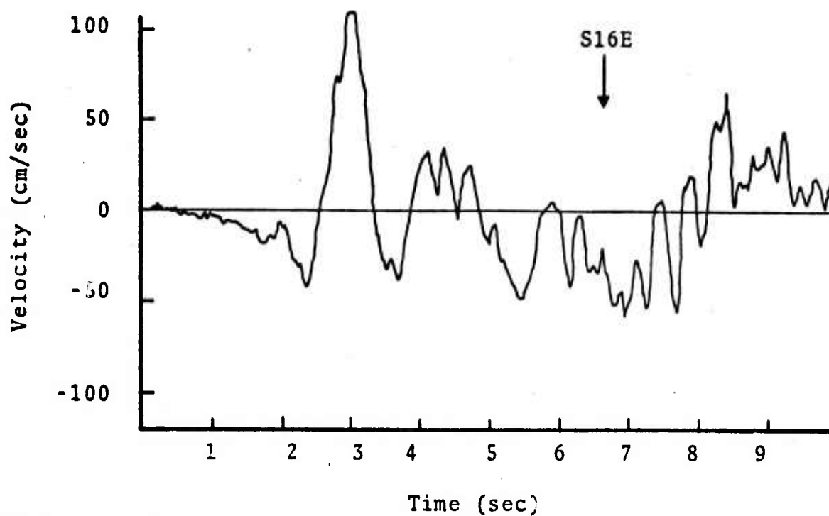
Fig. 29--Horizontal component of particle velocity at Pacoima Dam from the San Fernando Earthquake. Motion in the positive direction corresponds to ground velocity toward the epicenter.
